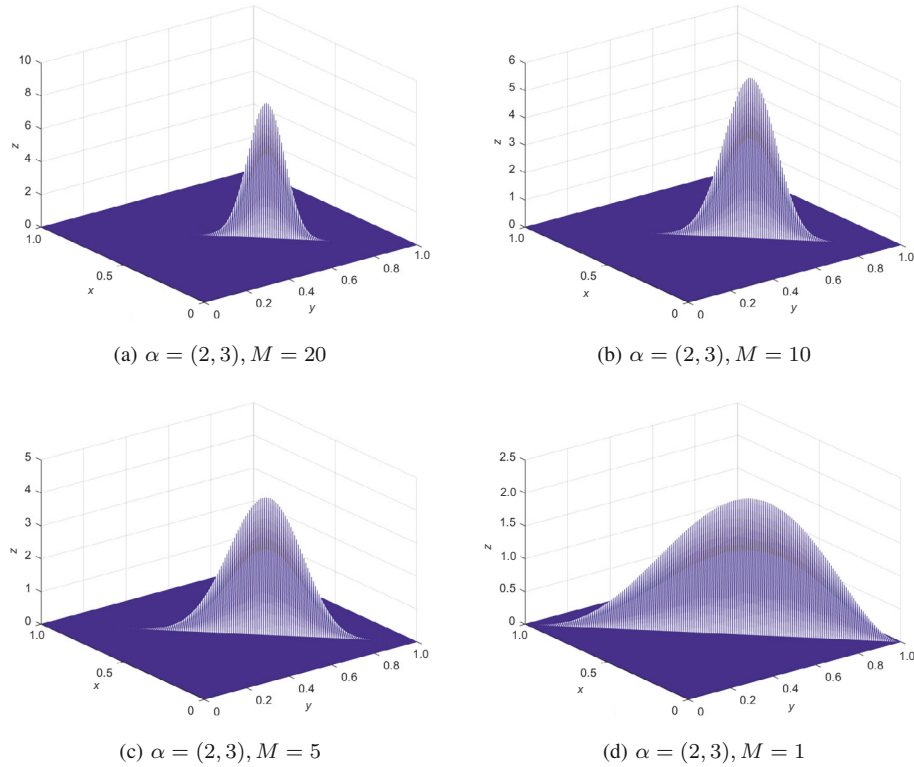
Figure 3 (Color online) The probability density function of 2-D Dirichlet distribution with different scale parameters
