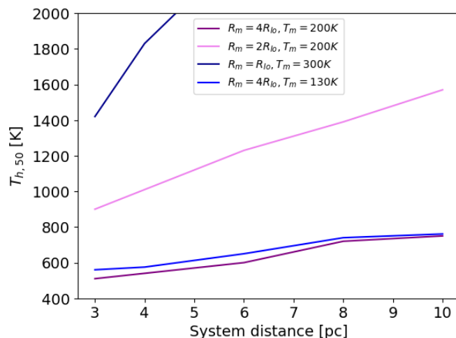
Fig. 6. T_{h,50} as a function of the system’s distance for the modeled 2.5 h variable planet with a 600 K effective temperature and different moon properties (orbital period = 27 h). For moon sizes between 2-4 R_{Io} , a moon can be detected even for moderate T_h and T_m in 140 h observations. For very nearby systems, an exo-Io ( R_m = R_{Io} ) can be detected for high T_h ( >1400\text{K} )
