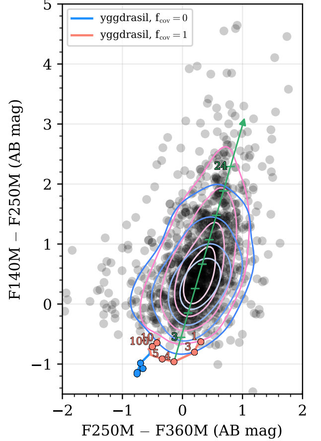
Figure 4. A color-color plot of the clusters (black dots). The contours show the density of the points; contour levels show 10, 25, 50, and 75% density levels for clusters which overlap with the Mayya et al. (2008) catalog (blue) and those only detected with NIRCам (pink). The colored tracks show YGGDRASIL SSP models assuming no ( f_{\text{cov}} = 0 ; blue) and maximal ( f_{\text{cov}} = 1 ; red) contributions from nebular emission. The green arrow shows the slope of the reddening vector with A_V = 3 - 24 mag marked in increments of 3. The clusters in M 82 detected with NIRCам show significant reddening with respect to the dust-free SSP tracks.
