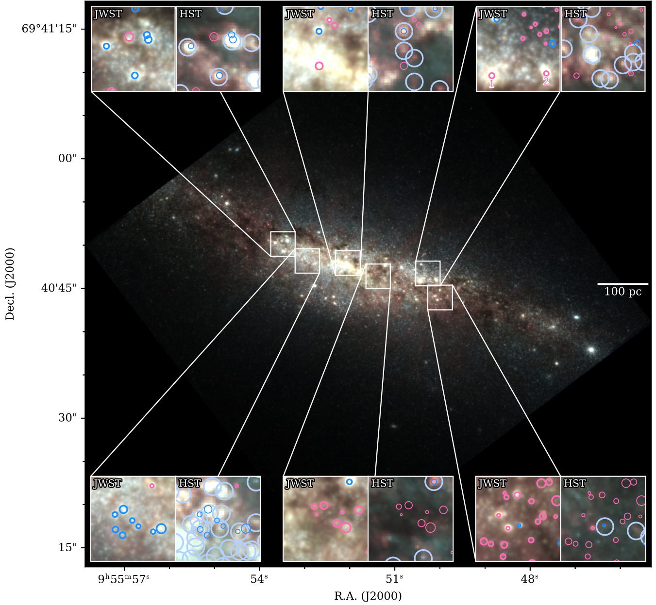
Figure 1. The central 870 pc of M 82 seen with NIRCам showing F140M (blue), F250M (green), and F360M (red) on an asinh scale. Insets show zoom-ins to 50 pc \times 50 pc regions around some representative massive star cluster candidates. The circles indicate the massive clusters identified in the NIRCам image, where the radius of the circle is the fitted (deconvolved) radius (see Section 3 and Table 1). Blue (pink) circles show clusters which do (do not) overlap with the HST catalog (Mayya et al. 2008, see Section 4.1). Clusters 1 and 2 are labeled (see Sections 3.2 and 4.1). The right insets show HST three-color images at the same locations (blue: F435W, green: F555W, red: F814W). The light blue circles in the HST insets show the star clusters identified by Mayya et al. (2008) in these selected regions using the same HST data, where the radius of each circle is 5 pc. The pink and blue circles are the same as in the left panels.
