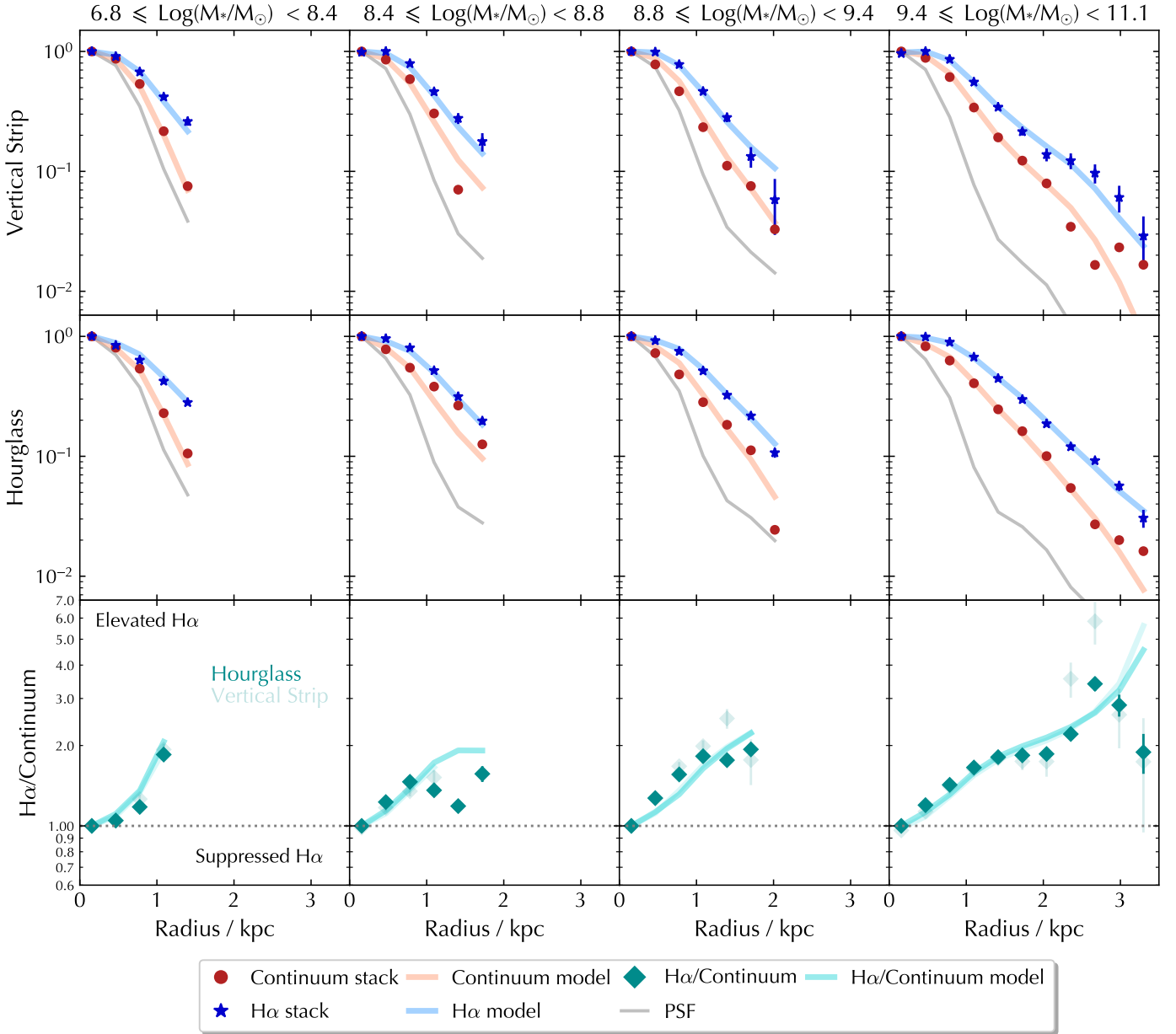
Fig. 3. Peak-normalised surface brightness profiles of the FRESCO stellar continuum and H \alpha stacks along with their PSF-convolved best-fit GALFIT models and PSFs accounting for pixels only within the vertical strip along the centre of the thumbnail (top row) or within the hourglass mask (middle row). Bottom row: Peak-normalised H \alpha equivalent width ( [H\alpha/C] ) profiles for both the stacks and PSF-convolved best-fit GALFIT models. [H\alpha/C] \geq 1 and increases with increasing galactocentric radius, suggesting the inside-out growth via star formation of star-forming galaxies as early as z \sim 5.3 .
