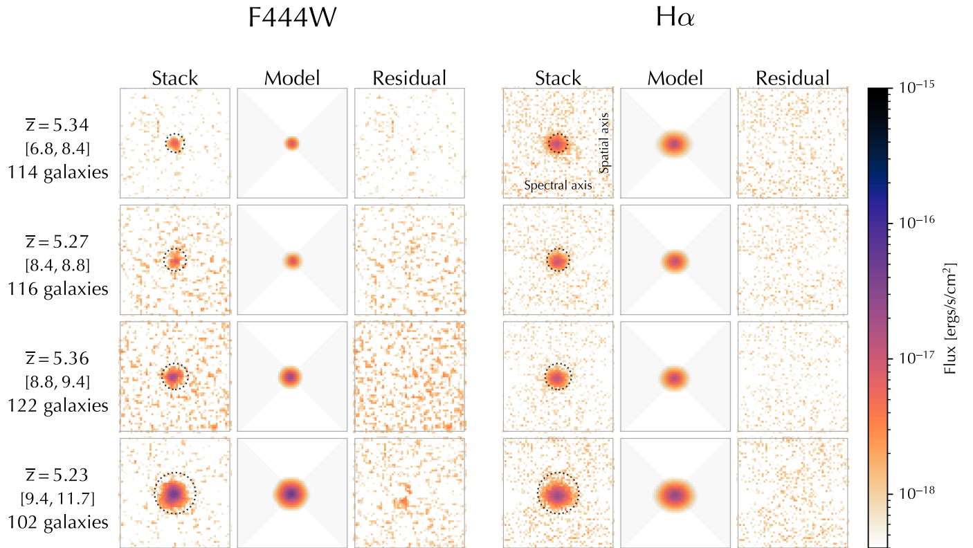
Fig. 2. F444W and H\alpha stacks with their associated GALFIT fits. Models are PSF-convolved single-component Sérsic profiles (see Section 3.2 for more details). Residuals after the model was subtracted from the data are shown in the last column for both F444W and H\alpha . Each thumbnail is 60 \times 60 pixels, where 1 \text{ pixel} = 0.05'' . \bar{z} is the median grism redshift of each stack, below which the \text{Log}(M_*/M_\odot) range of each stack is shown in square brackets. The colour map is logarithmic, with H\alpha stacks and fits multiplied by 100 for visibility. The shaded grey regions show pixels that were ignored by the hourglass mask (see Section 3), and the dotted black circles show the region within which surface brightness profiles were measured (see Section 4).
