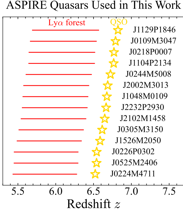
Figure 1. The redshift distribution (yellow) of ASPIRE quasars used in this work, in the ascending order of redshift, and the redshift range of the Ly \alpha forest used in the analysis is denoted by the red horizontal line. We exclude the Ly \alpha forest spectrum at > 1176 \text{ \AA} rest frame to exclude the possible emission from the quasar proximity zone and exclude the rest \lambda < 1040 \text{ \AA} Ly \alpha forest to exclude the contamination from O VI \lambda 1033 emission and the Ly \beta forest. The redshift range of ASPIRE quasars used in this work is from z \sim 6.5 to z \sim 6.8 and the corresponding Ly \alpha absorption redshift range is from z \sim 5.4 up to z \sim 6.6 .
