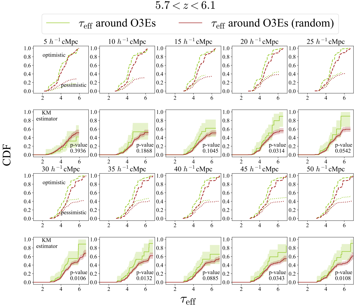
Figure 10. Similar to Figure 9, but for [O III] emitters at 5.7 < z < 6.1 .
