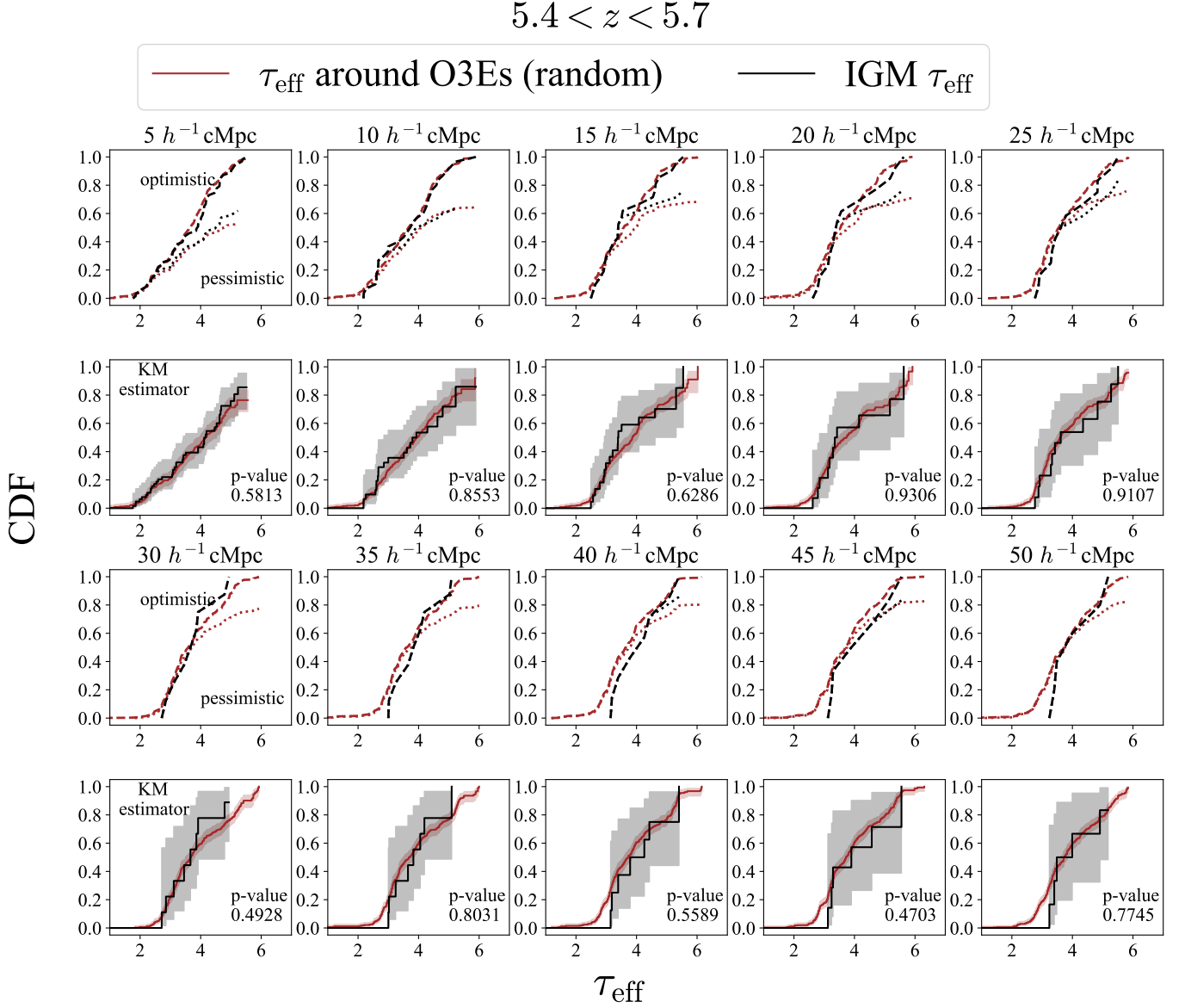
Figure 19. The cumulative distribution function of the random \tau_{\text{eff},[\text{OIII}]} (brown) and \tau_{\text{eff}} of IGM patches (black) at 5.4 < z < 5.7 .
