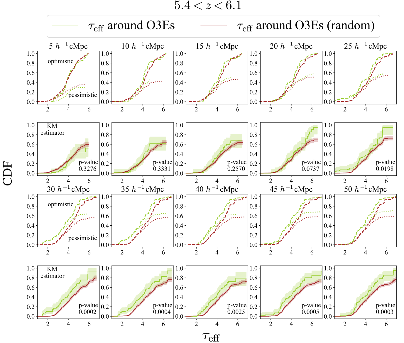
Figure 9. The first and the third rows show the cumulative distribution functions of the \tau_{\text{eff}} around [O III] emitters at 5.4 < z < 6.1 (yellowgreen), adopting influence radii from 5 h^{-1} \text{ cMpc} to 50 h^{-1} \text{ cMpc} . The random cumulative distribution function of the \tau_{\text{eff}} around [O III] emitters is shown in brown, representing the \tau_{\text{eff}} distribution of IGM patches. The “optimistic” and the “pessimistic” CDFs are plotted in dashed and dotted lines, respectively. The second and the fourth rows show the fitted CDFs from Kaplan-Meier (KM) estimator and 1\sigma confidence interval of the CDF is shown in the shaded regions of the corresponding color. The null-hypothesis p-value from the log-rank test is shown in the bottom right corner of each sub-panel. See text for more details.
