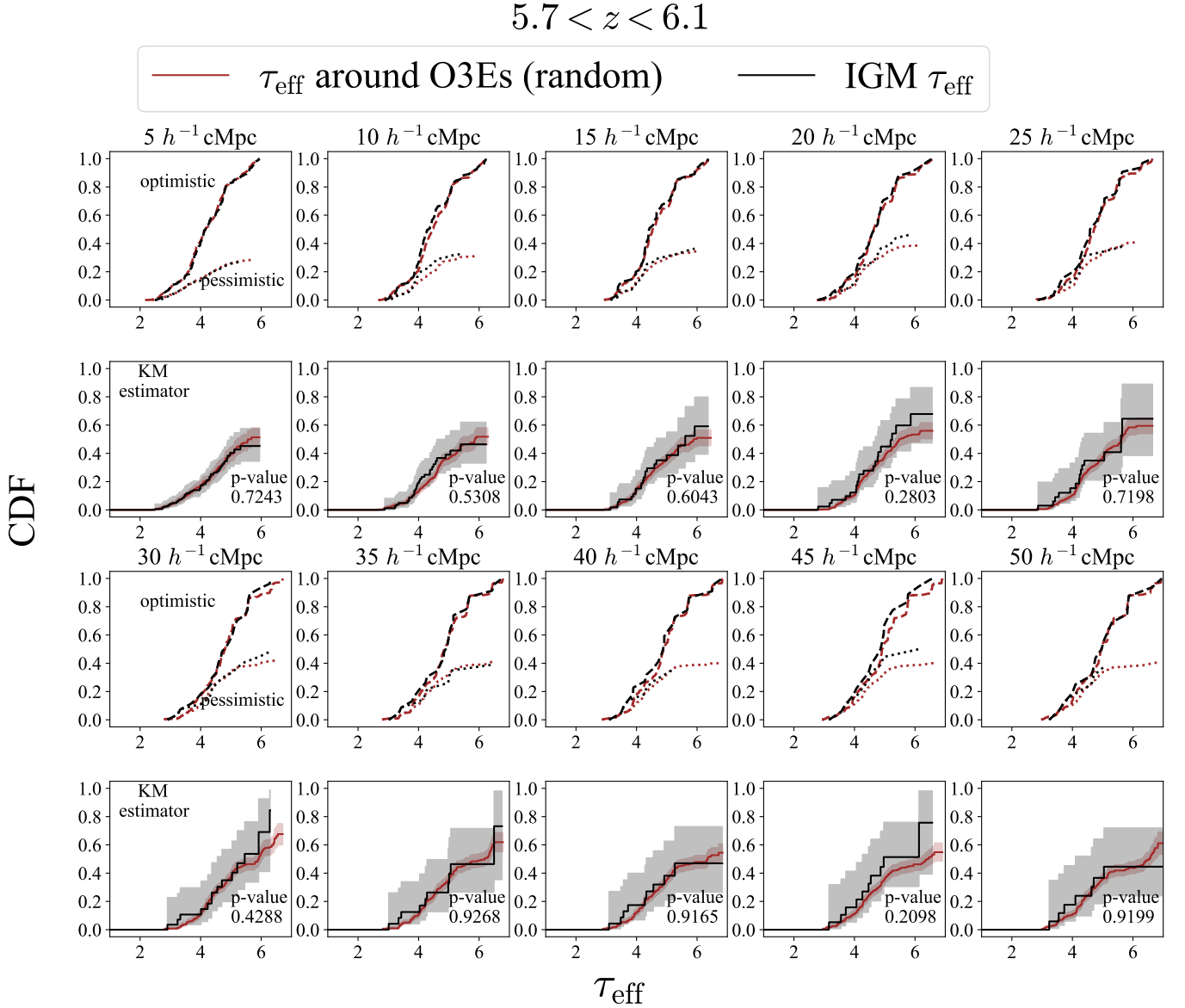
Figure 18. The cumulative distribution function of the random \tau_{\text{eff},[\text{OIII}]} (brown) and \tau_{\text{eff}} of IGM patches (black) at 5.7 < z < 6.1 .
