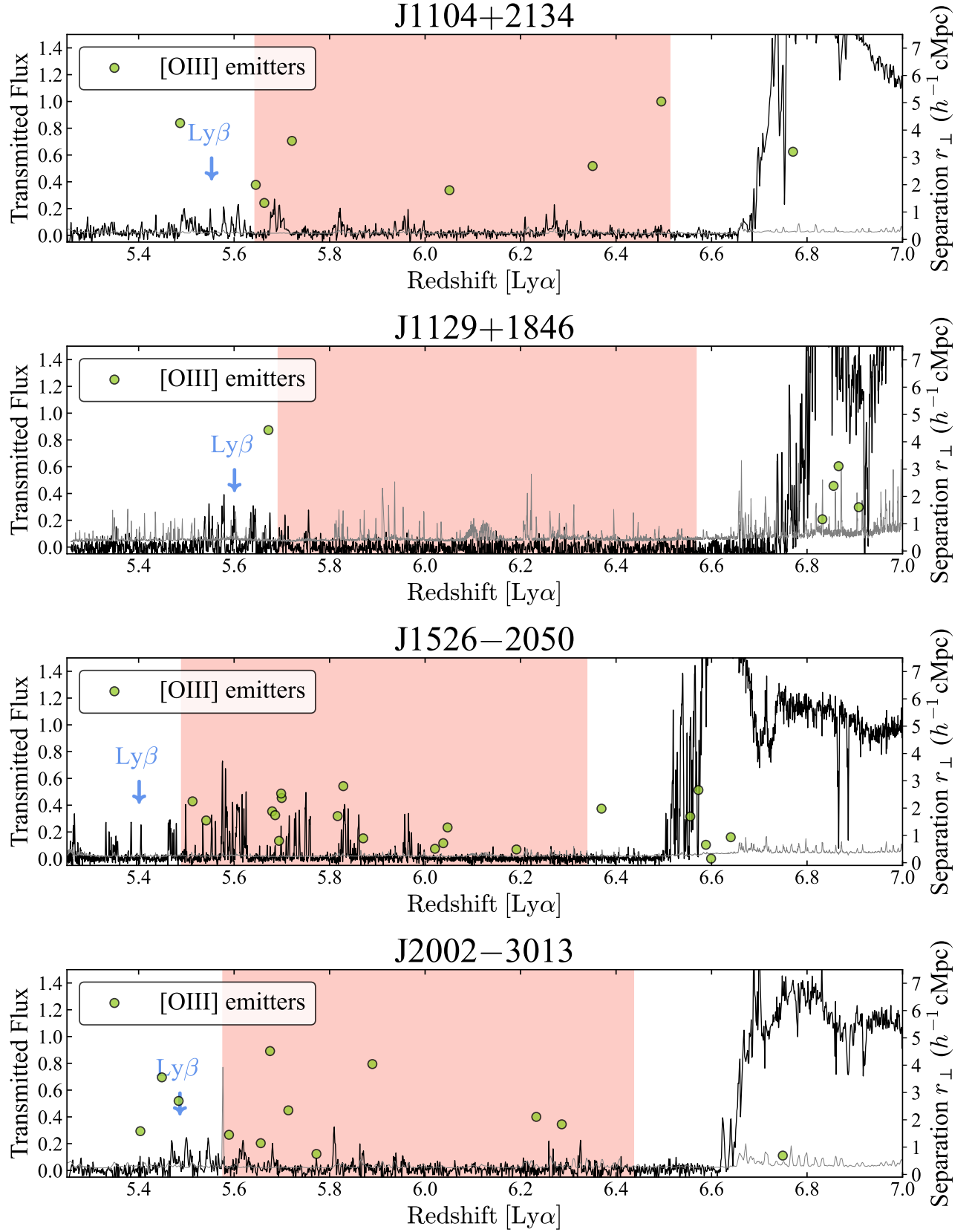
Figure 15. (continued.) The line of sight plot of ASPIRE quasars J1104+2134, J1129+1846, J1526–2050, and J2002–3013, together with [\text{O III}] emitters detected in the quasar fields.
