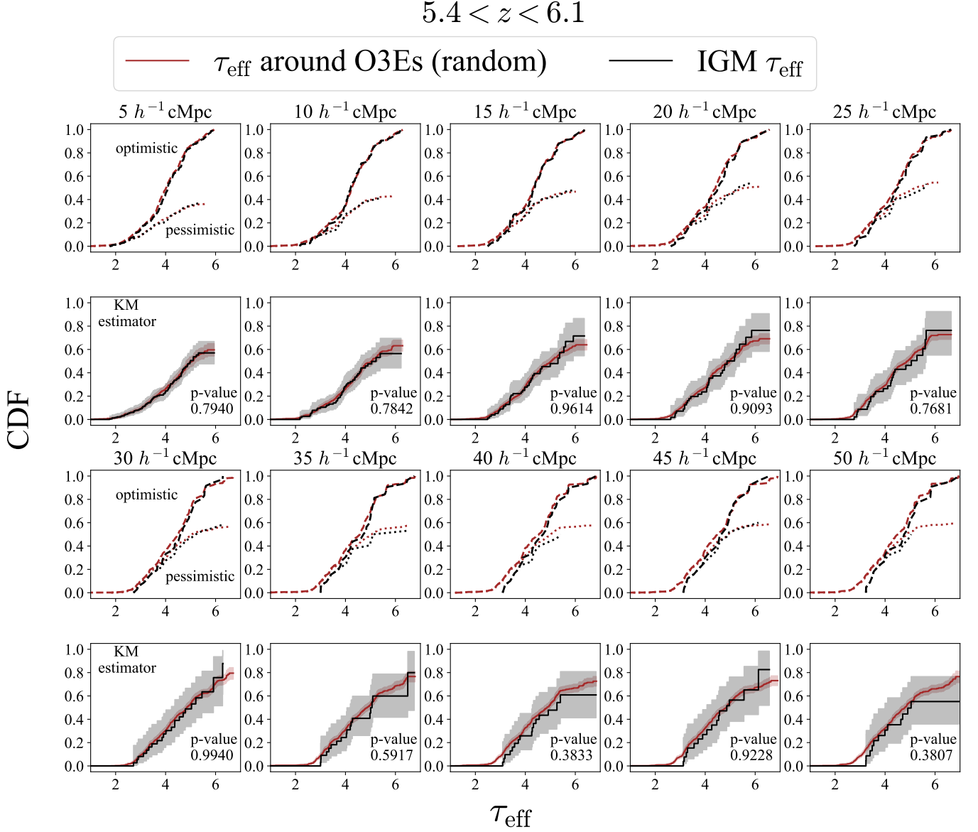
Figure 17. The first and the third rows show the cumulative distribution functions of the random \tau_{\text{eff}} around [O III] emitters (brown), and \tau_{\text{eff}} of IGM patches (black) at 5.4 < z < 6.1 . The influence radius is from 5 h^{-1} \text{cMpc} to 50 h^{-1} \text{cMpc} for \tau_{\text{eff}, [\text{O III}]} measurements and \tau_{\text{eff}} are measured using the bin size of twice the corresponding influence radius. The “optimistic” and the “pessimistic” CDFs are plotted in dashed and dotted lines, respectively. The second and the fourth row show the fitted CDFs from Kaplan-Meier (KM) estimator and 1\sigma confidence interval of the CDF is shown in the shaded regions of the corresponding color. The null-hypothesis p-value from the log-rank test is shown in the bottom right corner of each sub-panel. With all influence radii, the random \tau_{\text{eff}, [\text{O III}]} distribution is consistent with \tau_{\text{eff}} distribution of IGM patches.
