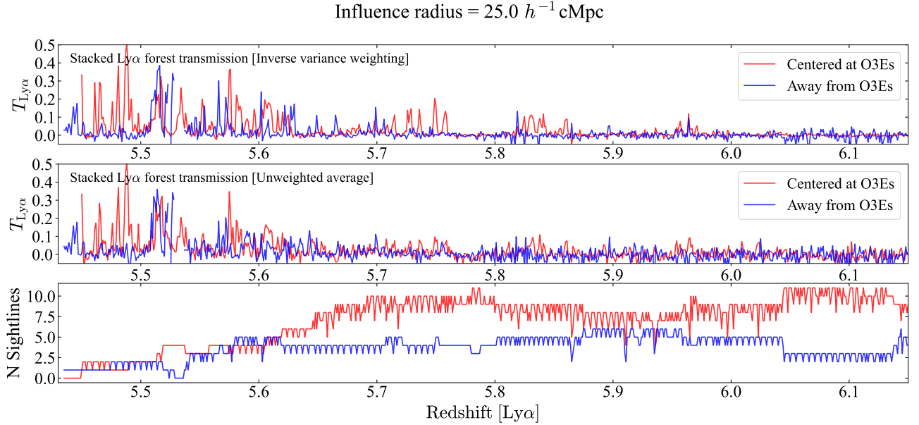
Figure 6. Top - The stacked transmission of the \text{Ly}\alpha forest around [O III] emitters (red) and away from [O III] emitters (blue), adopting the inverse variance weighting and an influence radius of 25 h^{-1} \text{ cMpc} , see text for details. Middle - The stacked transmission of the \text{Ly}\alpha forest around [O III] emitters (red) and away from [O III] emitters (blue), where the stacked transmission is the unweighted average transmission. Bottom - The number of quasar line of sights (LOSs) available in each pixel of the stacked \text{Ly}\alpha forest transmission around [O III] emitters (red) and the stacked \text{Ly}\alpha forest transmission away from [O III] emitters (blue).
