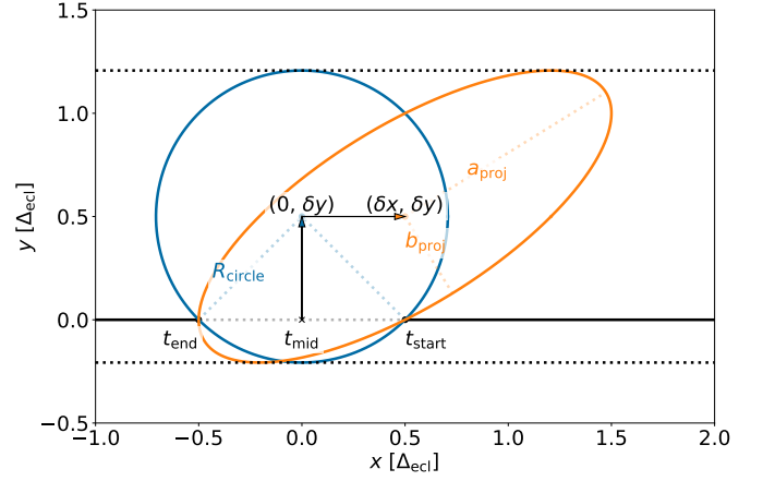
Fig. 2. Determining the simplest sheared disc model. The coordinate system is centred at (0,0). The midpoint of the disc is shifted up to (0, \delta y ). A circle (blue) is drawn with radius R_{\text{circle}} (Equation 3). The midpoint of the disc is shifted to ( \delta x , \delta y ), shearing the circle into an ellipse (orange, Equation 4, 5 and 6). From this ellipse the disc parameters can be determined.
