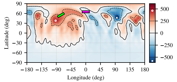
Figure 1. Surface magnetic field structure of AB Dor, derived from spectropolarimetric observations performed in December 2002 ( Hussain et al. 2007 ). Two rectangular patches display the two different flux rope locations for the simulated CME models: the green patch is located at open magnetic field region, while the magenta patch at closed-field region. The white circle and cross indicate the maximum and minimum magnetic field strengths. The average strength of the depicted radial field is 105 G.
