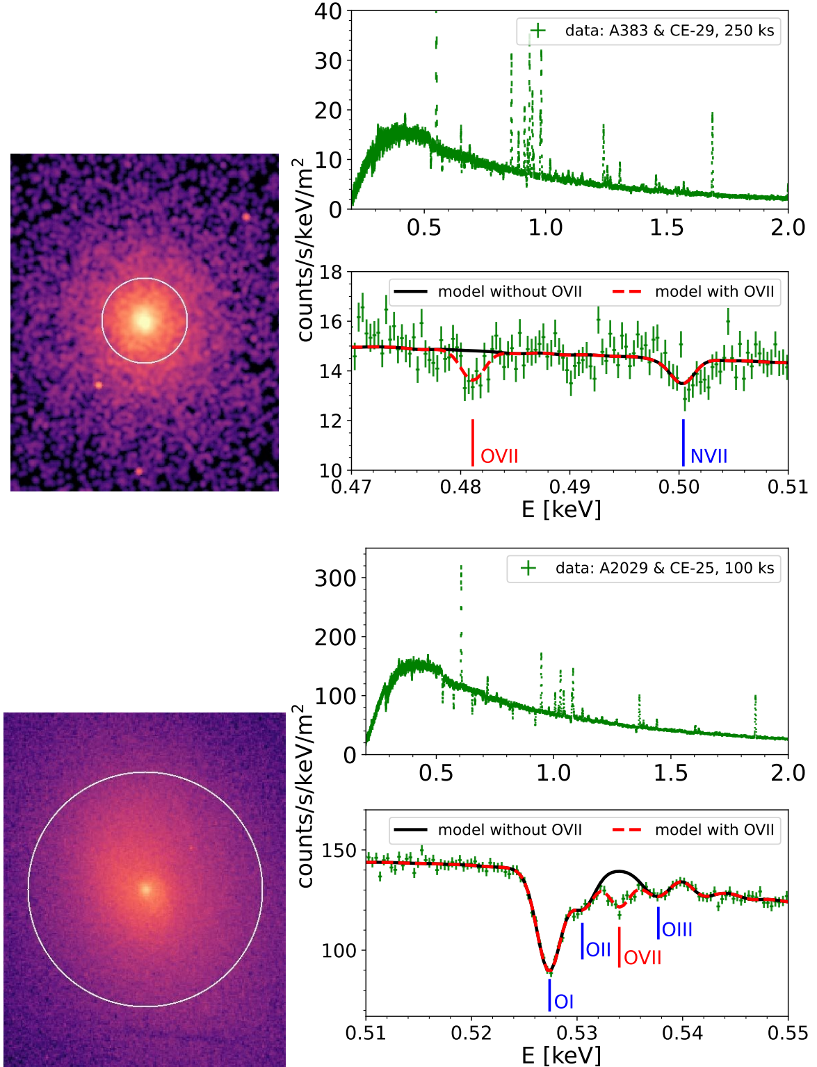
Figure 6. Broad band simulated spectrum for Athena X-IFU in the energy range 0.2 – 2 keV and a zoom-in to 0.47 – 0.51 keV of the CE-29 z + Hydrangea absorber and A383 (top two right panels, 250 ks exposure time, z = 0.1883 ) and the CE-25 and A2029 (bottom two right panels, 100 ks exposure time, z = 0.0779 ), where the zoom-in for CE-25 and A2029 shows the energy band 0.51 – 0.55 keV. The black solid line represents the spectral model (folded through the response of X-IFU) together with the three-component absorption model of the Milky Way ISM as described in Sec. 3.1.3. The absorption lines of the local ISM are indicated in all panels with blue vertical lines. The red dashed line represents the same spectral model as the black solid line but with an addition of the Hydrangea O VII absorption line (solid red vertical lines) according to the best-fitting parameters described in Table 2. Left panels show the Chandra images of A383 (top left panel) and A2029 (bottom left panel). The white circle has a radius of 100 kpc as used in all calculations in this paper. The errors shown in the spectra represent the standard deviation 1\sigma .
