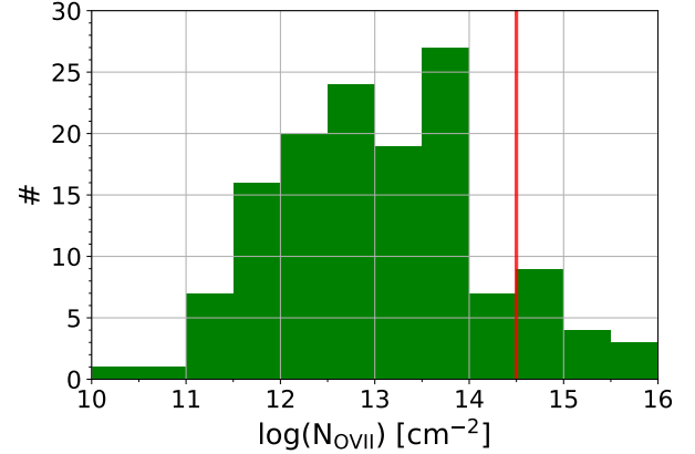
Figure 1. Histogram of the number of sightlines (out of the total number of 138 through Hydrangea cluster centres) as a function of O VII total column density per line of sight. The width of the column density bins is 0.5 dex. The red solid line represents the cut for all LoSs with O VII total column density higher than 10^{14.5} \text{ cm}^{-2} . This cut selects 16 directions of lines of sight that are later discussed in the paper.
