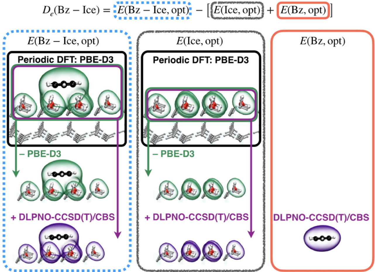
Figure 1. Representation of the ONIOM approach used to compute the adsorption energy of benzene on an ice surface model. Each component of the energy expression at the top is decomposed into up to three calculations: two periodic DFT calculations (full system and model) and one DLPNO-CCSD(T) calculation (model). The full system optimized at the PBE-D3/MOLOPT-TZV2P is shown at the top of each panel. Note that the benzene component is simply computed directly at the DLPNO-CCSD(T)/CBS level using an optimized PBE-D3/MOLOPT-TZV2P geometry. PBE-D3 calculations are indicated using a green colour and the DLPNO-CCSD(T) calculations using a purple colour.
