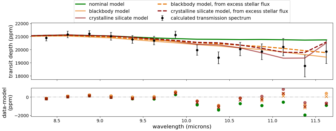
Figure 3. (top) WASP-39b MIRI observed transmission spectrum along with its model retrieval and the model retrievals adjusted by the dilution factor induced by our best debris disk models. (bottom) The residuals between the data and the models. The inclusion of the debris disk decreases the residuals.
