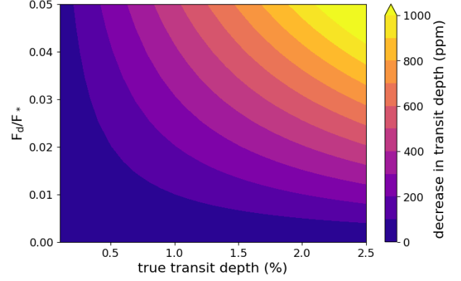
Figure 4. The decrease in transit depth due to a relatively faint debris disks can be on the order of several hundred ppm.
