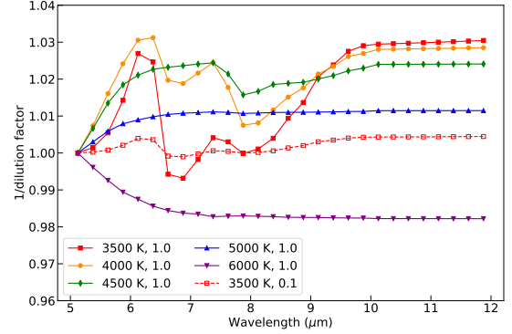
Figure 5. Dilution factor on the MIRI transit spectrum for a hypothetical stellar blend with various temperatures. The labels in the legend indicate the effective temperature and flux fraction from the blended star (1.0 is the maximum possible fraction).
