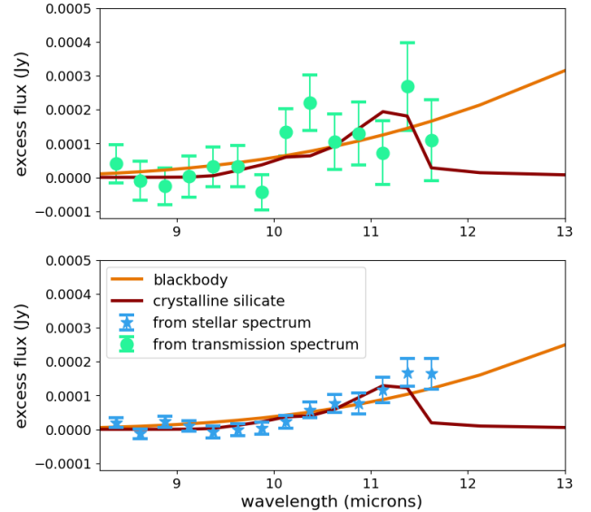
Figure 2. The best fits to the excess flux as calculated from the transmission spectrum (top) or from the stellar spectrum (bottom). We fit a crystalline silicate feature and a blackbody curve to both spectra separately. These plots assume the 3\sigma upper-limit to the WISE/W4 flux.
