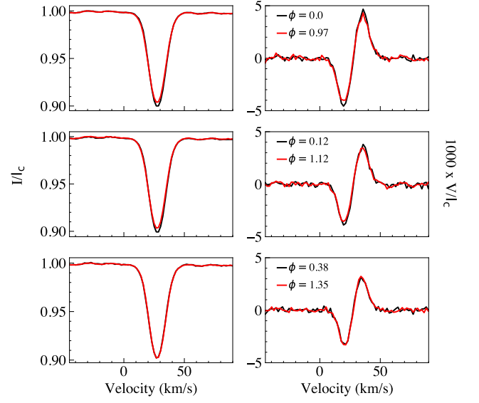
Figure 2. Stokes I (left column) and Stokes V (right column) profiles of the most recent spectropolarimetric measurements of HD 54879 (red) compared to archival data of the star at approximately the same rotation phase \phi (black), but one cycle previous to the new data. The profiles are consistent with each other.
