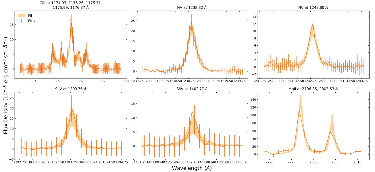
Fig. 3. Sample of measured UV lines with fitted Voigt models for LTT 1445A. The sample covers UV lines from all three COS gratings used (G130M, G160M, and G230L). Lines that are blended, e.g., C III and Mg II, were fit with combined Voigt models, whereas well-separated lines, e.g., N V and Si IV, were fit with individual models. Voigt models are made with pyspeckit (Ginsburg et al. 2022) and we explore the model parameter space with dynesty (Speagle 2020).
