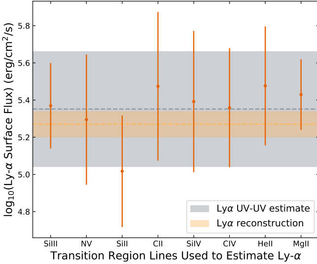
Fig. 7. Deriving the Ly \alpha flux of LTT 1445A using a reconstruction from the wings of the Ly \alpha profile observed with the STIS/G140M grating (orange 1 \sigma band; Youngblood et al. 2016) and using UV-UV line correlations with other measured UV lines with the COS instrument (orange points with 1 \sigma errors, and the average 1 \sigma gray band; Youngblood et al. 2017; Diamond-Lowe et al. 2021, 2022). In the case of LTT 1445A, we find that individual transition region lines agree with each other, and with the reconstructed value.
