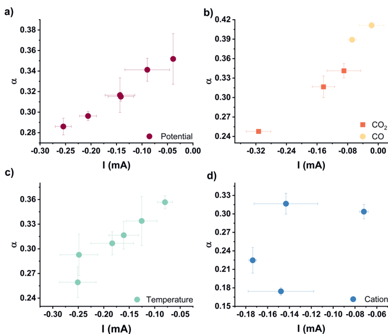
Figure D.16 chain growth probability \alpha plotted vs the activity at different conditions: a) at different potentials (data from figure 3) b) at different anions and with CO or CO 2 as reactant (data from Figure 5) c) at different temperature (data from Figure 1) d) with different cations (data from Figure 4)
