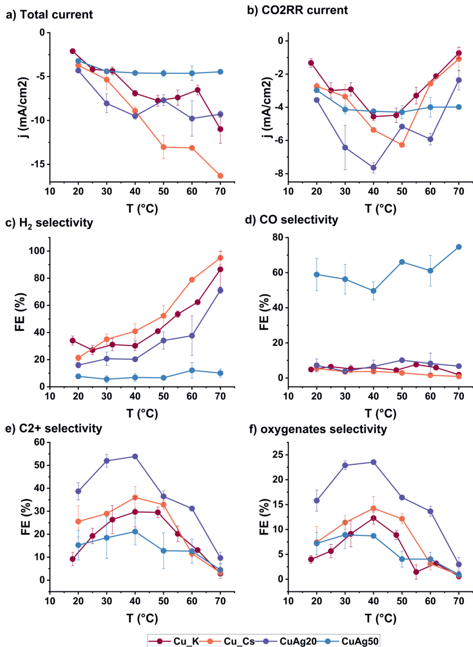
Figure 4.5 a) Total current density and b) current density towards CO 2 RR and faradaic efficiency for c) hydrogen d) CO e) C 2 + products f) oxygenates for Cu, CuAg20 and CuAg50 at -1.1V vs RHE in 0.1 M CsHCO 3 and also in 0.1 M KHCO 3 for Cu. 14
