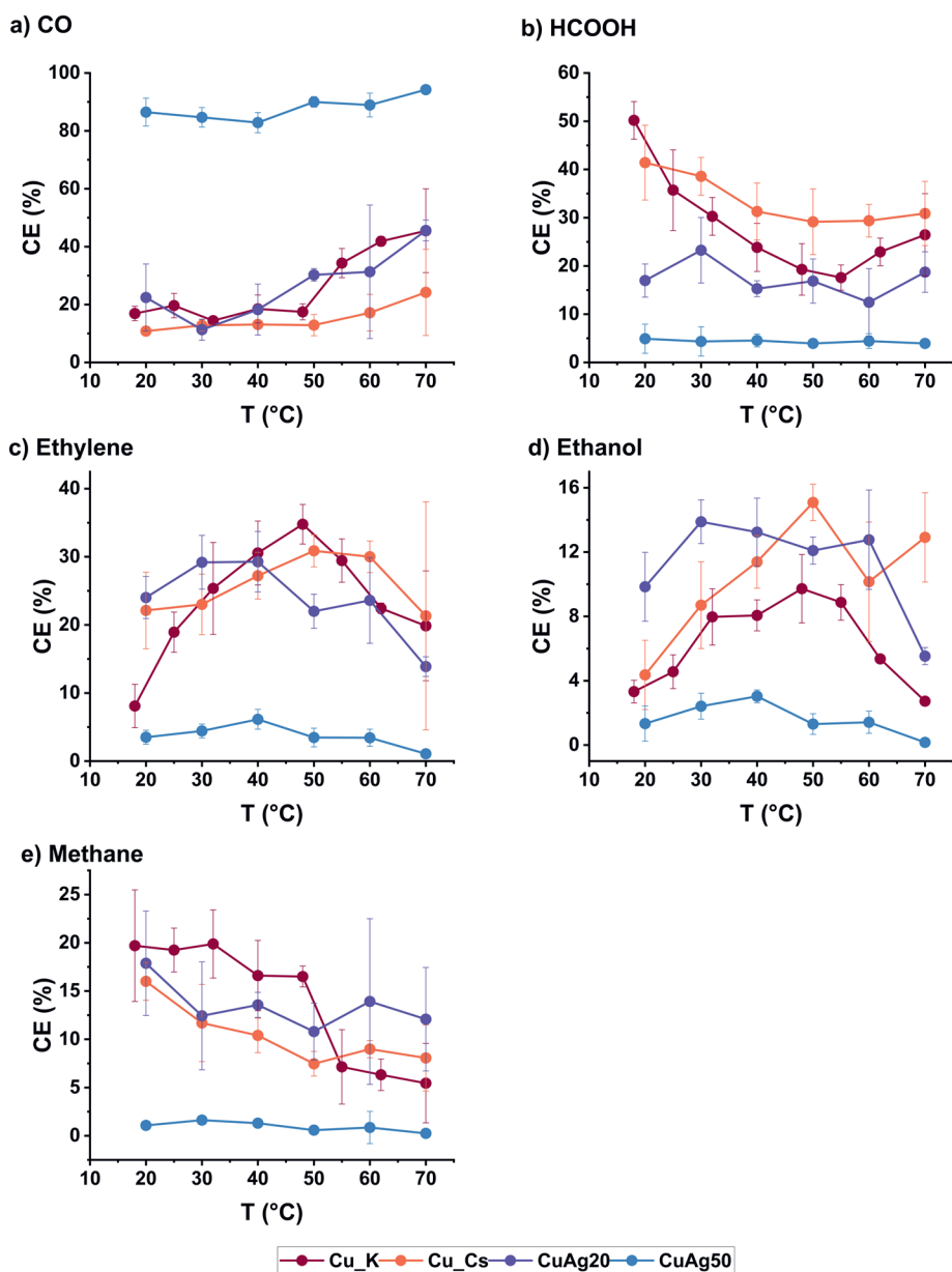
Figure C.16 Comparison of the Carbon efficiency for a) CO b) HCOOH c) ethylene d) ethanol e) methane for Cu, CuAg20 and CuAg50 at -1.1V vs RHE in 0.1 M CsHCO 3 and also in 0.1 M KHCO 3 for Cu.
