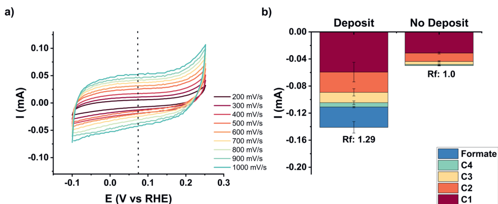
Figure D.4 a) Determination of the double layer capacitance by cyclic voltammetry. The double layer capacitance was determined at 0.075 V vs RHE and used to calculate a roughness factor (Rf). b) the roughness factor was used to normalize the deposited layer to the non-deposited catalyst, showing that the enhancement is not due to a roughness effect.
