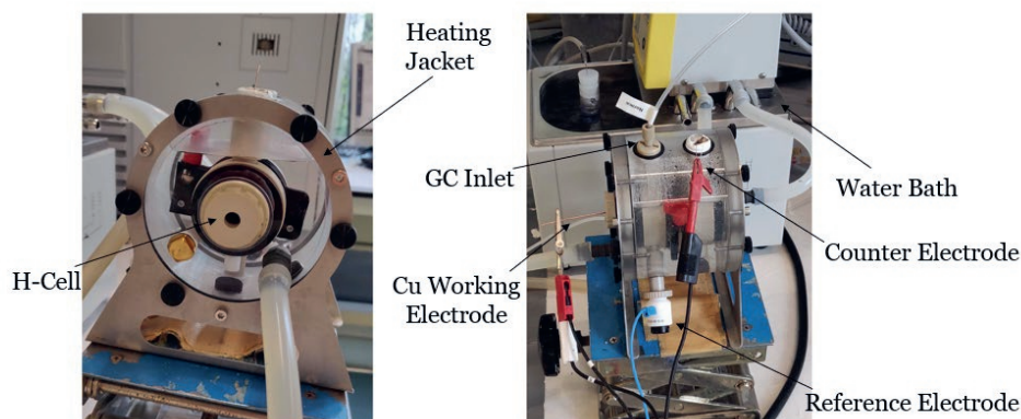
Figure C.1 Photos from the H-cell surrounded by the water jacket used to control the temperature
