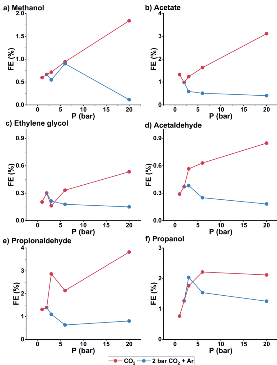
Figure F.13 Faradaic efficiency towards the minor CO 2 RR products as function of CO 2 and total pressure at -1.5 V vs SHE in 0.2 M KHCO 3 at 25 °C. Red lines are performed in pure CO 2 and blue lines are at 2 bar of CO 2 and pressure is increased with Ar. FE for a) methanol b) acetate c) ethylene glycol d) acetaldehyde e) propionaldehyde and f) 1-propanol
