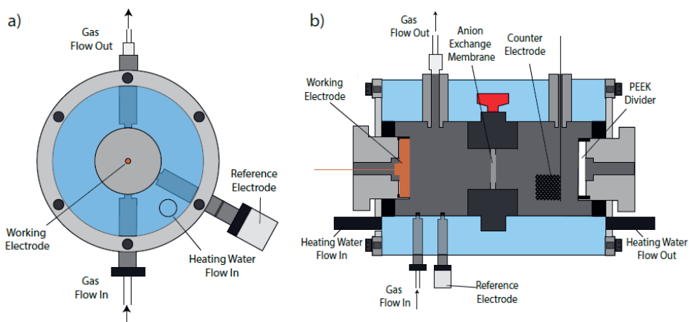
Figure C.2 Schematics of the H-cell surrounded by the water jacket used to control the temperature. a) Frontal-section of the cathodic chamber and (b) cross-section of the electrochemical H-cell with heating jacket
