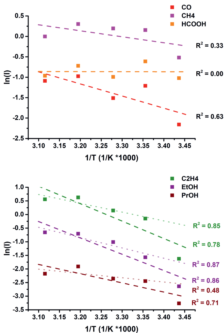
Figure B.20 Arrhenius plots of a) CO, methane, formic acid production and b) ethylene, ethanol and 1-propanol during CO 2 RR at -1.1 V vs. RHE in -0.1M KHCO 3 . The striped lines gives the trendline with the corresponding R^2 value to illustrate the linearity of the trendline. The light dotted lines for the C 2 + products are the trendlines without the point at 18 °C. It can be seen that the slope changes significantly.
