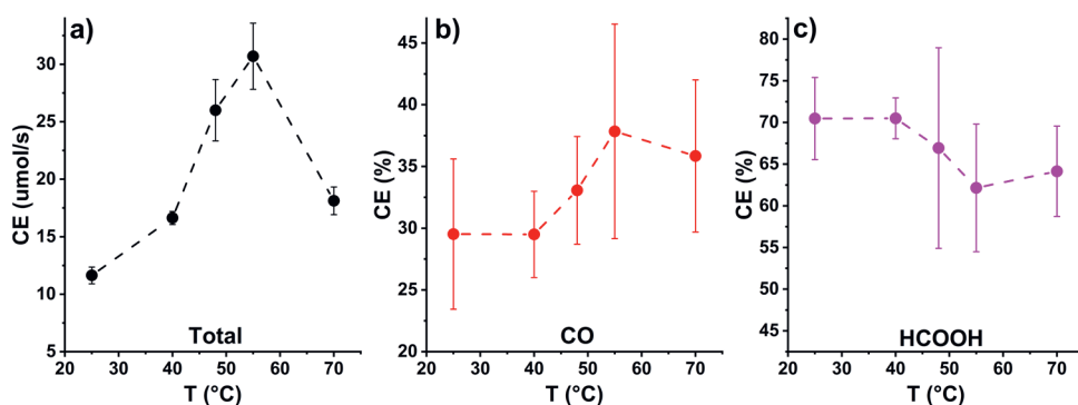
Figure B.7 a) Total consumption of CO 2 of CO 2 RR at different temperatures in 0.1 M KHCO 3 at -0.7 V vs. RHE and the carbon efficiency towards b) CO and c) HCOOH. Dotted lines are a guide to the eye and error bars are determined from at least 3 measurements.
