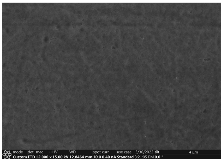
Figure B.25 SEM micrographs after CO 2 RR at -1.1V vs. RHE at a) 25 °C b) 48 °C c) 70 °C
