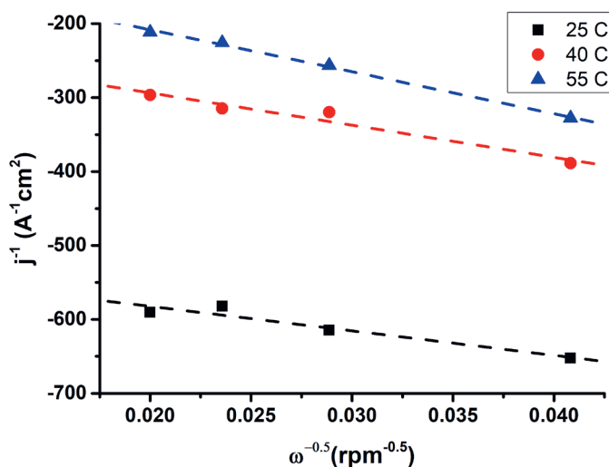
Figure A.7 Koutecky-Levich plot of CO 2 RR towards CO at -0.8V vs RHE
