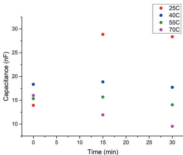
Figure B.26 Capacitance measured by double layer capacitance studies from CVs in the range -0.2 to 0.3 V vs. RHE at scan rates from 200 to 1400 mV/s before and after 15 and 30 min of CO 2 RR at different temperatures. The capacitance was determined at 0.0 V vs. RHE.
