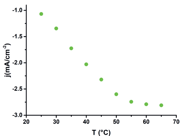
Figure A.2 The partial current density of CO 2 RR towards CO formation at -0.7V vs RHE plotted against temperature in 0.1M NaHCO 3 to illustrate the plateau in the activity starting around 55 °C.
