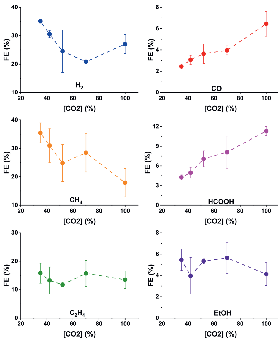
Figure B.8 Faradaic efficiency of CO 2 RR at different CO 2 bulk concentrations by changing the partial pressure in 0.1 M KHCO 3 at -1.1 V vs. RHE for a) hydrogen b) CO c) methane d) formic acid e) ethylene f) ethanol g) 1-propanol. Dotted lines are a guide to the eye and error bars are determined from at least 3 measurements.
