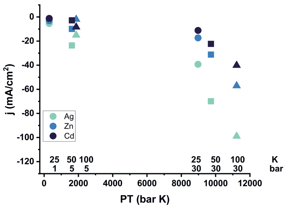
Figure G.6 The partial current density for CO 2 RR as function of pressure and temperature for Ag, Zn and Cd. Both temperature and pressure increase the CO 2 RR current density, except when high temperatures are used at low pressures
