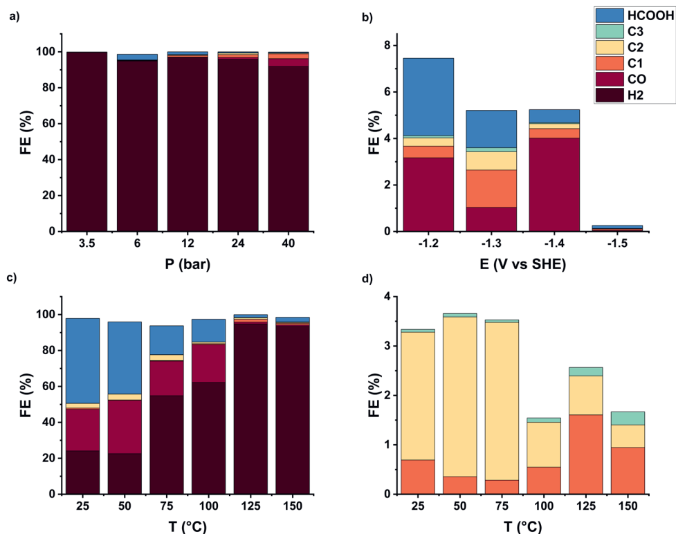
Figure F.5 Faradaic efficiencies for the CO 2 RR reduction as function of a) pressure at 24 bar and -1.3 V vs SHE b) potential at 24 bar and 125 °C and c and d) temperature at 24 bar and -1.3 V vs SHE. a) and c) show total FE. b) shows the CO 2 RR products with the remaining FE being H 2 and d) shows only the hydrocarbons
