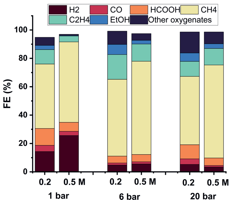
Figure F.17 Faradaic efficiency as function of pressure and electrolyte concentration at room temperature and -1.5 V vs SHE.
