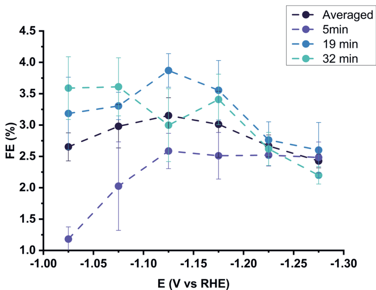
Figure D.12 Faradaic efficiency as function of potential and time on Ni in 0.1 M KHCO 3 at 18 °C
