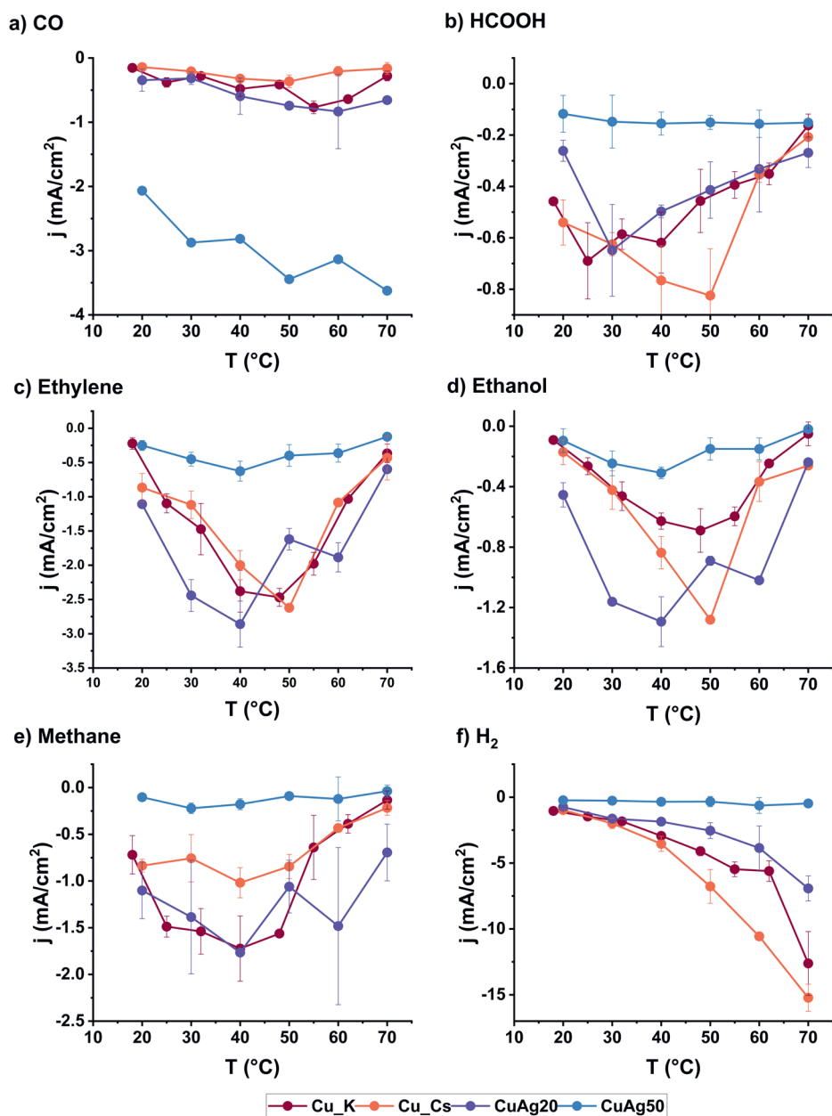
Figure C.17 Comparison of the partial current densities for a) CO b) HCOOH c) ethylene d) ethanol e) methane f) for Cu, CuAg20 and CuAg50 at -1.1\text{V} vs RHE in 0.1\text{ M CSHCO}_3 and also in 0.1\text{ M KHCO}_3 for Cu.
