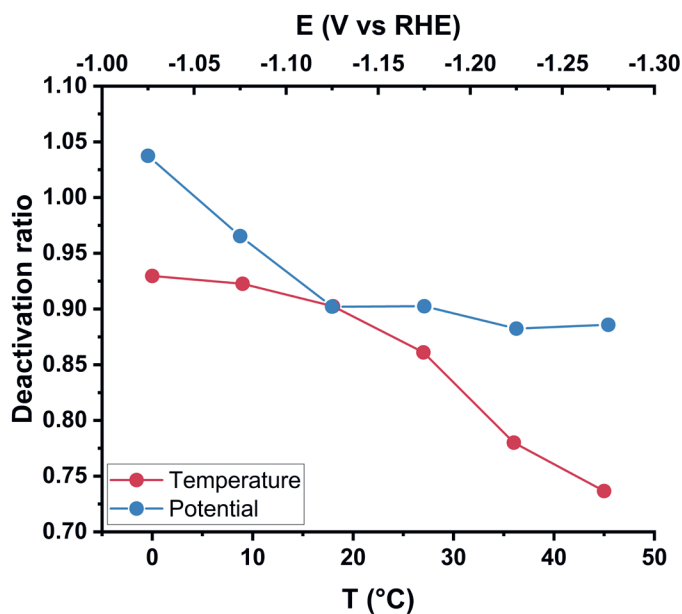
Figure D.8 Deactivation ratio as function of temperature and potential
