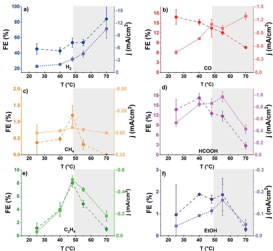
Figure B.4 Faradaic efficiency (in dark circles) and partial current density (in light squares) of CO 2 RR at different temperatures in 0.1M KHCO 3 at -0.95V vs. RHE for a) hydrogen b) CO c) methane d) formic acid e) ethylene f) ethanol g) 1-propanol. Dotted lines are a guide to the eye and error bars are determined from at least 3 measurements.
