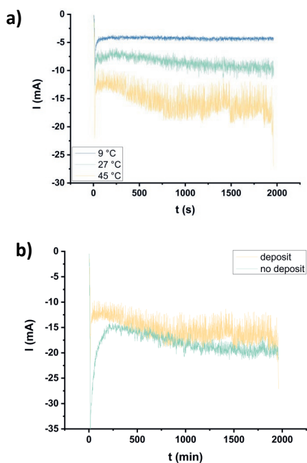
Figure D.9 a) Time dependence of current at different temperatures b) Time dependence of current at 45 °C both with the deposited electrode and the plain Ni electrode
