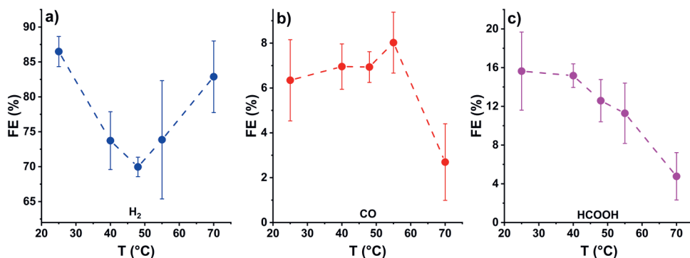
Figure B.6 Faradaic efficiency of CO 2 RR at different temperatures in 0.1 M KHCO 3 at -0.7 V vs. RHE for a) hydrogen b) CO c) formic acid
