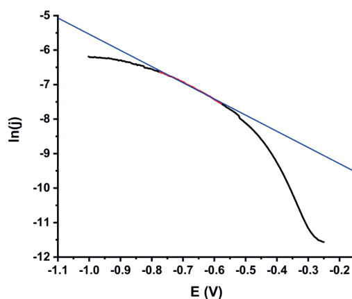
Figure A.1 Determination of the exchange current density using an extrapolation in the Tafel plot of the partial current density for CO formation
