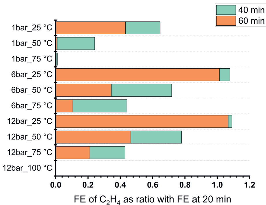
Figure F.12 Stability as function of temperature and pressure. Stability is here defined as the FE that remains after 40 and 60 minutes compared to the FE at 20 minutes at a certain condition.
