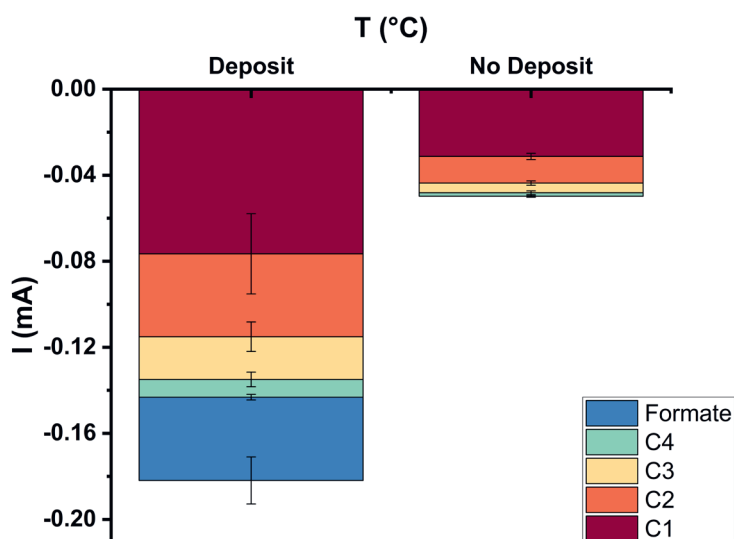
Figure D.3 Activity for CO 2 reduction on a polished polycrystalline Ni electrode with and without Ni deposition. Deposition shows higher activities at -1.175 V vs RHE at 18 °C
