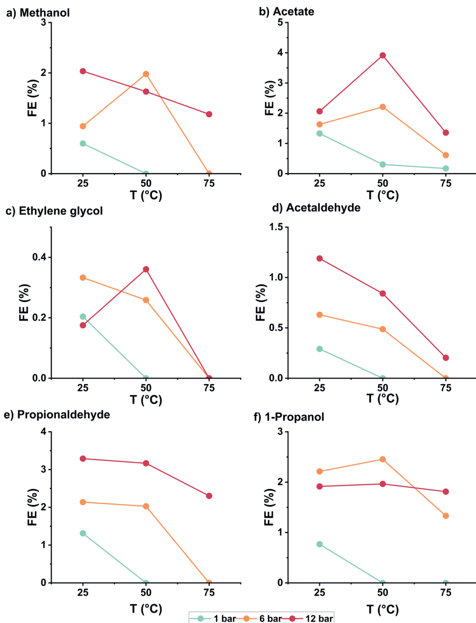
Figure F.10 Faradaic efficiency towards the minor CO 2 RR products at different pressures as function of temperature at -1.5 V vs SHE in 0.2 M KHCO 3 . FE for a) methanol b) acetate c) ethylene glycol d) acetaldehyde e) propionaldehyde f) 1-Propanol
