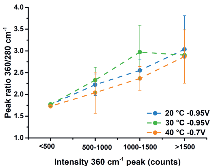
Figure B.12 The ratio between 360 and 280 \text{cm}^{-1} peak areas on Cu in 0.1 M \text{KHCO}_3 vs. the peak intensity of the 360 \text{cm}^{-1} peak, which is used as a proxy for the intensity of the Raman spectra. Three different conditions are shown to illustrate that this trend is not a coincidence. It can be seen that the ratio depends on the intensity of the peaks: at higher intensities the peak area ratio increases.
