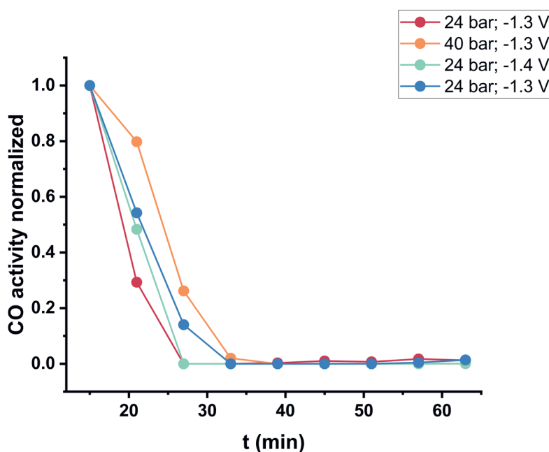
Figure F.7 The normalized CO activity as function of time for several conditions, all at 125 °C. This illustrates that CO is only produced at the start of the experiment as it decreases rapidly and from 32 min the activity is 0
