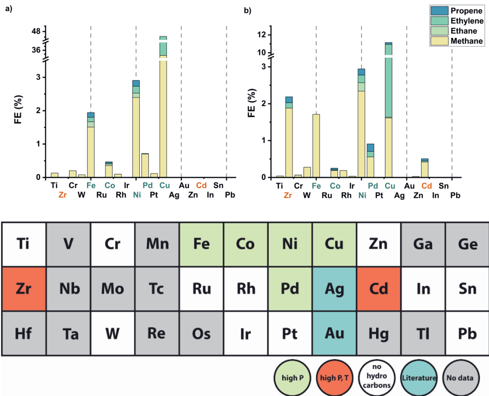
Figure G.10 Hydrocarbon production for all metals studied at a) 30 bar and 25 °C and b) 30 bar and 100 °C. The metals in green can produce longer hydrocarbons already at 25 °C, while the orange metals only produce these at higher temperatures. For the metals in blue hydrocarbons have been found in literature with more than 0.1% FE 14 , for the metals in gray no hydrocarbons longer than methane have been observed in this study at – 1.5V vs SHE in 0.1 M KHCO 3
