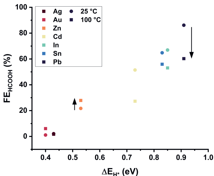
Figure G.8 Trend of formic acid efficiency with increasing temperature at 30 bar plotted vs hydrogen binding energy.
