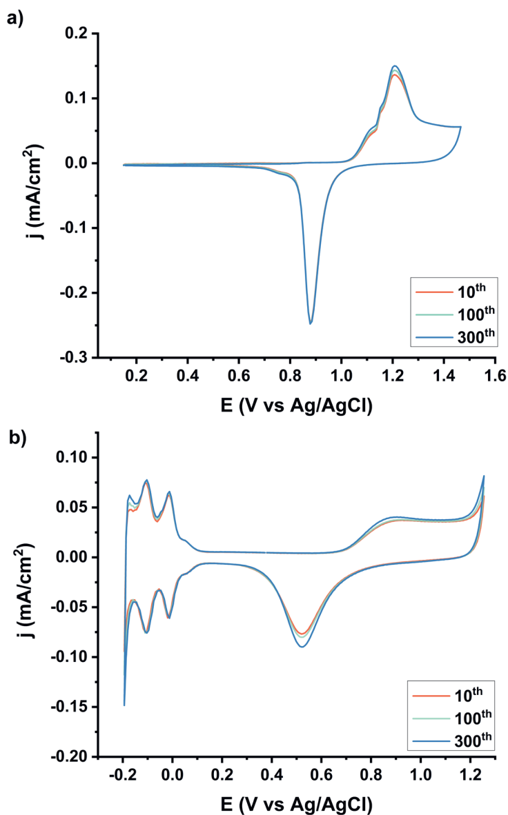
Figure E.2 Cyclic voltammograms of a) Au and b) Pt in 0.1M H_2SO_4 at scan rate of 100 mV/s, 0 barg, and 22°C.
