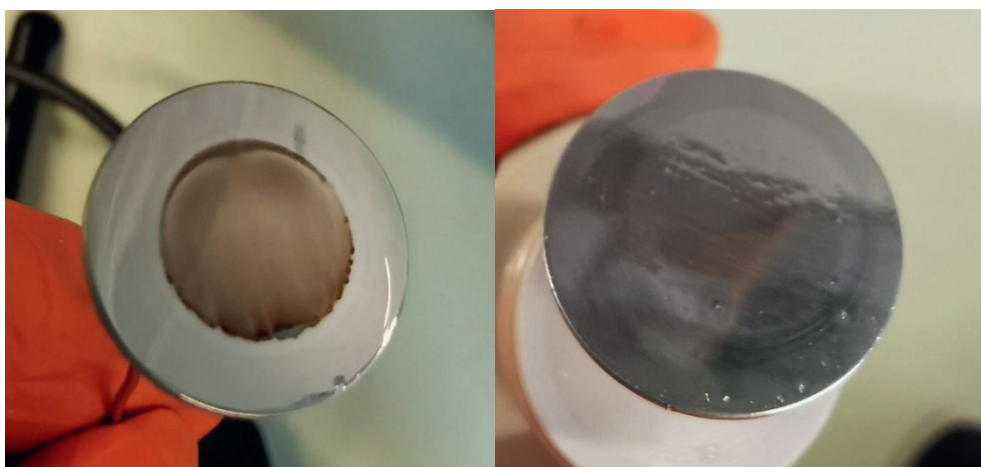
Figure D.10 Photographs of the electrode after a) CO 2 RR and b) HER showing that the coke only forms after CO 2 RR
