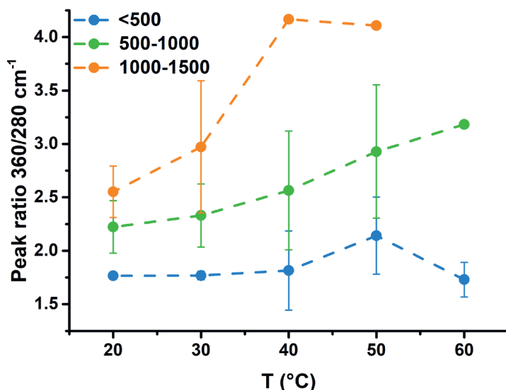
Figure B.13 The ratio between 360 and 280 cm -1 peak area on Cu in 0.1 M KHCO 3 vs. temperature at -0.95 V vs. RHE. It can be seen that the intensity of the Raman spectra, here indicated by the peak intensity of the 360 cm -1 peak, influences the peak ratio. The effect of temperature on the peak ratio and thus the CO coverage is more pronounced with more intense peaks.
