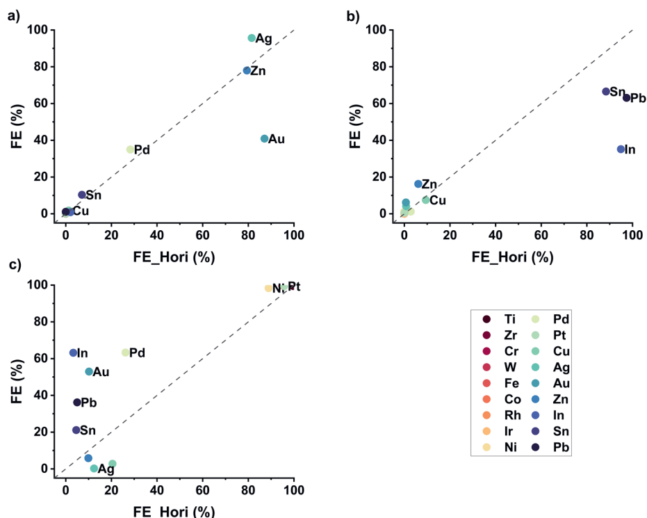
Figure G.5 Comparison of Faradaic efficiency at 1 bar and room temperature between this study and the study of Hori et al. 6 The dotted line shows the same efficiency; above this line, our study shows higher efficiencies, and below this line, the study of Hori shows higher efficiencies. a) shows the Faradaic efficiency towards CO, b) towards HCOOH and c) towards H 2 .
