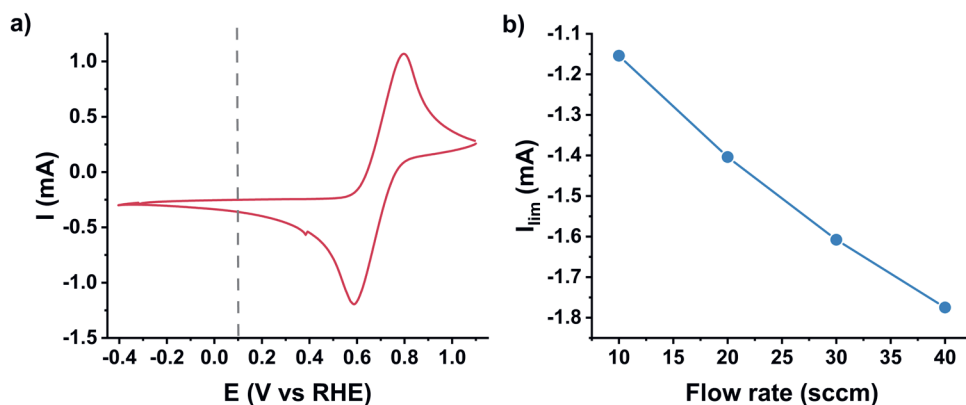
Figure C.8 a) the CV of \text{K}_3\text{Fe}(\text{CN})_6 at 20 mV/s without an flow in \text{CO}_2 saturated 0.1 M \text{KHCO}_3 b) the limiting current of \text{K}_3\text{Fe}(\text{CN})_6 at 0.1 V vs RHE in the GC cell showing that increased flow rates lead to improved mass transport
