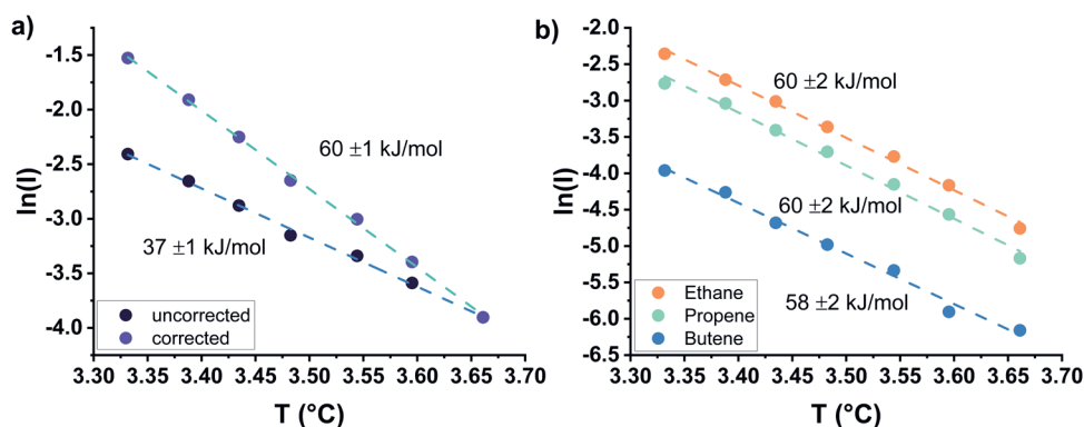
Figure D.15 a) Arrhenius plot after 5 min for methane, b) and for the other hydrocarbons which have similar activation energies
