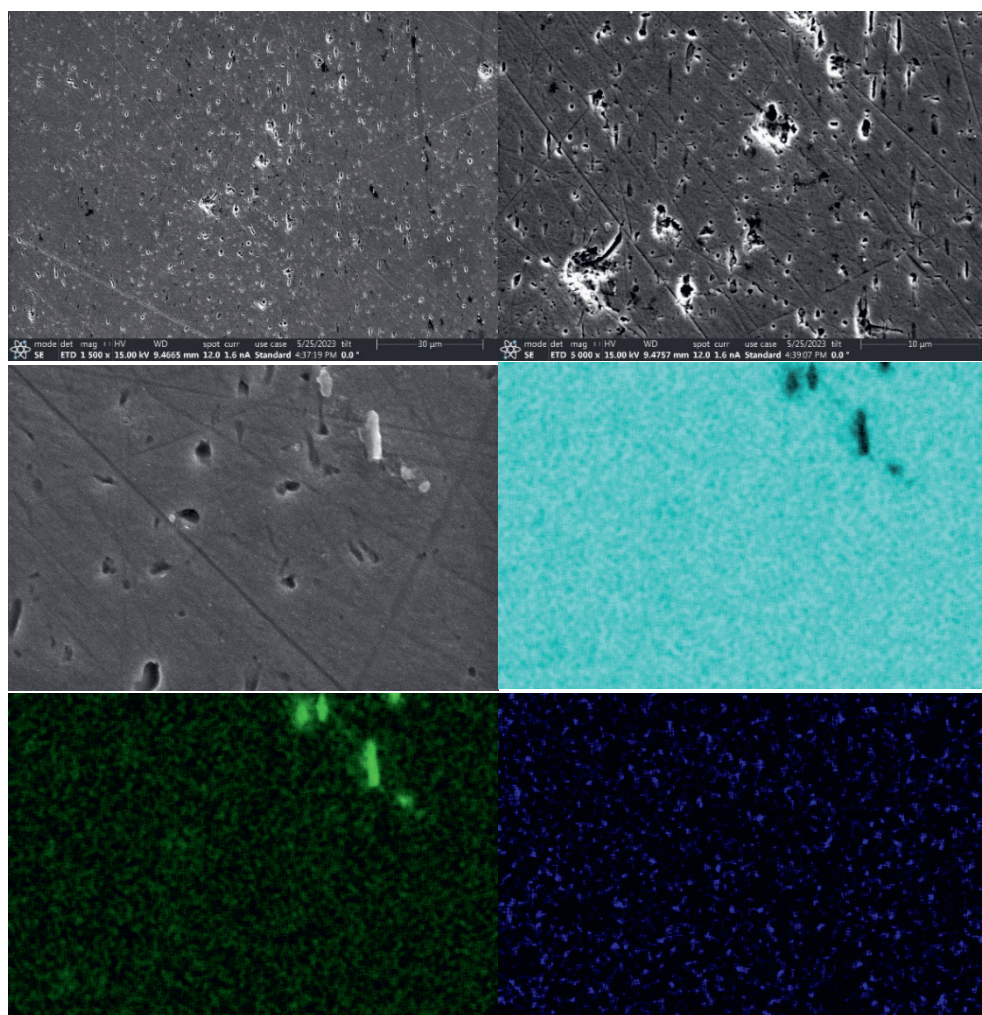
Figure D.2 SEM image of the Ni deposited electrode after CO 2 RR for 32 minutes at respectively a) 1500 and b) 5000 magnification. EDX maps at 50 000 magnification showing c) the SEM image d) nickel e) oxygen f) phosphorus.
