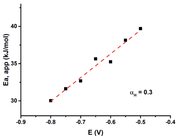
Figure A.12 The apparent activation energy of CO_2 reduction towards CO formation in 0.1M CsHCO_3 plotted against the applied potential
