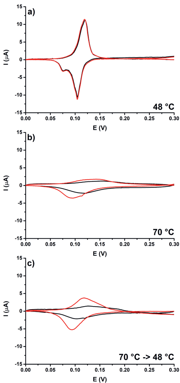
Figure B.23 Pb UPD CVs from 0.3 to 0.0 V vs. RHE at 5 mV/s in 0.1 M \text{NaClO}_4 + 1mM \text{NaCl} + 2 mM \text{PbClO}_4 . a) after CO2RR for 20 min at -1.1V vs. RHE in 0.1M \text{KHCO}_3 at a) 48 °C b) 70 °C and c) 20 min at 70 °C and 30 min at 48 °C. The red and black line represent two different measurements.
