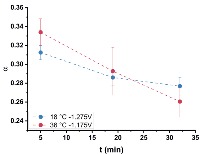
Figure D.13 Chain growth probability in time for 2 different experiments with similar activity showing that higher temperature causes deactivation of the catalyst
