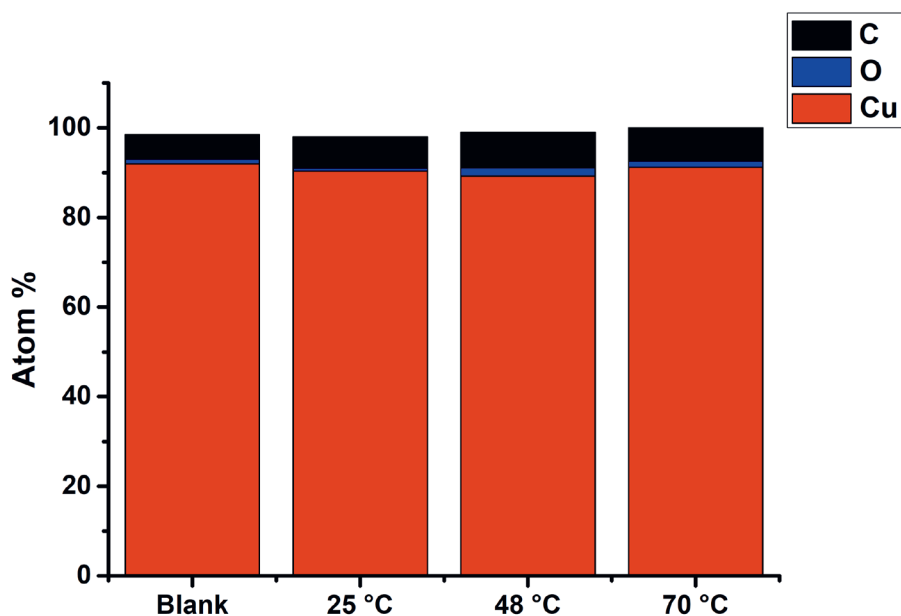
Figure B.24 Elemental composition measured using SEM-EDX of the copper surface after CO 2 RR at -1.1V at different temperatures and the blank before CO 2 RR
