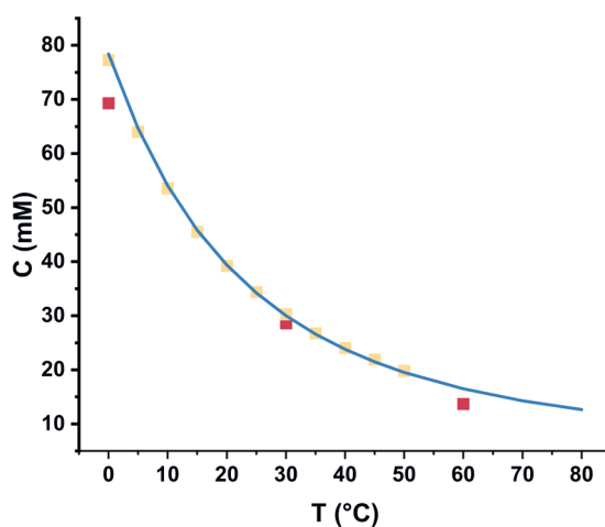
Figure C.3 the CO 2 concentration in water (yellow 1 , red 2 , blue 3 ) as function of temperature
