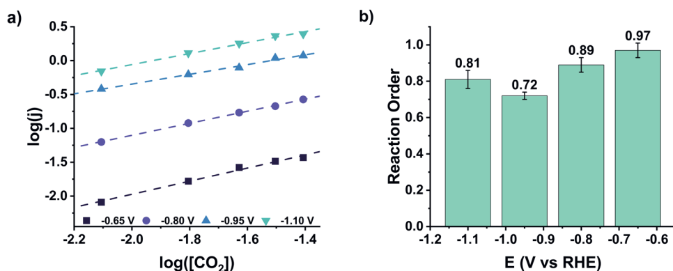
Figure C.6 Reaction order of CO 2 at different potentials in 0.1 M KHCO 3 . From the plot in a) the reaction order in b) has been determined
