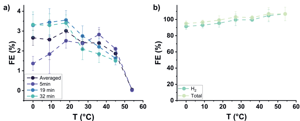
Figure D.7 Faradaic efficiency as function of temperature on Ni in 0.1 M KHCO 3 at -1.175 V vs RHE towards a) the total hydrocarbon formation (C1 up to C4 hydrocarbons) during CO 2 reduction both averaged and as function of time and b) towards H 2 and total FE
