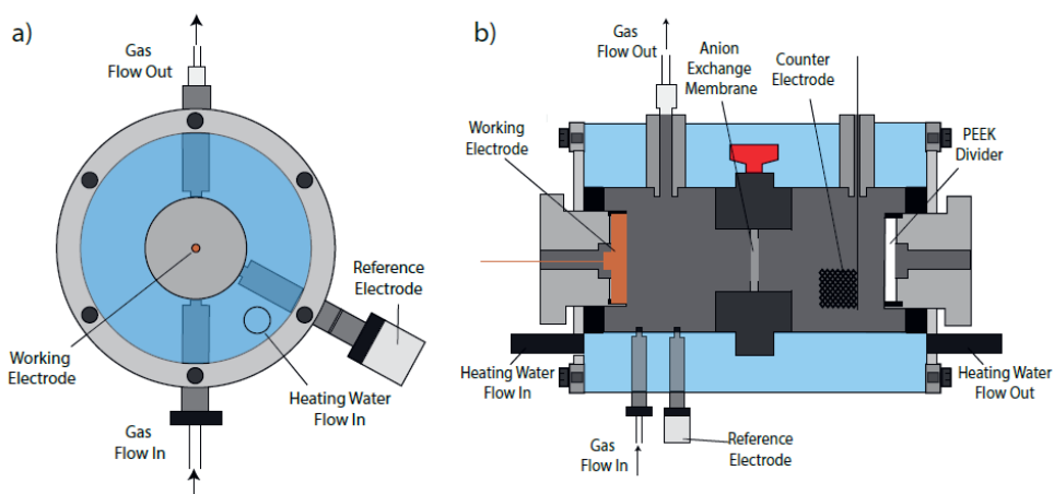
Figure B.2 Schematics of the H-cell surrounded by the water jacket used to control the temperature. a) Frontal-section of the cathodic chamber and (b) cross-section of the electrochemical H-cell with heating jacket
