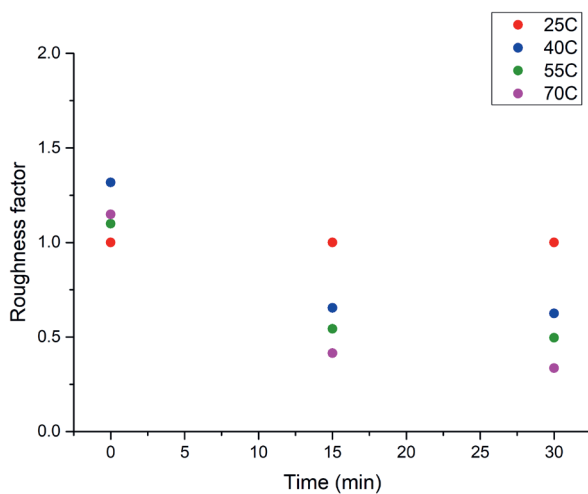
Figure B.27 Roughness factor determined from the data from Figure B.23 by setting the capacitance at 25 °C as 1 at every time interval and normalize the other values.
