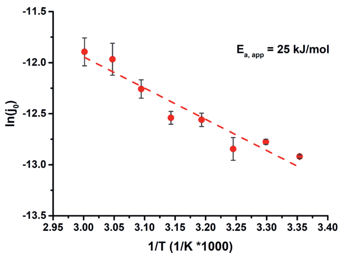
Figure A.11 Arrhenius plot of HER in Ar saturated 0.1M NaHCO 3
