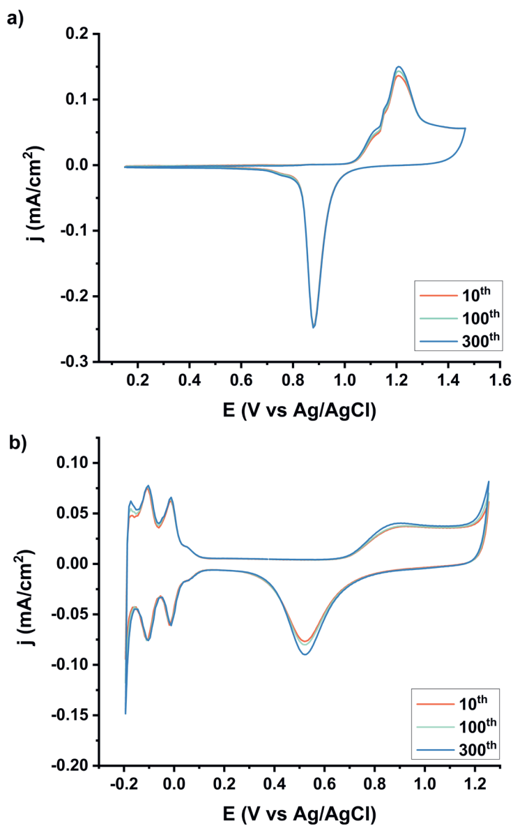
Figure E.2 Cyclic voltammograms of a) Au and b) Pt in 0.1M H_2SO_4 at scan rate of 100 mV/s, 0 barg, and 22°C.
