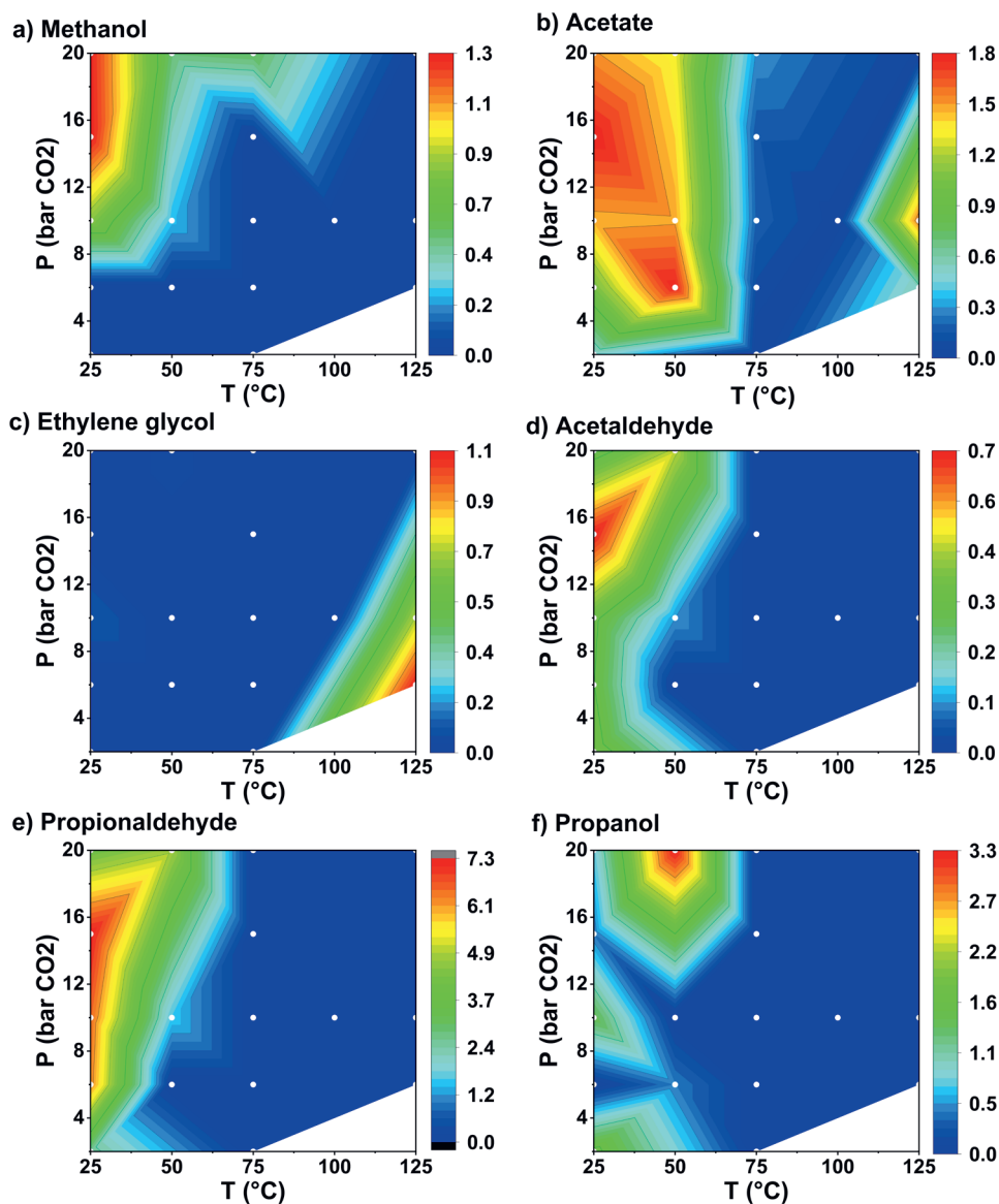
Figure F.1 Faradaic efficiency towards the minor CO 2 RR products as function of temperature and pressure at -1.4 V vs SHE in 0.2 M KHCO 3 with a 50/50 ratio of CO 2 and Ar. The white dots give the measured points and the maps are constructed via interpolation between these points. FE for a) methanol b) acetate c) ethylene glycol d) acetaldehyde e) propionaldehyde and f) 1-propanol
