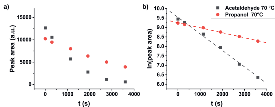
Figure C.19 Illustration of the evaporation experiments, a) the peak area and b) \ln of the peak area of acetaldehyde and propanol at 70 °C vs. time
