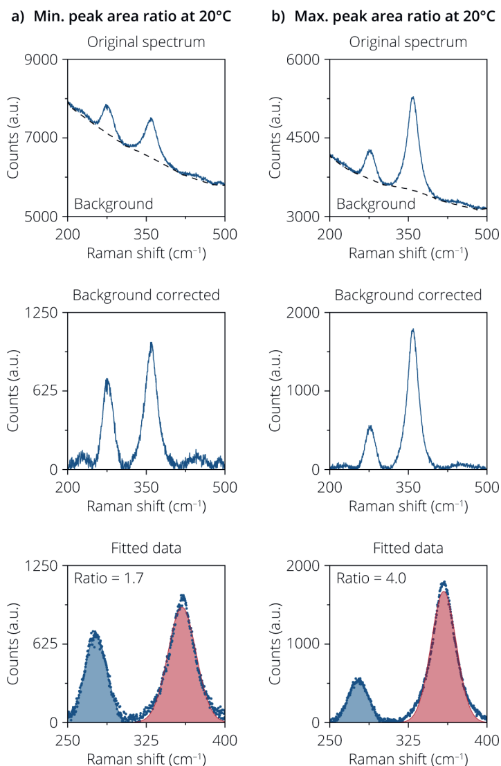
Figure B.11 Example of the data processing of the Raman data. Panel a) shows an example with small peak area ratios and b) with large peak area ratios. From top to bottom the Figure B.shows the original spectrum, the background corrected spectrum and then the data that is fitted with a Gaussian peak fitting procedure to calculate the area of the 280 \text{cm}^{-1} and 360 \text{cm}^{-1} peaks in blue and red, respectively.
