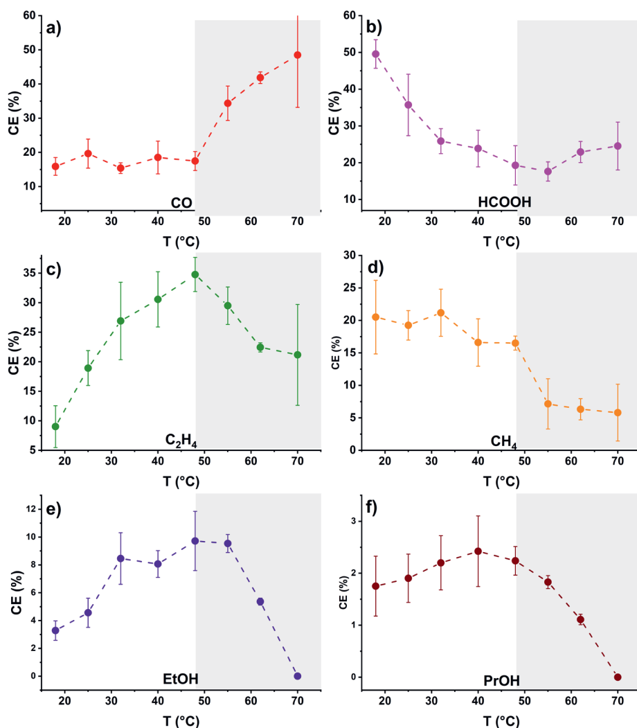
Figure B.3 Carbon Efficiency of CO 2 RR at different reaction temperatures in 0.1 M KHCO 3 at -1.1 V vs. RHE for a) CO b) formic acid c) ethylene d) methane e) ethanol, and f) 1-propanol. The error bars are determined from at least 3 separate experiments. The gray background indicates the second regime and the dotted lines are a guide to the eye.
