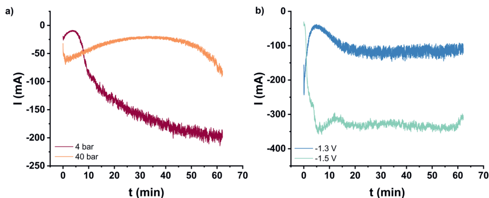
Figure F.4 Current as function of time for a) 4 and 40 bar at -1.5 V vs SHE at 75 °C and b) 24 bar at 125 °C at -1.3 V and -1.5 vs SHE. This illustrates that at elevated temperatures the current is not stable, especially at low pressures as seen in a). In b) the typical current profile at 125 °C and -1.3 V is observed, where the current is unstable in the first 20 minutes and first decreases and then increases again after which it stabilizes. It also shows the instability at higher overpotentials, where even the smallest electrode goes to currents above -300 mA, while at the start it was only -30 mA.
