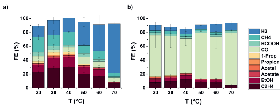
Figure C.14 Faradaic efficiencies for a) CuAg20 b) CuAg50 as function of temperature at -1.1 V vs RHE in 0.1 M CsHCO 3
