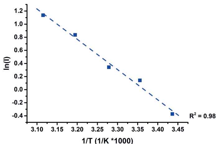
Figure B.19 Arrhenius plot of H_2 production during CO_2RR at -1.1 V vs. RHE in -0.1 M KHCO_3 . The striped line gives the trendline with the corresponding R^2 value to illustrate the linearity of the trendline.
