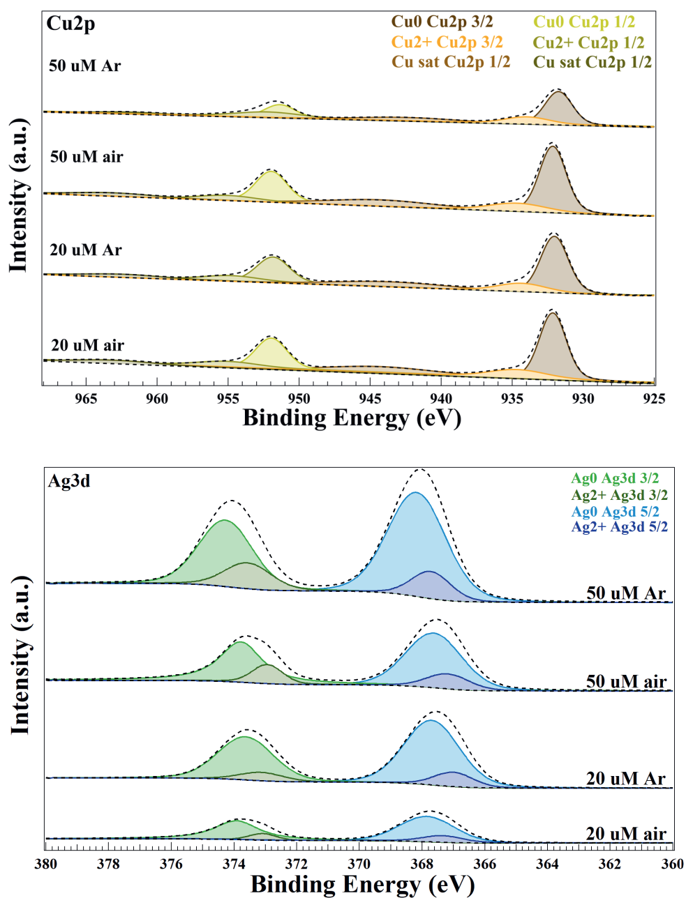
Figure C.11 the fitted Cu2p and Ag3d peaks determined with XPS
