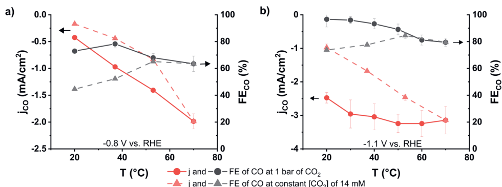
Figure C.5 Temperature effect of the partial current densities for CO and the FE for CO on Ag in 0.1 M KHCO 3 at constant CO 2 pressure of 1 bar for the full dark circles and at constant CO 2 concentration in electrolyte of 14 mM by changing the partial pressure accordingly in dashed light triangles at a) at -0.8 V and b) -1.1 V vs RHE
