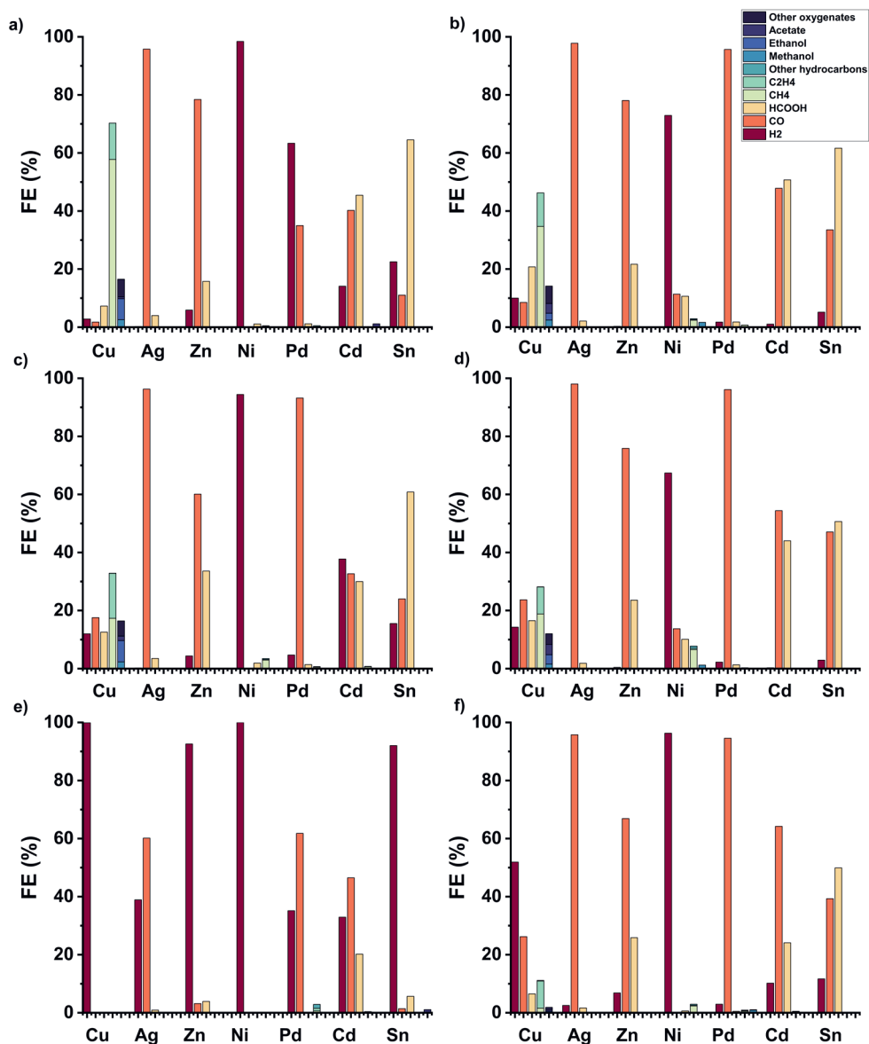
Figure G.1 Faradaic efficiency at six different conditions for Cu, Ag, Zn, Ni, Pd, Cd and Sn at -1.5 V vs SHE in 0.1 M KHCO 3 as shown in Figure 1 but categorized per condition a) 25 °C and 1 bar b) 25 °C and 30 bar c) 50 °C and 5 bar d) 50 °C and 30 bar e) 100 °C and 5 bar f) 100 °C and 30 bar
