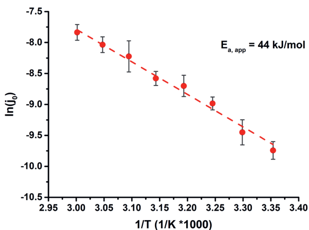
Figure A.9 Arrhenius plot of \text{CO}_2 reduction in 0.1M \text{NaHCO}_3 in the temperature range of 25\text{--}60^{\circ}\text{C} , not corrected for the changes in \text{CO}_2 concentration with temperature
