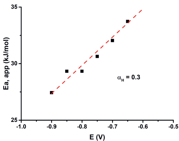
Figure A.12 The apparent activation energy of CO_2 reduction towards CO formation in 0.5M NaHCO_3 plotted against the applied potential
