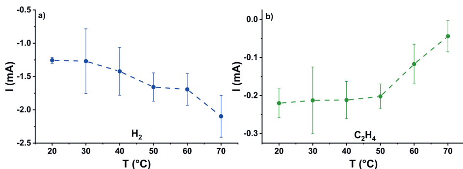
Figure B.18 Currents for CO reduction at different temperatures in 0.1 M KOH + 0.2 M K 2 SO 4 at -0.7 V vs. RHE for a) hydrogen and b) ethylene. Dotted lines are a guide to the eye and error bars are determined from at least 3 measurements.
