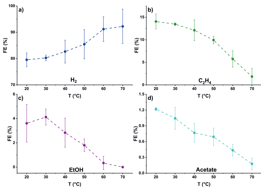
Figure B.17 Faradaic efficiency of CO reduction at different temperatures in 0.1 M KOH + 0.2 M K 2 SO 4 at -0.7 V vs. RHE for a) hydrogen b) ethylene c) ethanol, and d) acetate. Dotted lines are a guide to the eye and error bars are determined from at least 3 measurements.
