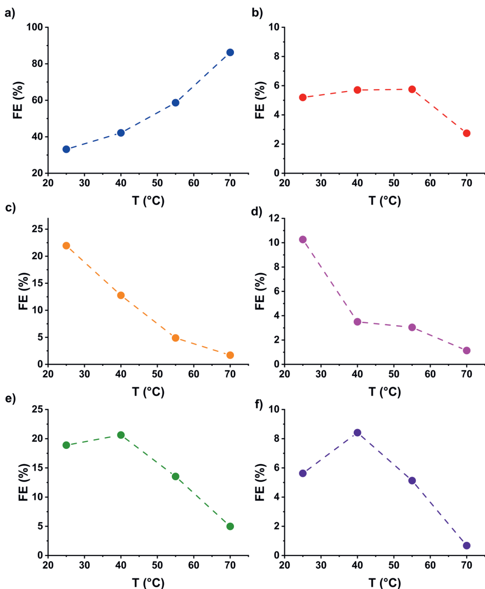
Figure B.9 Faradaic efficiency of CO 2 RR at different temperatures with constant CO 2 bulk concentrations by changing the partial pressure in 0.1 M KHCO 3 at -1.1 V vs. RHE a) hydrogen b) CO c) methane d) formic acid e) ethylene f) ethanol, and g) 1-propanol. Dotted lines are a guide to the eye and error bars are determined from at least 3 measurements.
