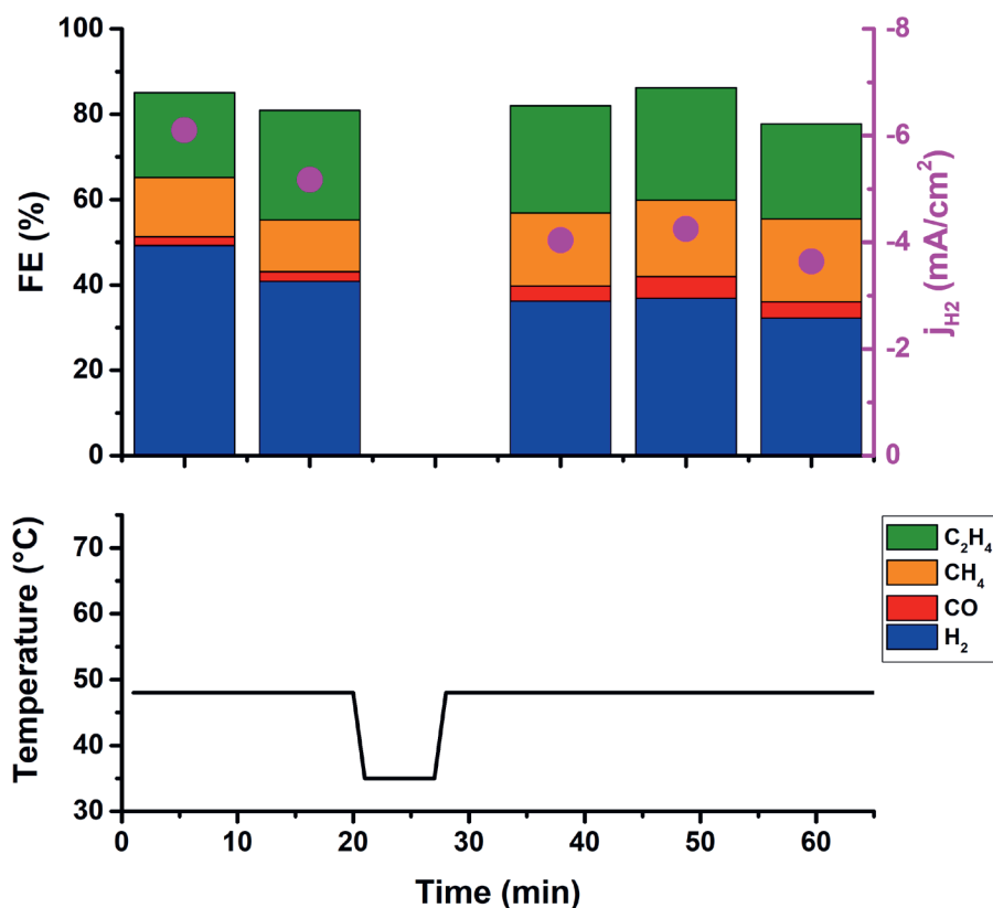
Figure B.28 Reversibility experiments, control experiment to Figure 6. The upper panel shows the Faradaic Efficiency of the gaseous products of CO 2 RR at -1.1V vs. RHE after 5 and 19 min at 48 °C, and after cooling down at 5, 19 and 32 min at 48 °C. The magenta dots show the partial current density towards H 2 . The lower panel shows the temperature profile.
