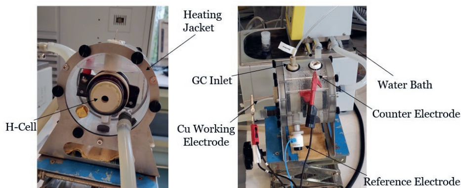
Figure B.1 Photos from the H-cell surrounded by the water jacket used to control the temperature
