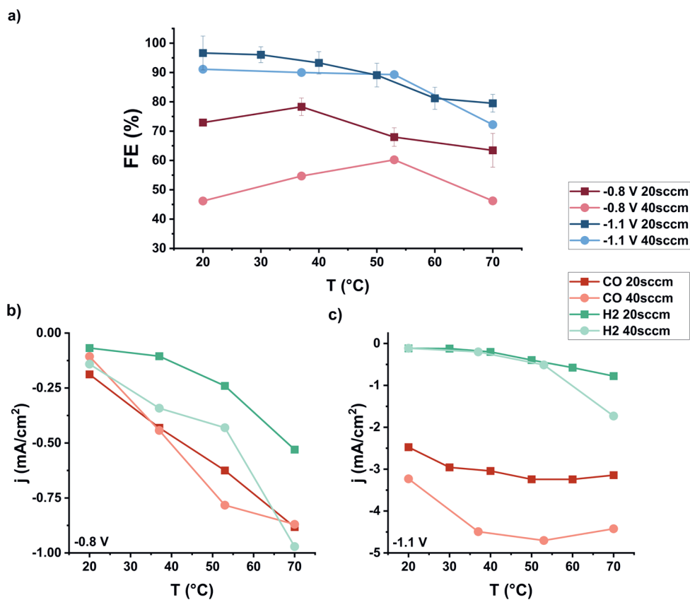
Figure C.9 Effect of mass transport on the CO 2 reduction on Ag in the GC cell in 0.1 M KHCO 3 on a) the Faradaic efficiency at different temperatures and the effect on the partial current densities to CO and H 2 at b) -0.8 V and c) -1.1 V vs RHE.
