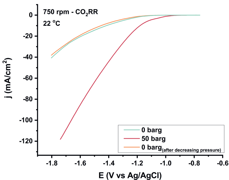
Figure E.5 Comparison of Linear sweep voltammograms (LSVs) in CO 2 -saturated 0.1M KHCO 3 before increasing pressure, then at 50 barg, and then returning pressure to 0 barg.
