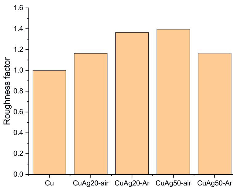
Figure C.10 Roughness factor determined from the double layer capacitance normalized to pure Cu
