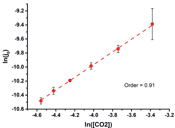
Figure A.6 The \ln of the exchange current density at different concentrations of \text{CO}_2 to determine the reaction order of \text{CO}_2
