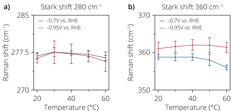
Figure B.16 Temperature- and potential-induced Stark tuning of the 280 cm -1 (left) and 360 cm -1 (right) peak maxima. The blue lines show the measurements at -0.7V vs. RHE, the orange lines at -0.95V vs. RHE. The data points are the average of 5–10 spots measured at every potential and temperature and the error bar shows the standard deviation of the peak positions of these spots.
