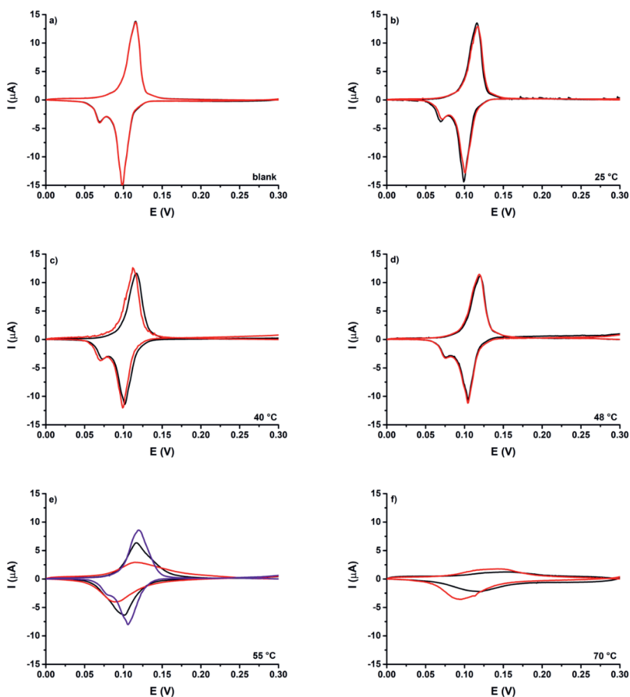
Figure B.21 Pb UPD CVs from 0.3 to 0.0 V vs. RHE at 5 mV/s in 0.1 M \text{NaClO}_4 + 1mM \text{NaCl} + 2 mM \text{PbClO}_4 . A) blank CV after only polishing before \text{CO}_2\text{RR} and after \text{CO}_2\text{RR} for 20 min at -1.1V vs. RHE in 0.1M \text{KHCO}_3 at b) 25 °C c) 40 °C d) 48 °C e) 55 °C f) 70 °C. The red, black and purple lines are separate experiments to illustrate reproducibility.
