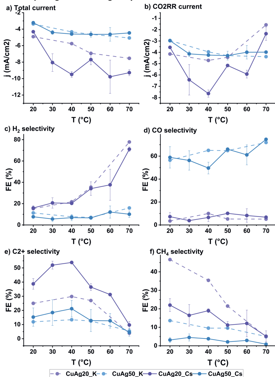
Figure C.15 a) Total current density and b) current density towards CO 2 RR and faradaic efficiency for c) hydrogen d) CO e) C 2 + products f) CH 4 for CuAg 20 in purple and CuAg 50 in blue at -1.1 V vs RHE in 0.1 M KHCO 3 (light dashed) and in 0.1 M CsHCO 3 (dark full line)
