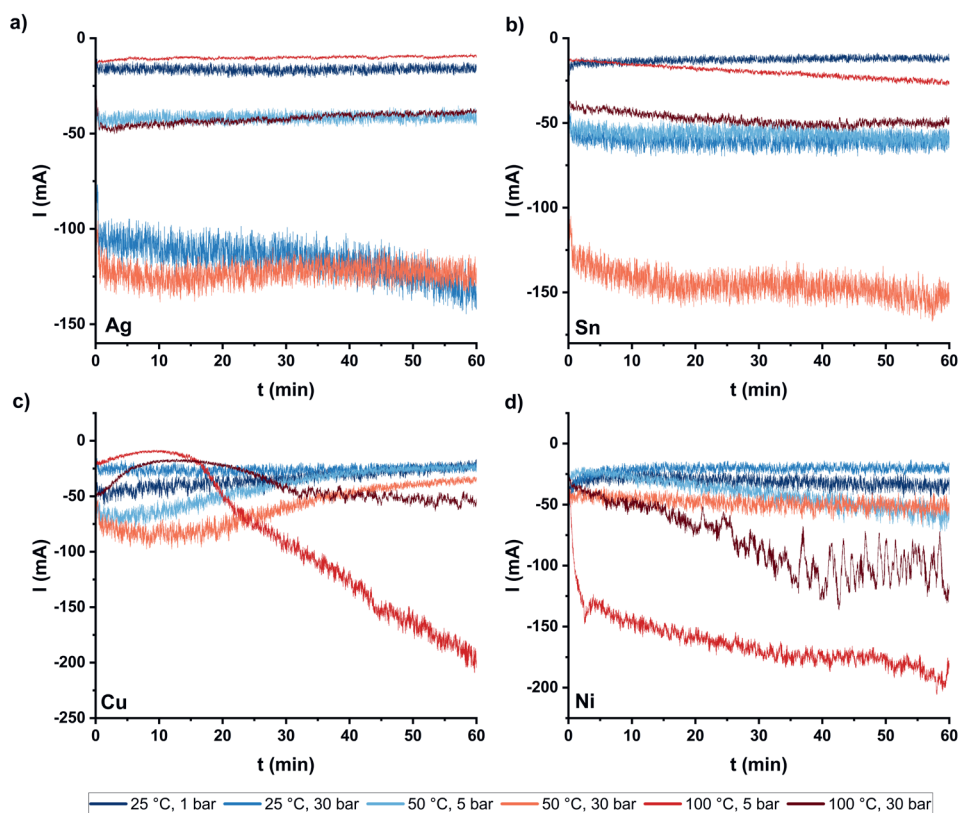
Figure G.3 Current vs time for the different conditions for a) Ag b) Sn c) Cu d) Ni. Higher temperatures lead to more unstable currents, especially on Cu and Ni.
