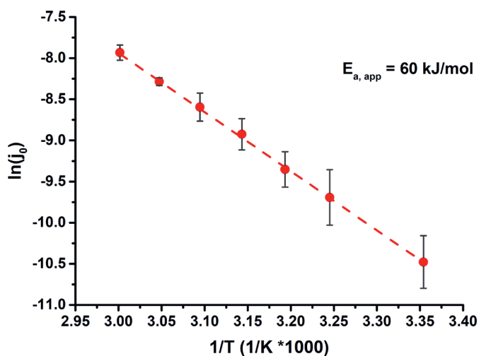
Figure A.10 Arrhenius plot of CO 2 RR towards CO formation in 0.1M NaHCO 3 using data from Figure 2.2, so at constant CO 2 concentration
