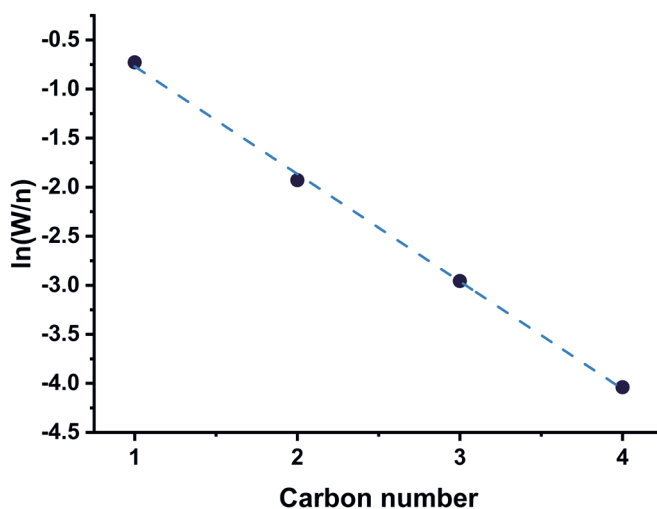
Figure D.6 Example of an Anderson-Flory plot to obtain the chain growth probability on the Ni electrode
