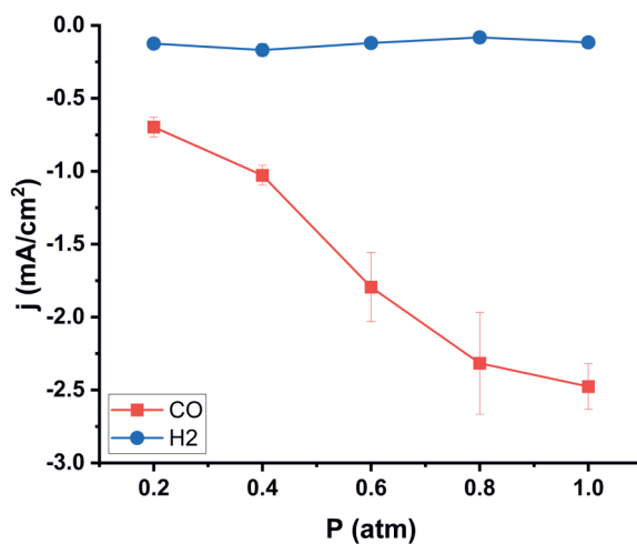
Figure C.4 Partial current densities at different partial pressures to change the bulk concentration of CO 2 at -1.1 V vs RHE at 20 °C in 0.1 M KHCO 3
