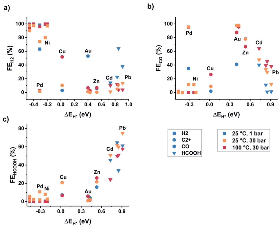
Figure G.7 The Faradaic efficiency at different experimental conditions for all metals tested as function of the binding energy determined by Bagger et al. 15 a) hydrogen b) CO and c) HCOOH. The symbol illustrates to which group the metal is typically classified.
