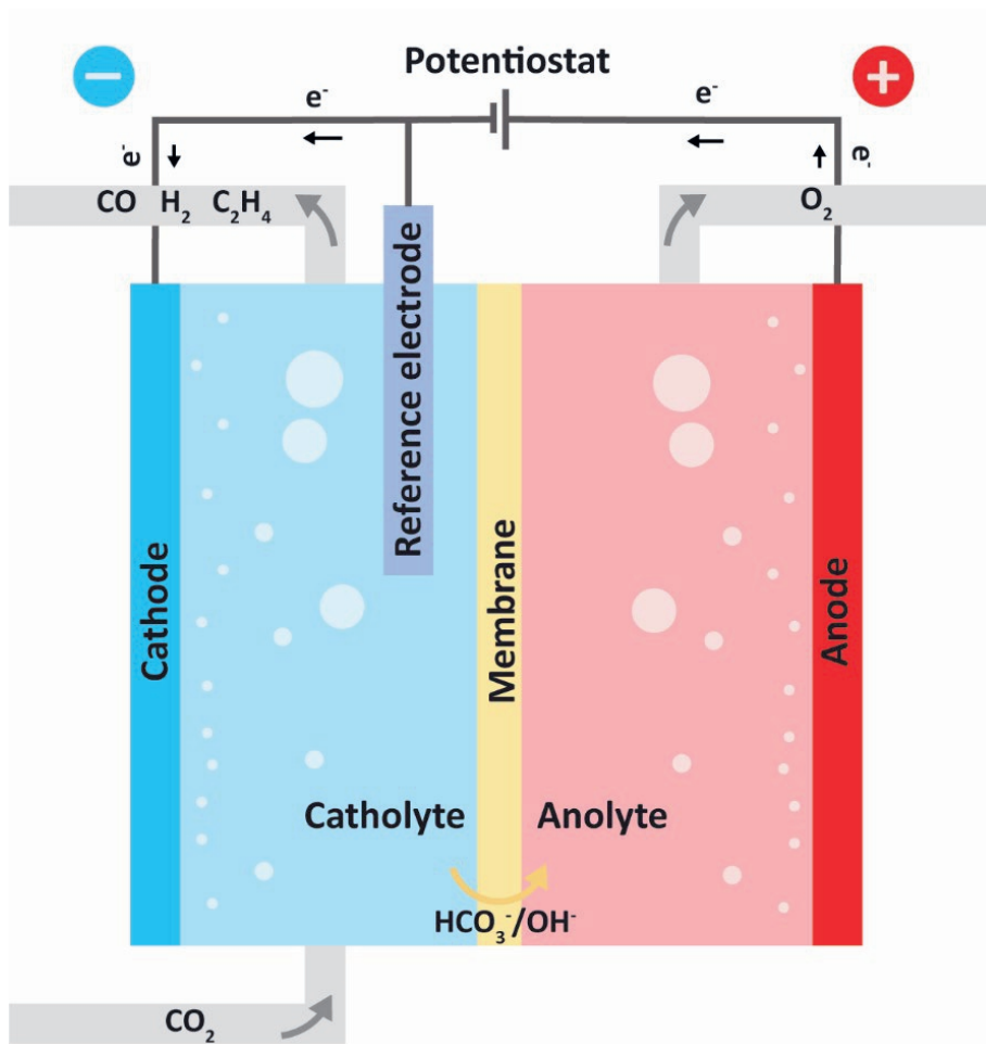
Figure 1.1 Pictorial representation of a three-electrode H-cell configuration for electrochemical CO 2 reduction where the cathode and anode are separated by an anion-exchange membrane
