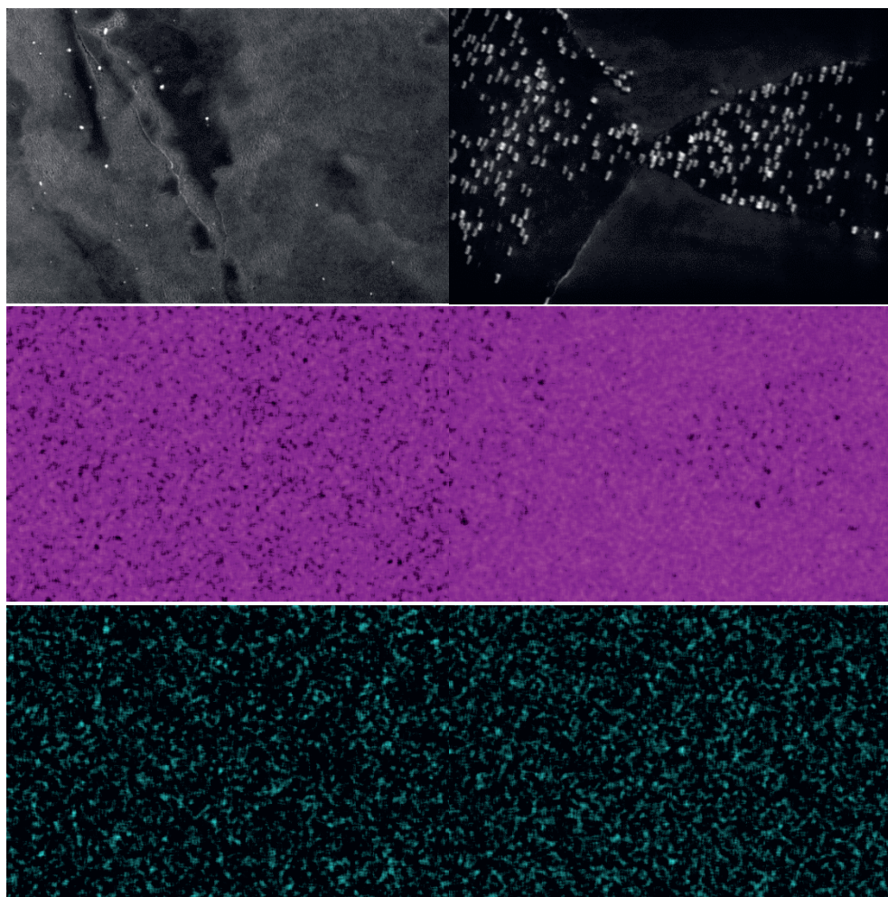
Figure C.13 EDX maps of the CuAg20 catalyst on the left and the CuAg50 catalysts on the right; pink is Cu, blue for Ag. The EDX map shows that Ag is uniformly distributed over the surface in both catalyst, as expected from galvanic exchange.
