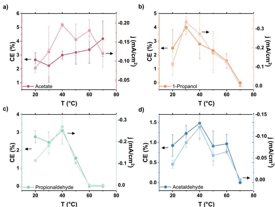
Figure C.18 Carbon efficiency and partial current density for minor liquid products on CuAg 20 at -1.1 V vs RHE in CsHCO 3 a) acetate b) 1- propanol c) propionaldehyde and d) acetaldehyde based on the HPLC data
