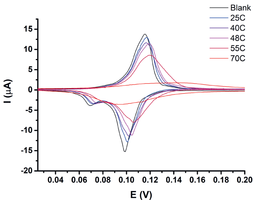
Figure B.22 Pb UPD CVs from 0.3 to 0.0 V vs. RHE at 5 mV/s in 0.1 M \text{NaClO}_4 + 1mM \text{NaCl} + 2 mM \text{PbClO}_4 . The copper sample was first used for \text{CO}_2\text{RR} for 20 min at -1.1V vs. RHE in 0.1 M \text{KHCO}_3 at different temperatures, while the blank is before \text{CO}_2\text{RR} was performed.
