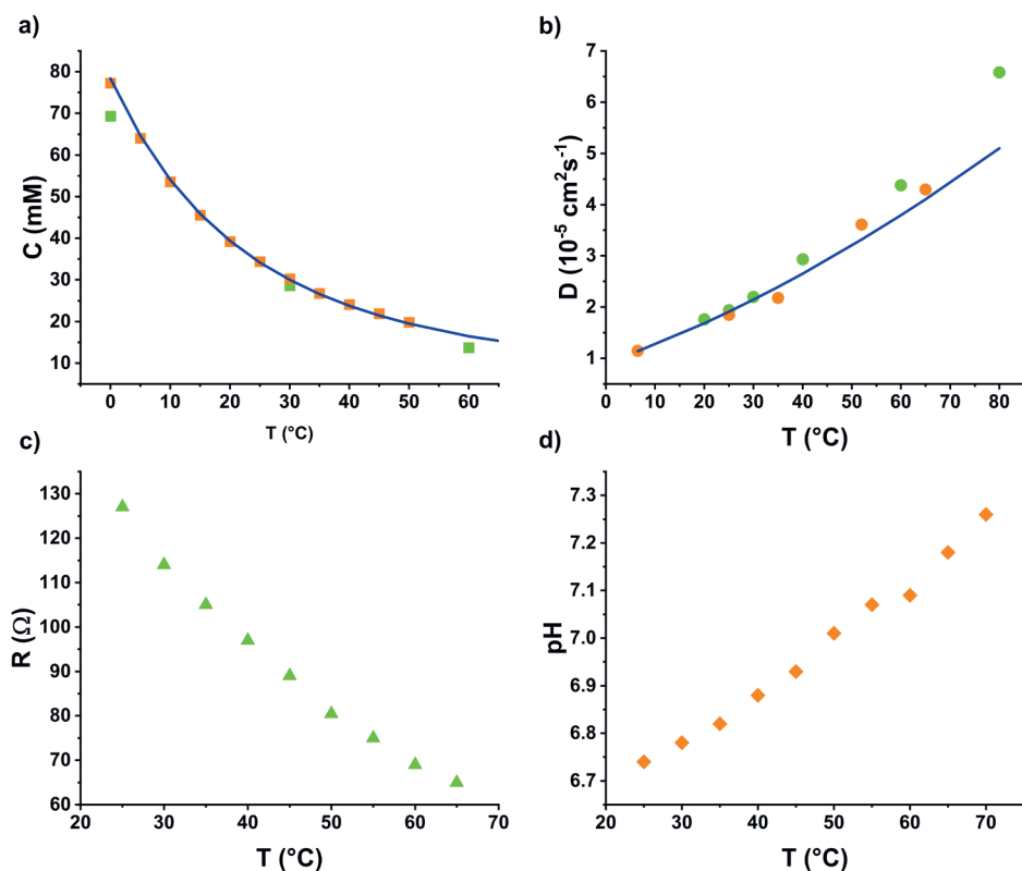
Figure A.4 Different parameters which change with temperature, (some values originate from literature); a) the CO 2 concentration in water (orange 3 , green 4 , blue 5 ), b) the diffusion coefficient of CO 2 in water (orange 6 , green 7 , blue 8 ), c) the resistance of 0.1M NaHCO 3 , d) the pH of 0.1M CO 2 saturated NaHCO 3
