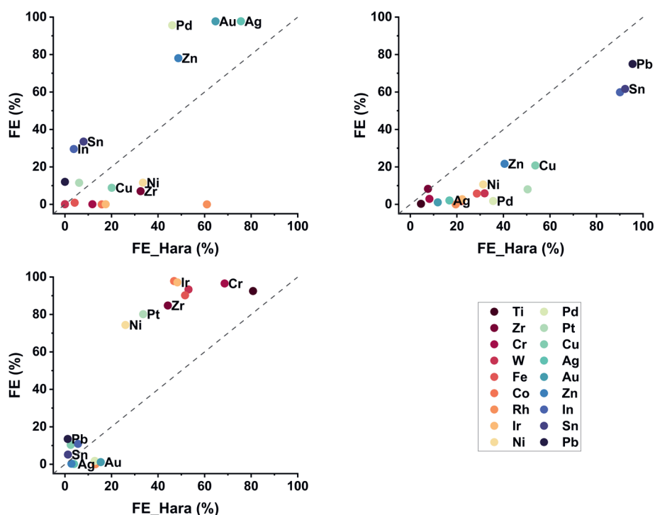
Figure G.4 Comparison of Faradaic efficiency at 30 bar and room temperature between this study and the study of Hara et al. 1 The dotted line shows the same efficiency; above this line, our study has higher efficiencies and below this line, the study of Hara shows higher efficiencies. a) shows the Faradaic efficiency towards CO, b) towards HCOOH and c) towards H 2 .
