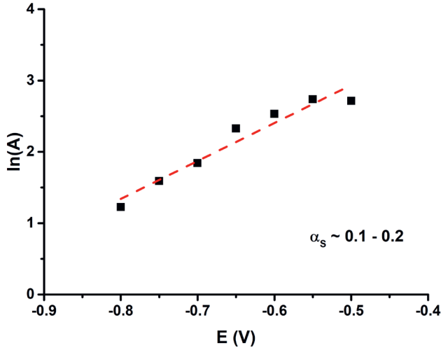
Figure A.14 The \ln of the pre-exponential factor plotted against the applied potential for \text{CO}_2 reduction towards \text{CO} in 0.1\text{M NaHCO}_3
