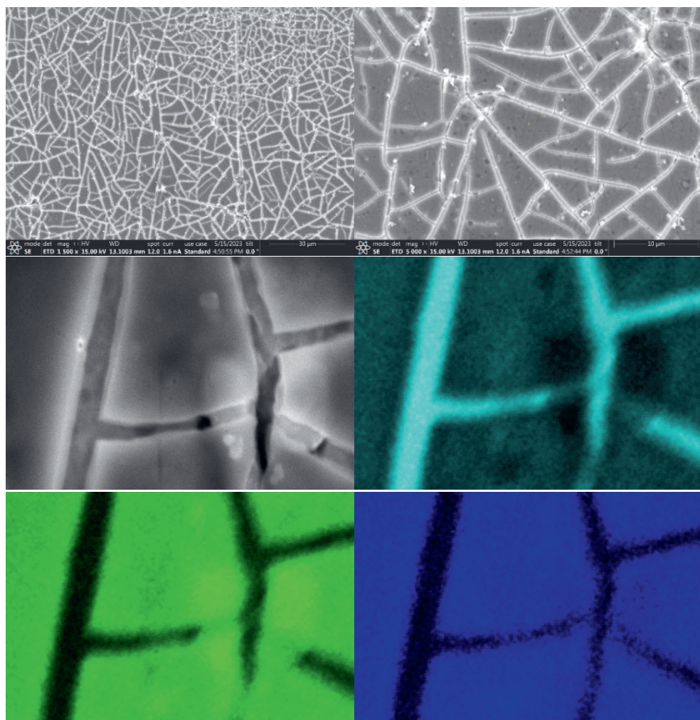
Figure D.1 SEM image of the Ni deposited electrode before CO 2 RR at respectively a) 1500 and b) 5000 magnification. EDX maps at 50 000 magnification showing c) the SEM image d) nickel e) oxygen f) phosphorus.
