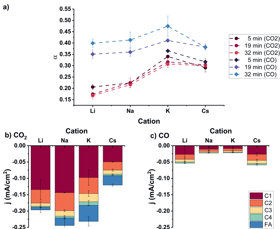
Figure 5.4 a) Chain growth probability for different cations for both CO 2 RR and CORR b) activity for CO 2 RR for different cations at -1.175 V vs RHE and c) activity for CORR for different cations at -1.075 V vs RHE on the Ni catalyst in 0.1 M KHCO 3
