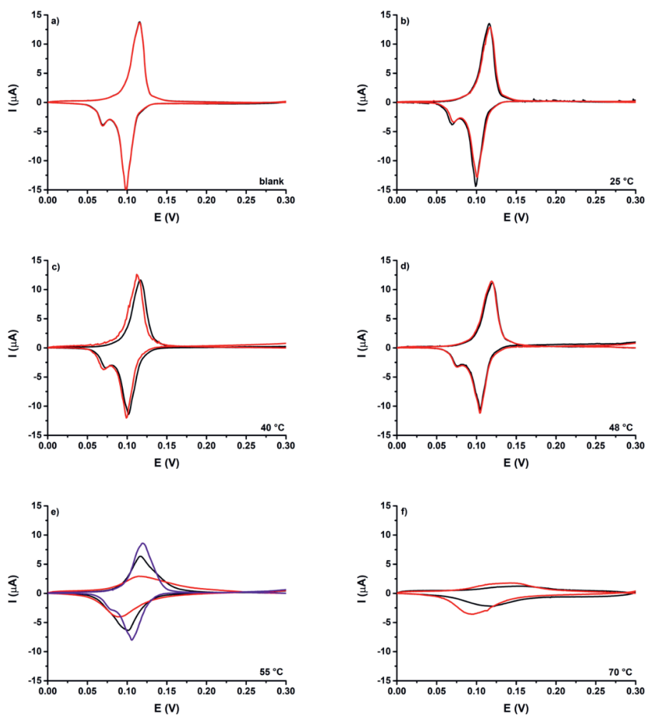
Figure B.21 Pb UPD CVs from 0.3 to 0.0 V vs. RHE at 5 mV/s in 0.1 M NaClO 4 + 1mM NaCl + 2 mM PbClO 4 . A) blank CV after only polishing before CO 2 RR and after CO 2 RR for 20 min at -1.1V vs. RHE in 0.1M KHCO 3 at b) 25 °C c) 40 °C d) 48 °C e) 55 °C f) 70 °C. The red, black and purple lines are separate experiments to illustrate reproducibility.
