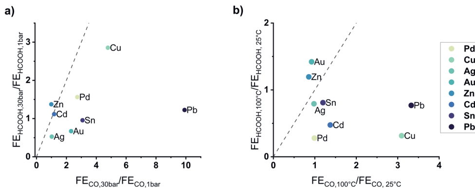
Figure G.9 The ratio between the Faradaic efficiency for HCOOH plotted against the ratio between Faradaic efficiency for CO to illustrate if relatively more CO or HCOOH is produced. The dotted line shows where both CO and HCOOH increase with the same amount; below the line CO increases stronger and above the line HCOOH increases stronger. a) shows the effect of pressure at 25 °C and b shows the effect temperature at 30 bar.
