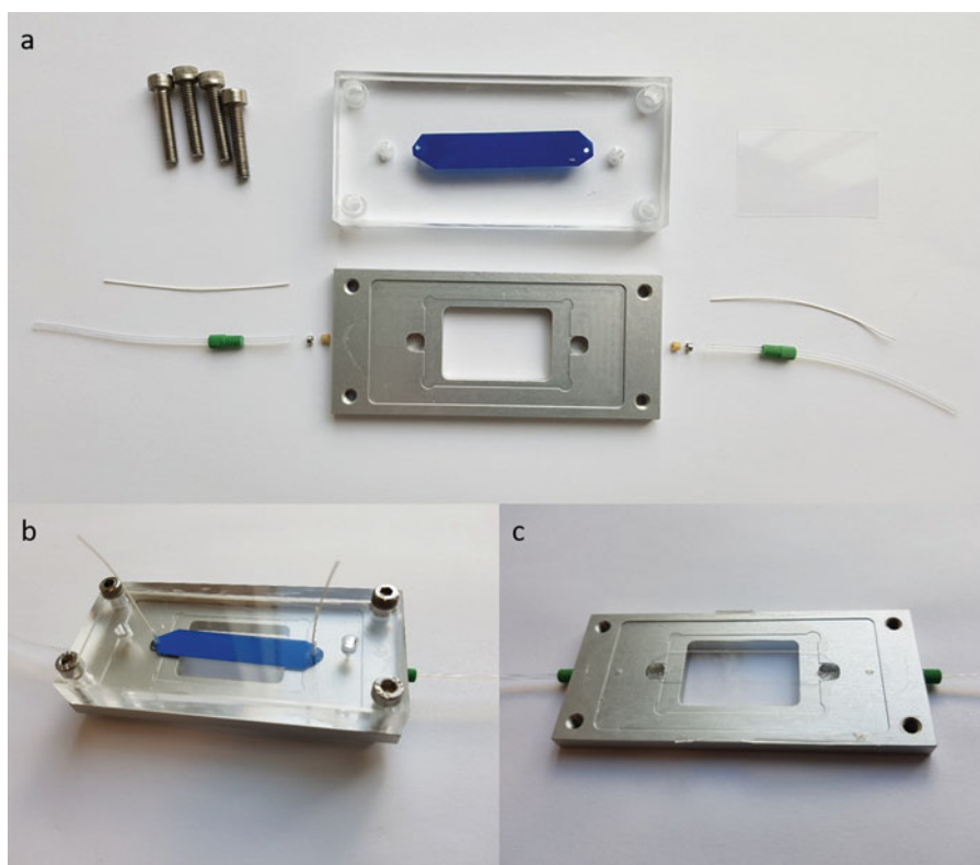
Fig. 1 The assembly of the custom-built flow cells is a three-step process. (a) Tubes and slides are assembled. The 24 \times 40 mm glass slide is placed in the designated cavity of the aluminum body. Electric wire is inserted into the FEP tubing and guided upward through the mold. (b) After mounting the Perspex mold, the assembled flow cell is ready for casting PDMS. (c) Once the PDMS is cured, the electric wire and mold can be removed and the flow cell is covered by a 24 \times 60 mm biochemically functionalized glass slide
