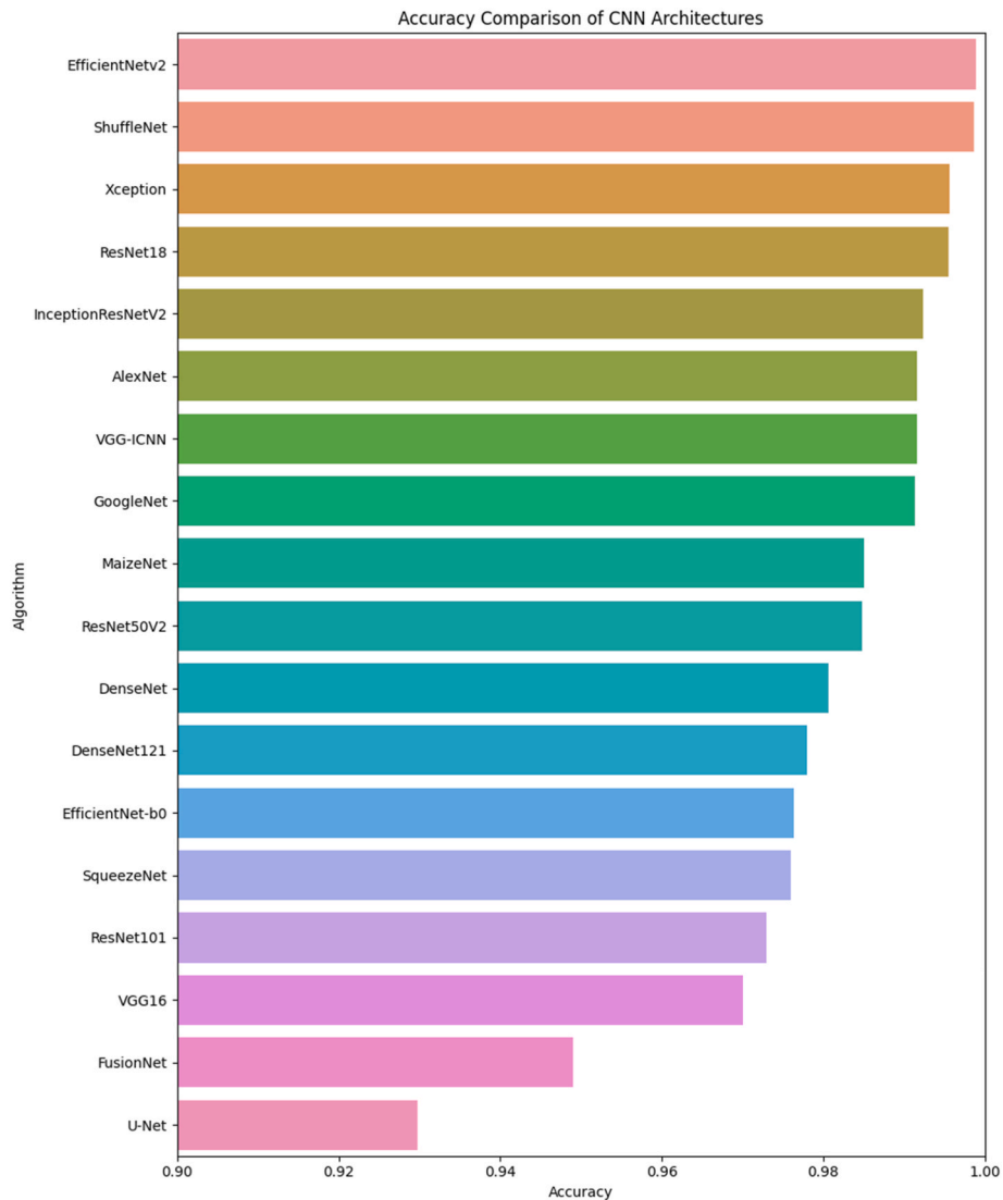
Fig. 2. Algorithm comparison.
