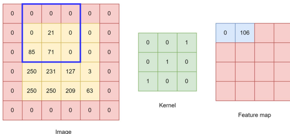
Fig. 5 Convolutional neural network sample (Cho and Kim 2021)
