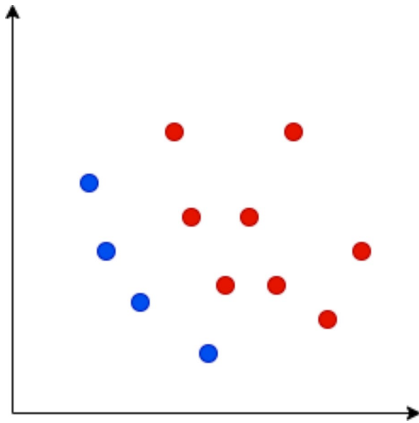
Fig. 3 The non-dominated solutions with blue color and the dominated solutions with red color
