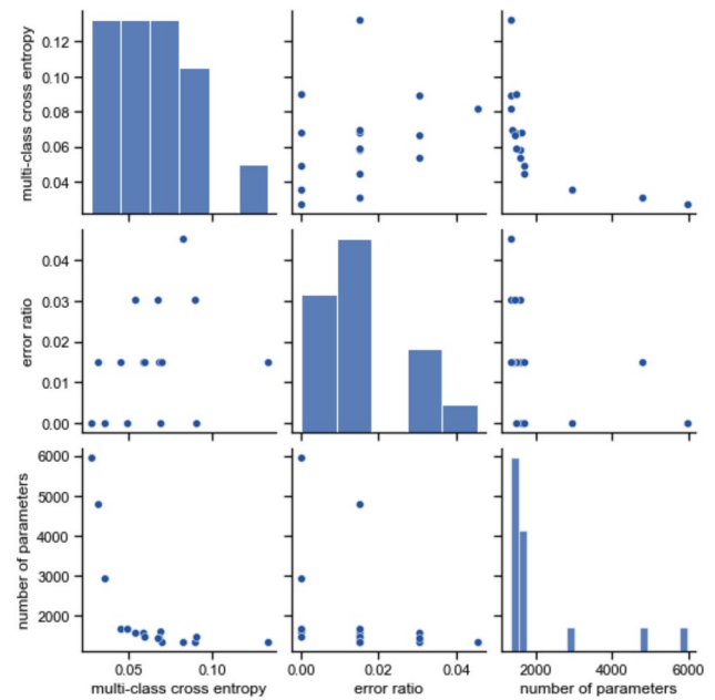
Fig. 12 Pareto front of NSGA-II
