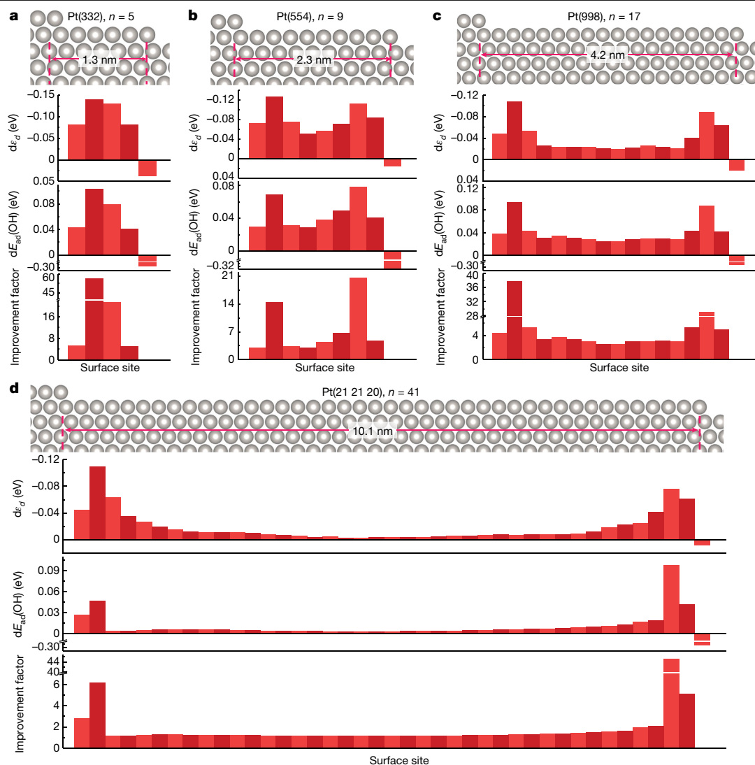
Fig. 2 | Atomic site-resolved electronic structure, surface reactivity and ORR activity of stepped Pt(111) surfaces. a–d, Side view (upper panels) and atomic site-resolved d -band centre shift ( d\epsilon_d ), OH adsorption energy shift
