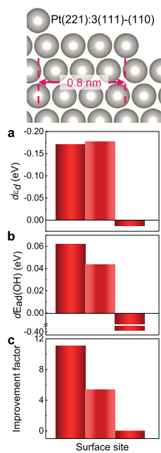
Extended Data Fig. 4 | Atomic site-resolved electronic structure, surface reactivity and ORR activity of Pt(221) with respect to that of Pt(111) surface. Shown are d -band centre shift d\epsilon_d (a), OH adsorption energy shift dE_{ad}(\text{OH}) (b), and ORR improvement factor (c). Surface sites correspond to atoms in the top layer of the side view (upper panel). The terrace width is indicated by double arrow lines.
