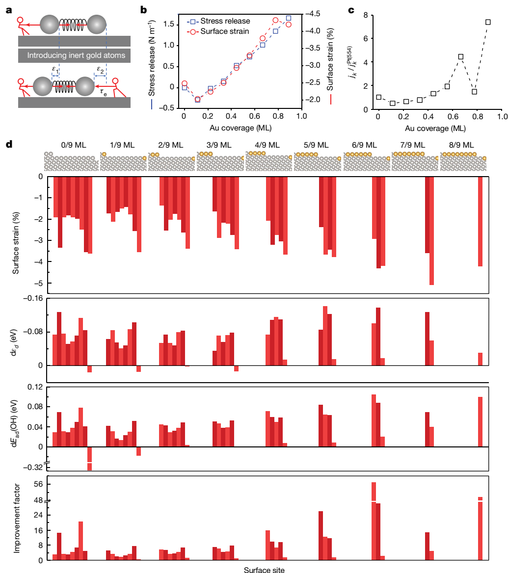
Fig. 3 | The response of residual surface stress, surface strain, surface electronic structure, surface reactivity and ORR activity with respect to external forces. a, Mechanism of generating extra compressive strain by releasing residual tensile surface stress through external compressive stress ( \tau_e ). b, Stress release and surface strain of Pt(554) with 0 ML to 8/9 ML of Au at the step edge. c, Predicted enhancement of ORR activity of Pt(554) with respect to the coverage of Au. To reduce the errors induced by reference states and at the
