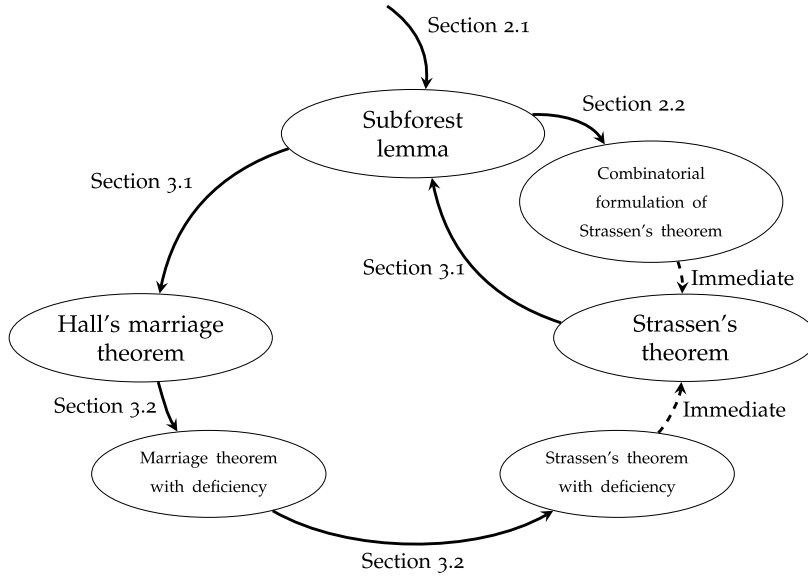
Fig. 1. A graphical outline of this paper, where the arrows represent the different proofs.
