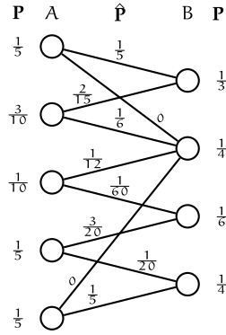
Fig. 2. A graphical representation of the setting of Theorem 1. The vertices represent the elements of sets A and B , and the edges represent the elements of R . The number next to a vertex denotes the mass that either \mathbf{P} or \mathbf{P}' assigns to that vertex. The numbers above the edges are the masses assigned by the coupling \hat{\mathbf{P}} , which is supported on a subset of R . By interpreting the masses of \mathbf{P} and \mathbf{P}' as vertex weights and the masses of \hat{\mathbf{P}} as edge weights, we find ourselves in the setting of Proposition 4.
