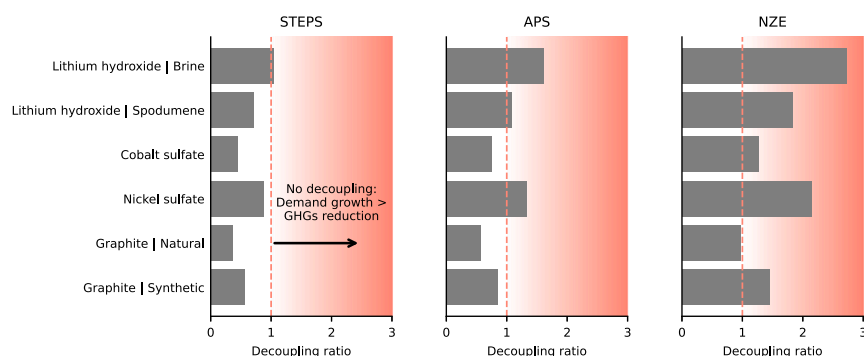
Figure 5. Decoupling ratio between EV's mineral demand by 2030 in the IEA's scenarios and the GHG emissions intensity of associated LIB raw materials considering the hypothetical decarbonization scenario
