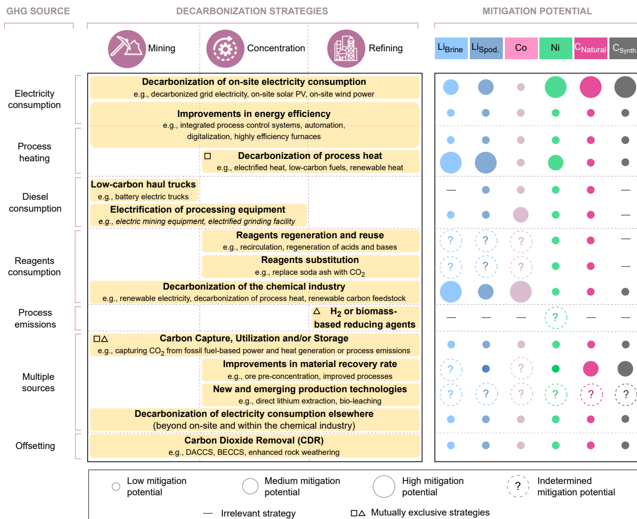
Figure 3. Strategies for reducing GHG emissions from battery-grade raw materials supply chain
