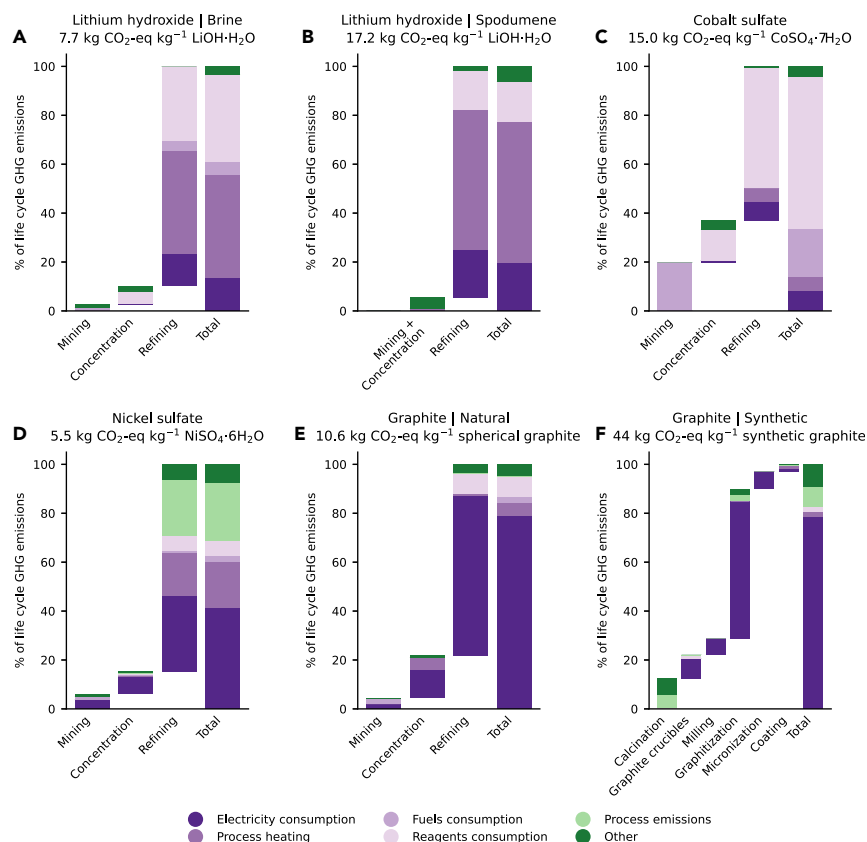
Figure 2. Breakdown of life cycle GHG emissions from the principal production routes for battery-grade raw materials
