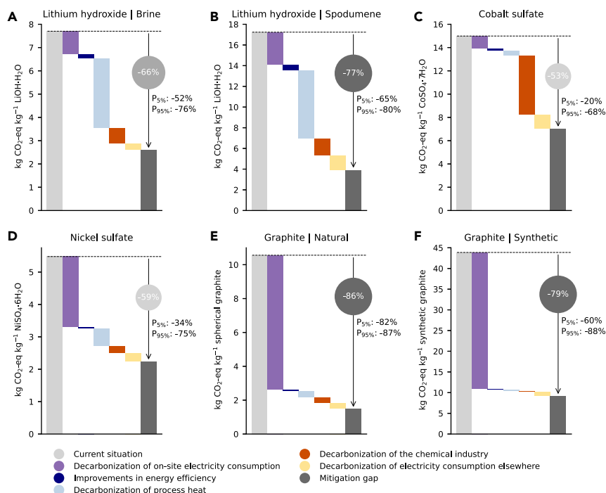
Figure 4. Mitigation potential of a decarbonization scenario for battery-grade raw materials involving the transition to renewable electricity and heat electrification across their supply chain “Decarbonization of on-site electricity consumption” is achieved by utilizing wind power paired with a BESS. “Improvements in energy efficiency” assumes a 5% reduction in overall energy consumption. “Decarbonization of process heat” is achieved through electrified heat powered by wind energy. Decarbonization of the chemical industry encompasses the use of wind power and electrified heat (also based on wind energy). Decarbonization of electricity consumption elsewhere entails transitioning to wind power for all remaining activities within the global economy. P 5% and P 95% indicate the 5 th –95 th percentiles from the Monte Carlo uncertainty analysis (full results are presented in Figure S3).
