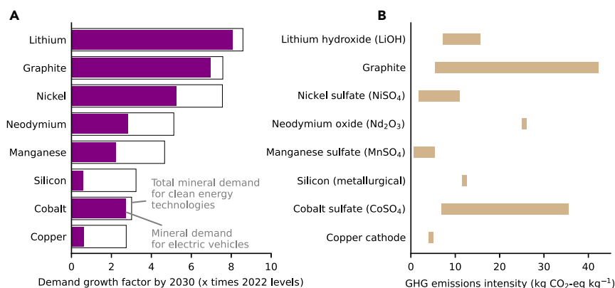
Figure 1. Minerals demand by 2030 in the IEA's Net-Zero Emissions scenario and GHG emissions intensities of associated commodities
