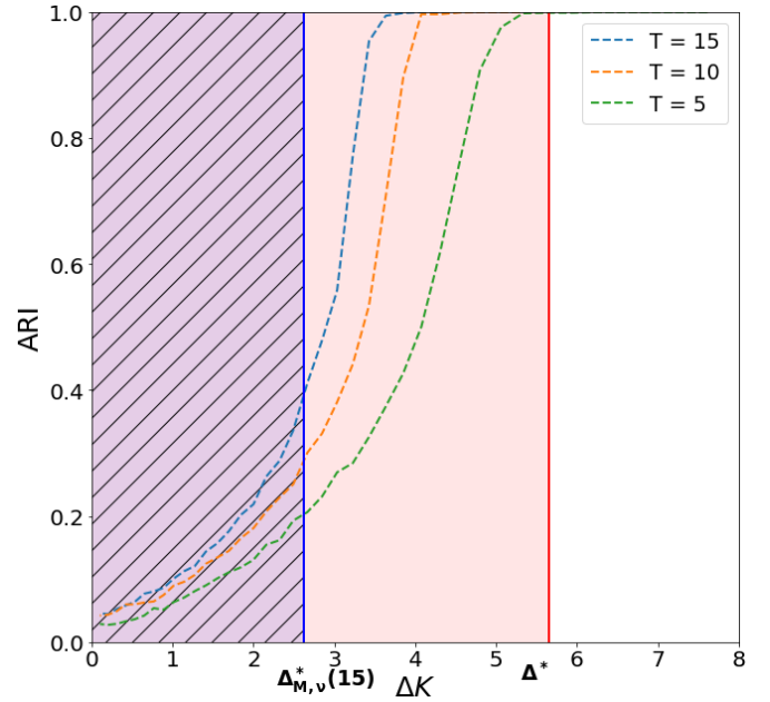
FIG. 4. This figure illustrates three different performance profiles of the modularity, as described in Eq. (15), for graph trajectories of varying lengths generated using the DSBM outlined in Sec. III B, for different values of \Delta k . The vertical blue line represents the DT for the temporal network with T = 15 , while the red vertical line indicates the DT for a single static snapshot. For each trajectory, we maintain \bar{k} = 8 , \bar{h} = 4 , two communities and N = 200 . Each point is the result of the average over 50 trajectories.
