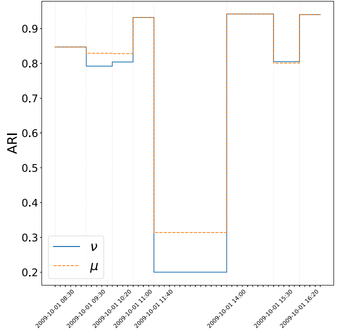
FIG. 6. The figure displays the ARI values across 10-min temporal windows at various identified breakpoints (red vertical lines). Each illustrated segment is proportional in length to the period during which the network can be considered stationary. Within this interval, the ARI value is fixed and calculated by comparing the detected communities to those presumed real. The figure showcases the results for two different types of modularity functions.
