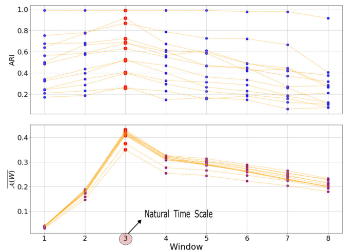
FIG. 10. Results from the numerical simulations described in Appendix 6. Each line is related to different initial values for \Delta k and \Delta h at the natural time scale, which is consistently 3 for all trajectories. Each network in the simulations comprises 200 nodes, 15 time steps, and five communities. Red dots represent the maximum for the given metric regarding the aggregation level.
