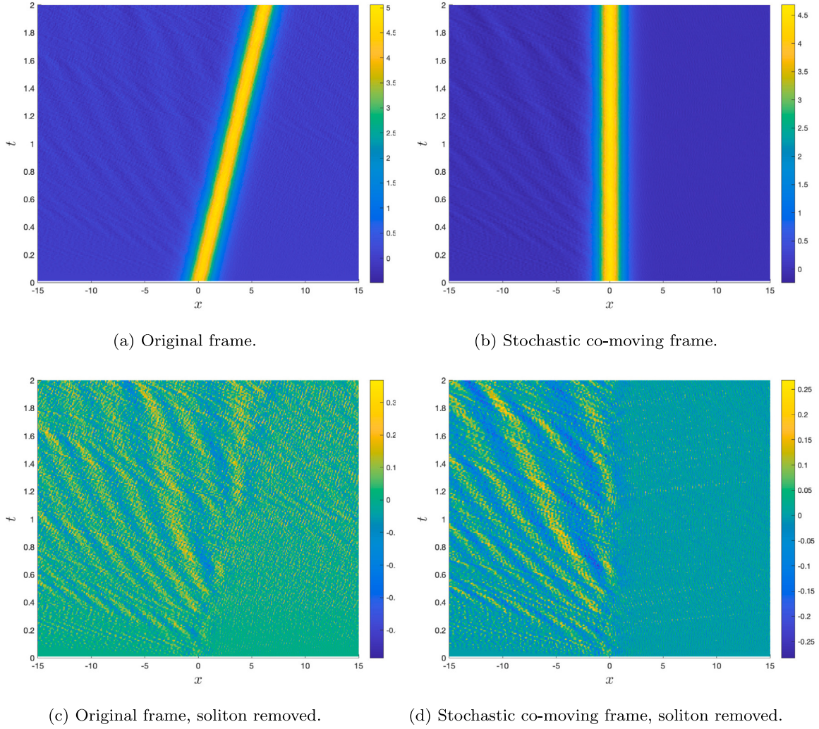
Fig. E.11. Simulation of the KdV equation with space-time white noise of strength \sigma = 0.05 . The original frame realization shows u(t, x) , from a simulation of (2.1). The frozen frame simulation shows \phi_c(x) + v(t, x) , from simulation of (2.30)–(2.32) with the same realization of the noise. Fig. E.11(c) and Fig. E.11(d) show the perturbation with respect to the soliton. The original frame realization shows u(t, x) - \phi_{c(t)}(x - \xi(t)) with the phase-definitions (2.55), and the frozen frame simulation shows v(t, x) .
