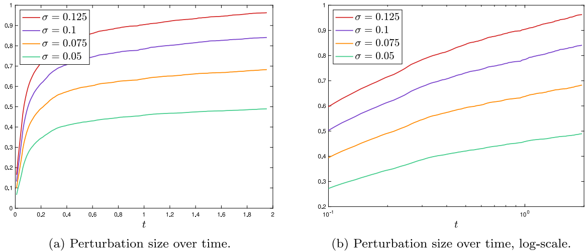
Fig. E.12. Sample mean of the process \sup_{s \leq t} \|v(s)\|_{L^2_x([-40, 10])} for space-time white noise, computed over 200 realizations for \sigma \in \{0.05, 0.075, 0.1, 0.125\} . This simulation was computed on the computational domain [-40, 40] , with values c_s = 3 and a = 0.15 .
