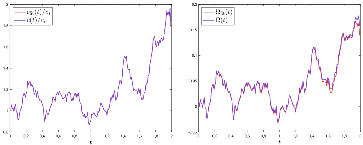
Fig. 2. Path-wise comparison of soliton amplitudes c(t) to c_{\text{fit}}(t) (left) and phase shifts \Omega(t) to \Omega_{\text{fit}}(t) (right) at noise strength \sigma = 0.25 and initial amplitude c_* = 3 . The parameters c_{\text{fit}}(t) and \Omega_{\text{fit}}(t) , defined in (2.55) and (2.56), are obtained from direct simulation in the original frame of (2.9). The soliton amplitude c(t) and phase shift \Omega(t) are obtained from simulation of the frozen frame system (2.33)–(2.35).
