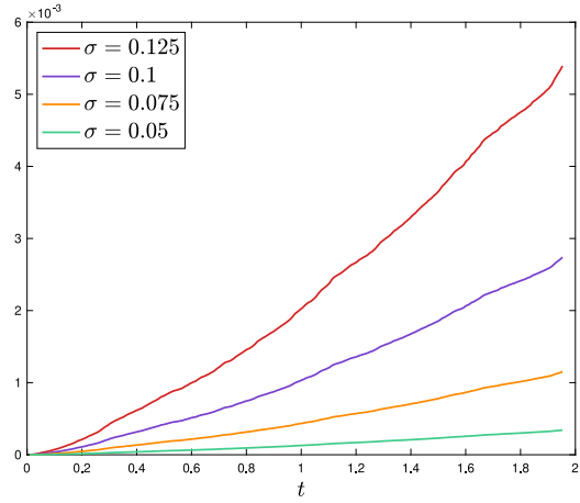
(b) Sample mean of \sup_{s \leq t} |c(s) - c_2(s)| .
