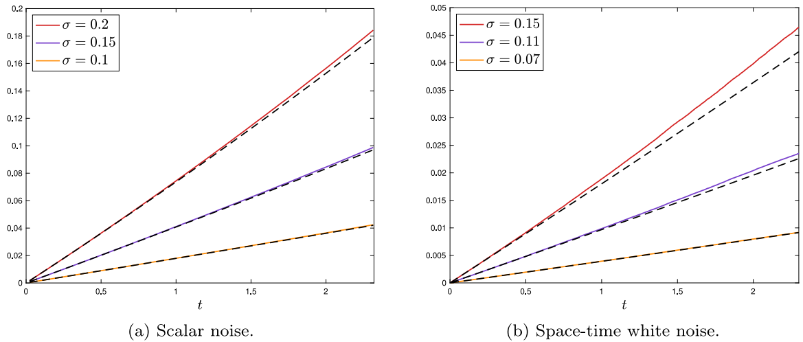
Fig. 5. Sample variance of the process c_{\text{fit}}(t)/c_* for scalar noise and space-time white noise at various noise strengths \sigma . Solid lines indicate the sample variance, dashed lines indicate the variance of c_0(t) as in (3.8) and (3.15), respectively. The sample variance is computed over 204 \cdot 10^4 and 8 \cdot 10^4 realizations, respectively.
