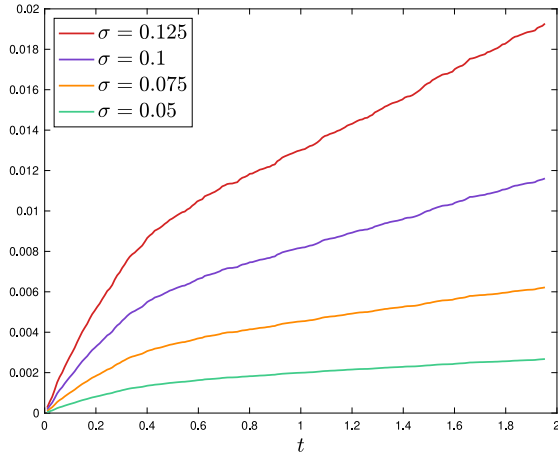
(a) Sample mean of \sup_{s \leq t} \|v(s) - v_1(s)\|_{L^2_a} .
