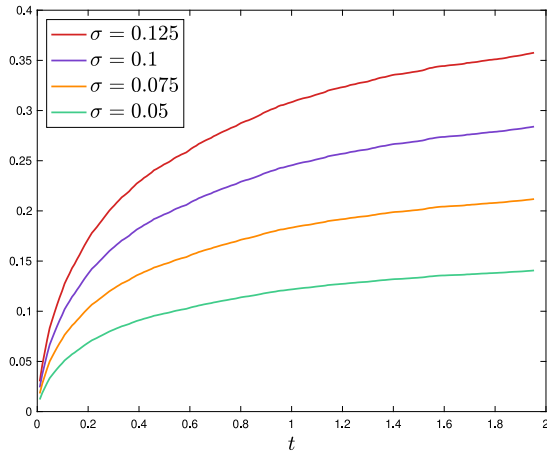
(a) Perturbation size over time.
