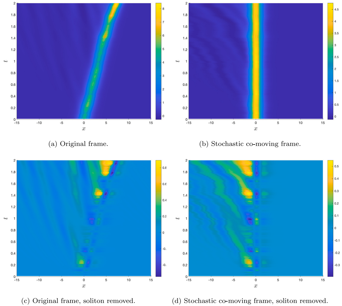
Fig. 1. Simulation of the KdV equation with scalar noise of strength \sigma = 0.25 . Panel (a) shows the original frame realization u(t, x) , from a simulation of (2.9). Panel (b) shows \phi_{c_*}(x) + v(t, x) , from simulation in the frozen frame of (2.33)–(2.35) with the same realization of the noise. Panels (c) and (d) show the perturbation with respect to the soliton, that is u(t, x) - \phi_{c(t)}(x - \xi(t)) with the phase-definitions (2.55) in panel (c), and v(t, x) in panel (d).
