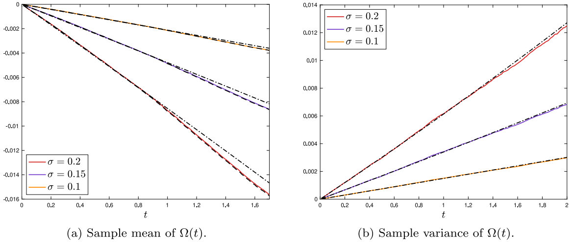
Fig. 7. Sample statistics of the process \Omega(t) for scalar noise. Computed over 3 \cdot 10^3 realizations for \sigma \in \{0.1, 0.15, 0.2\} . Dash-dotted lines indicate the theoretical mean and (leading-order) variance of \Omega_0(t) as in (3.10) and (3.11), respectively. Panel (a) also shows the sample mean of \Omega_2(t) (dotted), which gives significant improvement over the mean of \Omega_0(t) .
