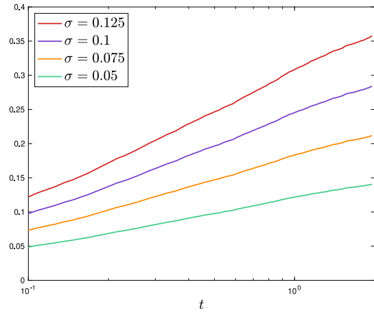
(b) Perturbation size over time, log-scale.
