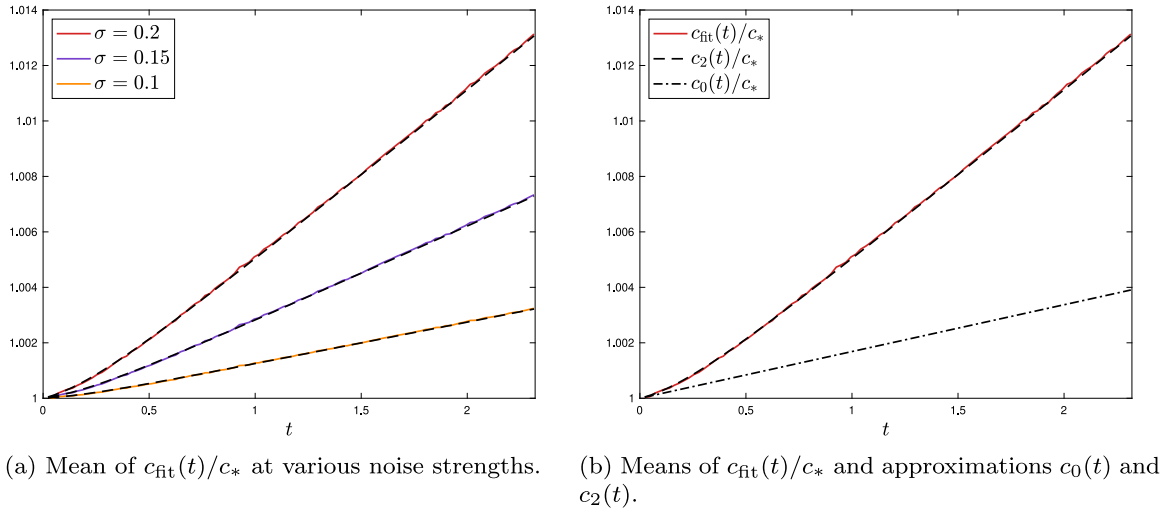
Fig. 6. Sample mean of the process c_{\text{fit}}(t)/c_* computed over 2 \cdot 10^4 realizations for scalar noise. The mean of c_2(t) (dashed) agrees well with that of c_{\text{fit}}(t) at the simulated noise strength values \sigma \in \{0.1, 0.15, 0.2\} , whereas the mean of c_0(t) (dash dot) as in (3.9) fails to capture the correct amplitude drift. The mean of c_1(t) provides no improvement, it cannot be distinguished from that of c_0(t) at these simulation values.
