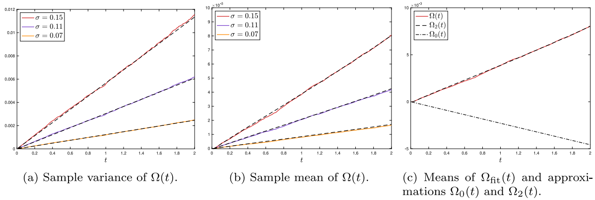
Fig. 10. Sample statistics (solid) of the process \Omega(t) for space-time white noise, at noise strengths \sigma \in \{0.07, 0.11, 0.15\} . Dashed lines indicate the theoretical variance of \Omega_0(t) as in (3.19) and the sample mean of \Omega_2(t) , respectively. The dash-dotted line in panel (c) shows the mean of \Omega_0(t) , see (3.18), which fails to capture the correct phase drift. The sample variance is computed over 2500 realizations and the sample mean over 10^4 realizations.
