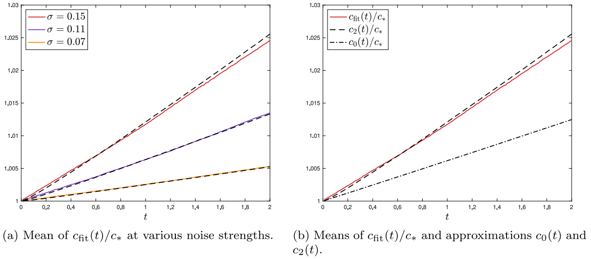
Fig. 9. Sample mean of the process c_{\text{fit}}(t)/c_* computed over 36 \cdot 10^3 realizations for space-time white noise. The mean of c_2(t) (dashed) agrees well with that of c_{\text{fit}}(t) at the simulated noise strength values \sigma \in \{0.07, 0.11, 0.15\} , whereas the mean of c_0(t) (dash dot) as in (3.9) fails to capture the correct amplitude drift. The mean of c_1(t) provides no improvement, it cannot be distinguished from that of c_0(t) at these simulation values.
