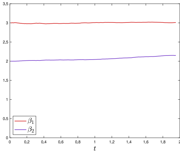
Fig. E.13. Estimation of the orders \beta_1 and \beta_2 at which the remainders |c - c_2| and \|v(t) - v_1(t)\|_{L^2_\sigma} depend on the noise strength \sigma . Here, \beta_1(t) is obtained from a least squares fit of \mathbb{E} \sup_{s \leq t} |c(s) - c_2(s)| (as in Fig. 8) to k_1(t)\sigma^{\beta_1(t)} . Similarly, the exponent \beta_2(t) is obtained from a least squares fit of \mathbb{E} \sup_{s \leq t} \|v(s) - v_1(s)\|_{L^2_\sigma} to k_2(t)\sigma^{\beta_2(t)} .
