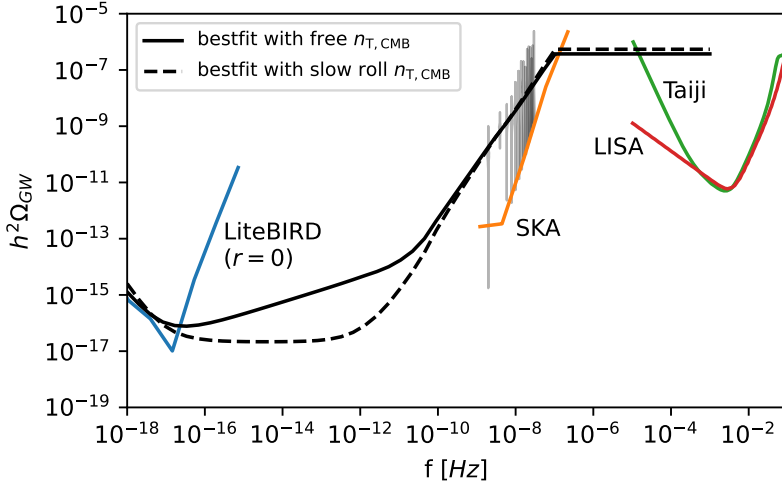
Figure 3. The bestfit energy spectrum \Omega_{GW}(f) of IGWB with n_T^{\text{CMB}} free and n_T^{\text{CMB}} = -r/8 , respectively. We also show the sensitivity curves for LiteBIRD, SKA (Square Kilometre Array), space-based laser interferometers: LISA and Taiji. Here, we use the transfer function showed in ref. [73], which can return to eq. (2.1) at the high frequency limit, see also refs. [61, 74–77]. As commented in section 4, when f > 10^{-7} the highly-blue ( n_T^{\text{PTA}} \simeq 2 ) tilt needs to be cut off, though we plot \Omega_{GW}(f > 10^{-7}) with a straight line, which but is actually model-dependent, e.g. [62, 63].
