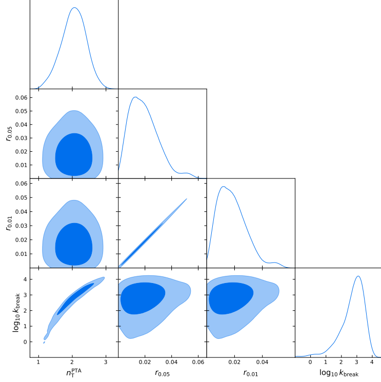
Figure 2. Marginalized posterior distributions of the parameters in the broken power-law model (1.2) with slow-roll n_{\text{T,CMB}} .
