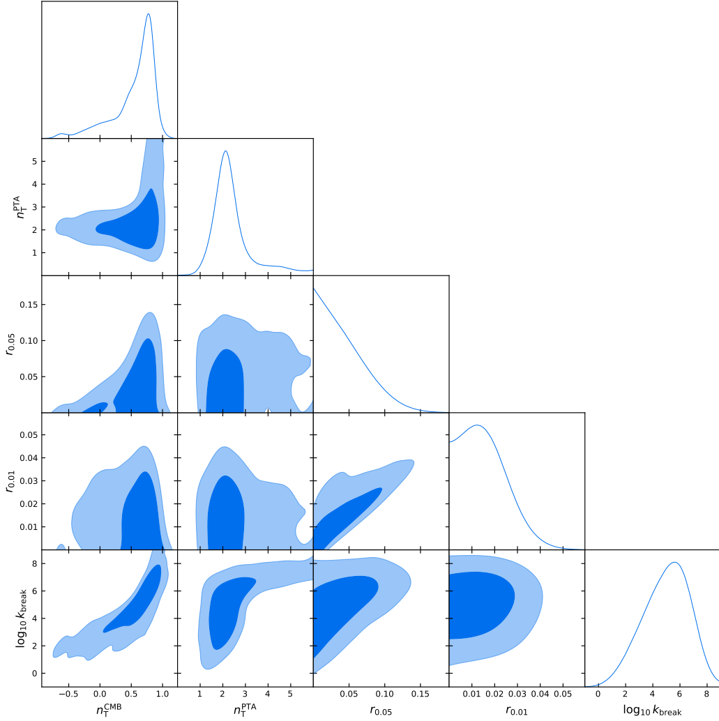
Figure 1. Marginalized posterior distributions of the parameters in the broken power-law model (1.2) of IGW with n_{T,CMB} free.
