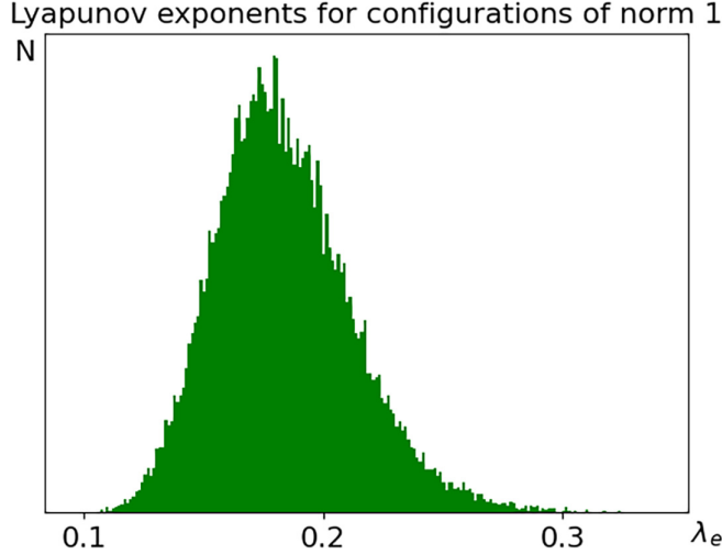
FIG. 2. Histogram of Lyapunov exponents for an SU(4) chaotic AB decomposition. The histogram of distribution of Lyapunov exponents for configurations \mathbf{x}_0 with ||\mathbf{x}_0|| = 1 . Twenty-five thousand random configurations are sampled.
