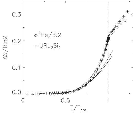
FIG. 2. The measured entropy for \text{URu}_2\text{Si}_2 [10] (with the value at T = 2 K subtracted to eliminate the superconducting transition) and ^4\text{He} [28]. A vertical scale factor of 5.2 has been applied to the helium data, and the results have been plotted versus reduced temperature. The dashed-dotted line is the predicted entropy for ^4\text{He} using the T = 0 K dispersion for the calculation, the solid curve (largely coinciding with the dashed curve) is the same for \text{URu}_2\text{Si}_2 using the dispersion from Ref. [7].
