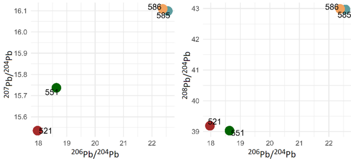
Fig. 5. The lead isotope compositions of four samples.
