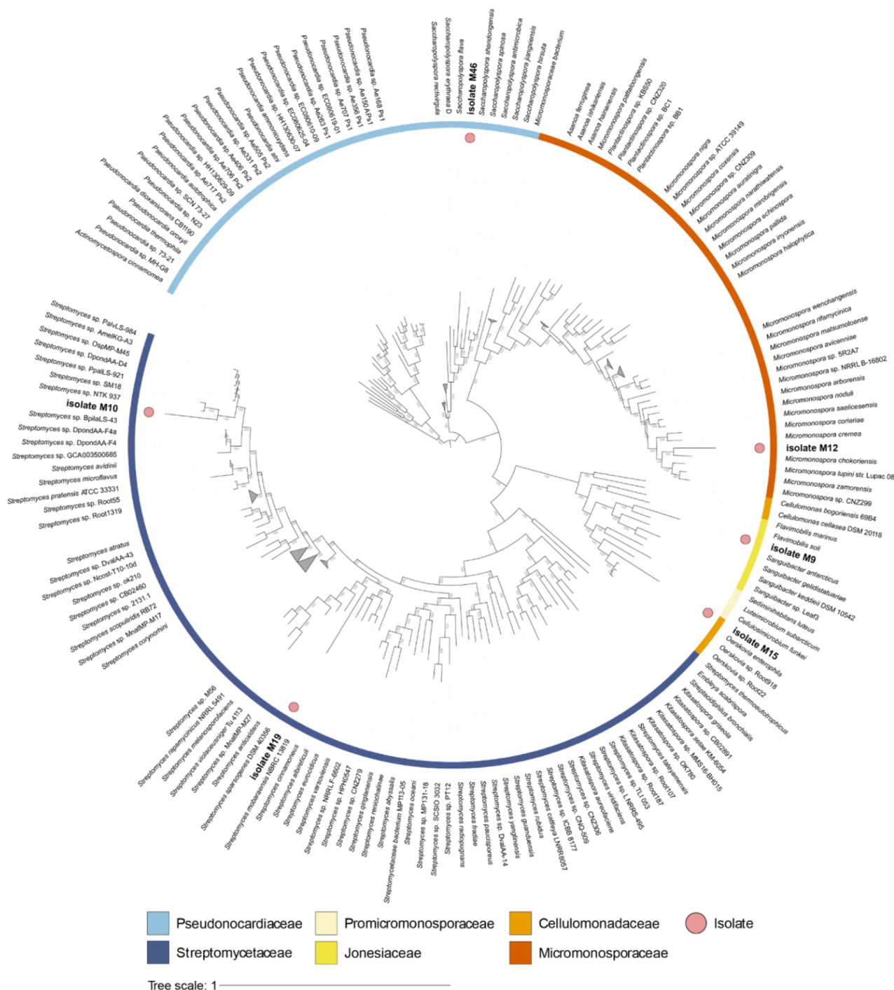
FIGURE 1 Phylogeny of whole-genome sequences of mammoth isolates and their closest known relatives. PhyloPhlAn-based maximum-likelihood tree of the six isolates compared to 578 Actinomycetota of six bacterial families (colour-coded in the outer ring), subdivided into 40 genera. The tree was rooted using Pseudonocardia sp. as outgroup and the numbers on the tree branches represent the bootstrap values in percentages of a total of 1000 bootstraps. Circles indicate the location of the novel isolates. The phylogenetic analysis suggests the following likely classification based on their nearest neighbours: M9, Sanguibacter ; M12, Micromonospora ; M15, Oerskovia ; M10 & M19, Streptomyces ; M46, Saccharopolyspora .
