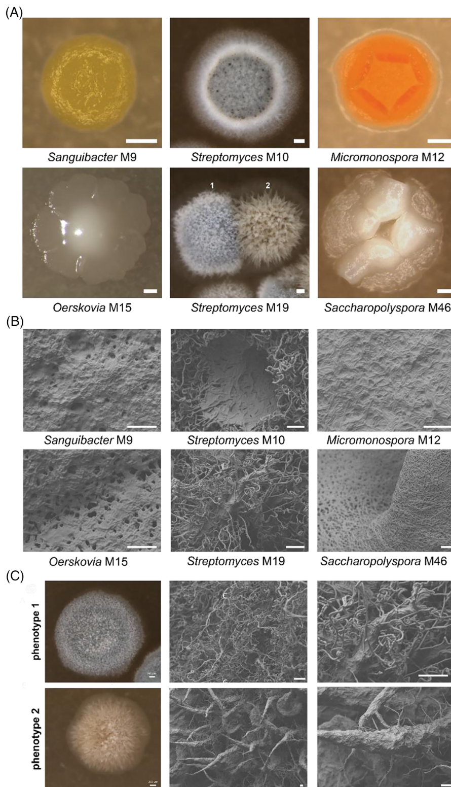
FIGURE 2 Phenotypic characterisation of Actinomycetota isolated from a faecal sample of a 28,000-year-old mammoth. Strains were grown on soya flour medium (SFM) agar plates for 9 days. (A) Stereomicrographs of isolates Sanguibacter sp. M9, Streptomyces sp. M10, Micromonospora sp. M12, Oerskovia sp. M15, Streptomyces sp. M19 and Saccharopolyspora sp. M46 (for phylogenetic analysis see Figure 1). Streptomyces sp. M19 showed two distinct phenotypes: fully developed colonies (1) and colonies with a bald appearance (2). Scale bar: 200 \mu m. (B) Scanning electron micrographs of isolates M9, M10, M12, M15, M19 and M46. Scale bar: 10 \mu m. (C) Scanning electron micrographs showing significant differences in morphology between the two colony phenotypes observed when Streptomyces sp. M19 is grown on SFM. Images of phenotype 1 show spirals of spore chains. Images of phenotype 2 show large spikes made up of hyphae and extracellular matrix. Also in the fully developed colony, such spikes can be found but in low frequency. The 16S rRNA sequencing strongly suggests that these morphological variants are phenotypes of Streptomyces sp. M19. Scale bar: 10 \mu m.
