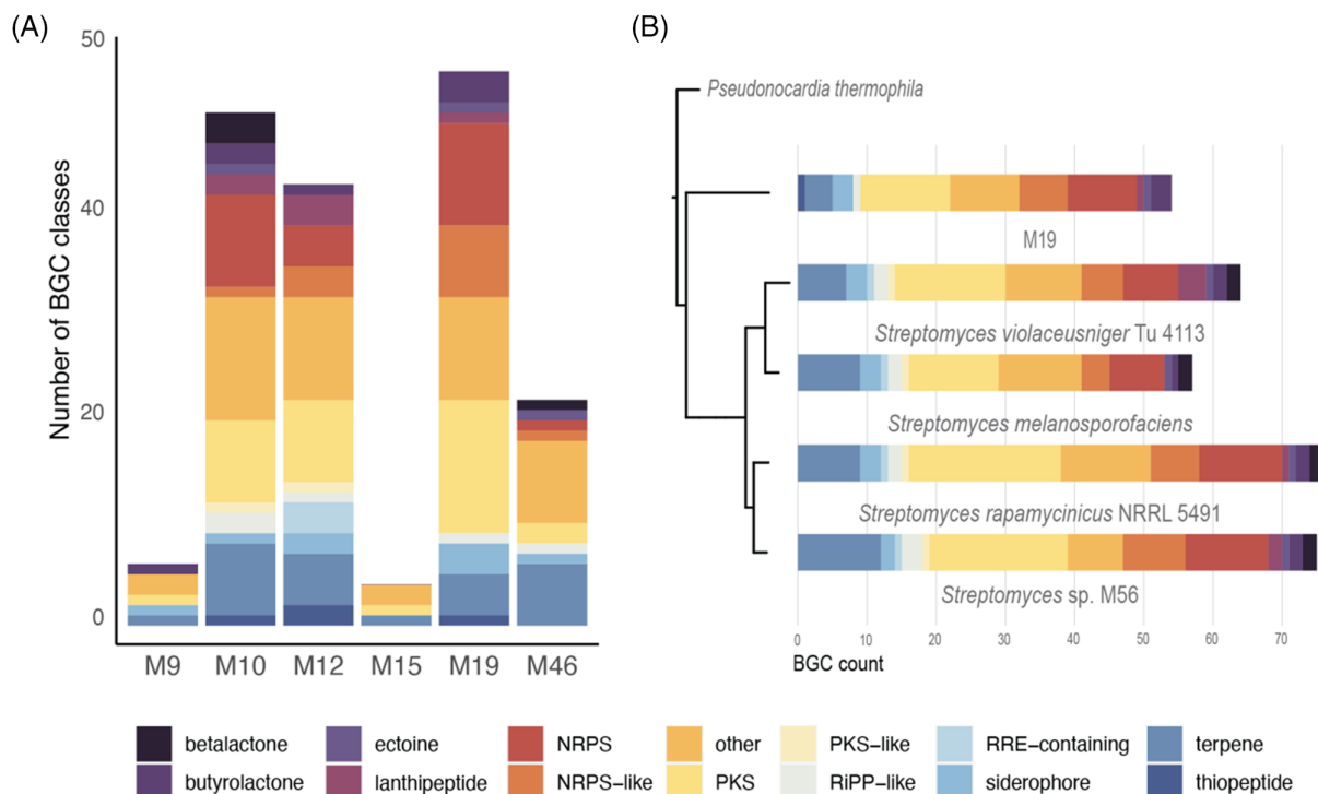
FIGURE 3 Classification of biosynthetic gene clusters (BGCs) predicted in the Actinomycetota genomes. (A) BGC classes for each isolate predicted with antiSMASH v6.0. Known types of BGCs representing <1% of all BGCs were grouped into the “other” category. The large number of BGCs in Streptomyces spp. M10 and M19, Micromonospora sp. M12 and Saccharopolyspora sp. M46 is particularly noteworthy. (B) Overview of all predicted BGC classes for isolate M19 and its closest neighbours Streptomyces violaceusniger Tu 4113, Streptomyces rapamycinicus NRRL 5491, Streptomyces sp. M56 and Streptomyces melanosporofaciens . The comparison shows that only two BGCs are shared between all three isolates, namely BGCs for desferrioxamine and for ectoine. Moreover, the genome of Streptomyces sp. M19 contains a greater variety of BGC classes, with a surprisingly high proportion of non-ribosomal peptide synthetases (NRPS) BGCs. PKS, polyketide synthases. RiPPs, ribosomally synthesized and post-translationally modified peptides. RRE, RiPP recognition element.
