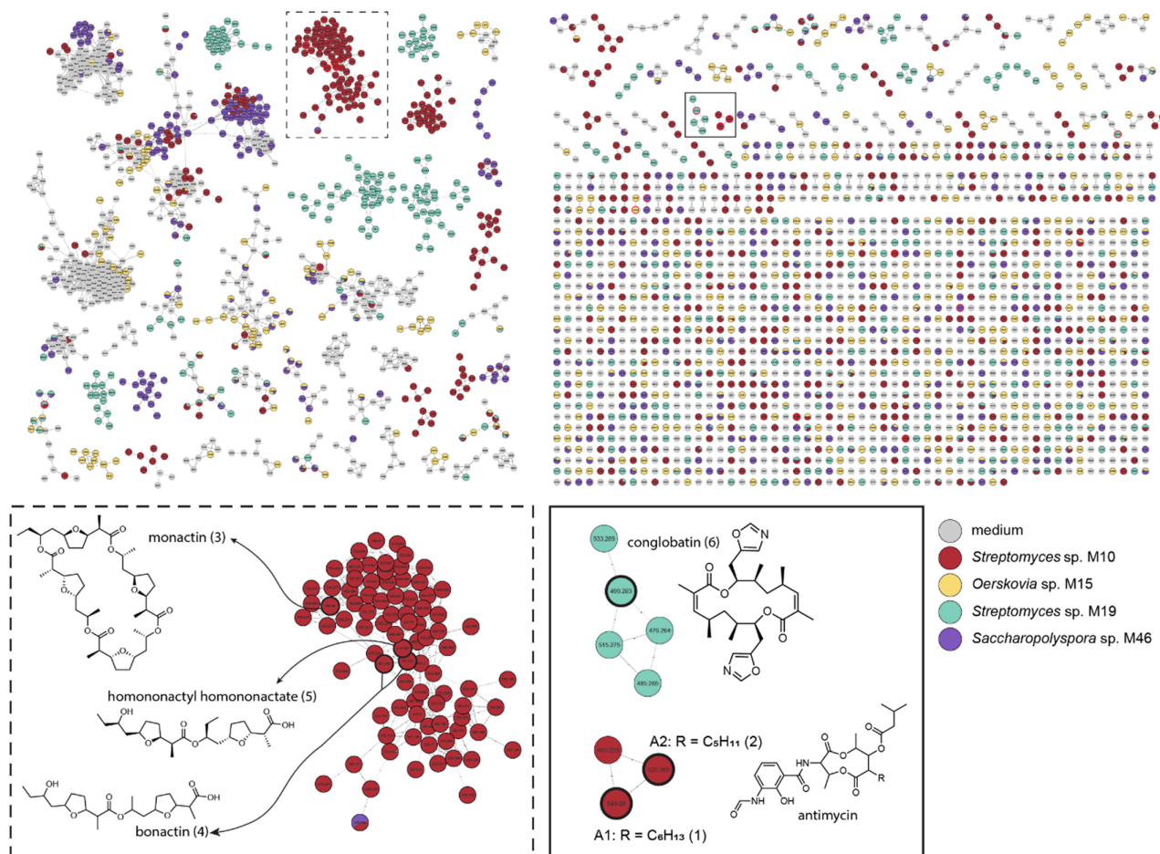
FIGURE 5 Molecular network of the ions detected in the crude extracts of the isolates and dereplication of bioactive compounds. A pie chart was mapped to the nodes which represents the abundance of each m/z value in the crude extracts of the different bioactive isolates (M10, M15, M19 and M46). Grey nodes indicate mass features that were also present in the medium blank. Nodes highlighted represent dereplicated known bioactive metabolites. Annotation was confirmed by manually checking the fragmentation data and the presence of the responsible biosynthetic gene clusters in the genome. The isolates were grown for 7 days on nutrient agar agar plates ( n = 3 ).
