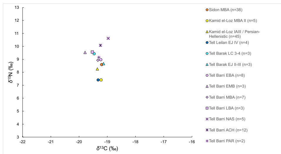
Fig. 8 Scatter plot of the mean \delta^{13}\text{C} and \delta^{15}\text{N} values of adults from North Syria Tell Brak (LC = Late Chalcolithic, c. 3900–3300 cal BCE, EJ II-III = Early Jezireh II-III = EBA, c. 3000–2000 cal BCE), Tell Barri (EBA = c. 2800–2200 BCE, EMB = Early/Middle Bronze Age, c. 2200–2000 BCE, MBA = c. 2000–1500 BCE, LBA = c. 1500–1200 BCE, NAS = Neo-Assyrian Period, c. 900–800 BCE,
