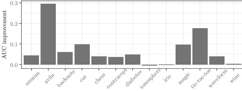
Fig. 3. Improvement in AUC by enabling the surrogate score for TURS.
