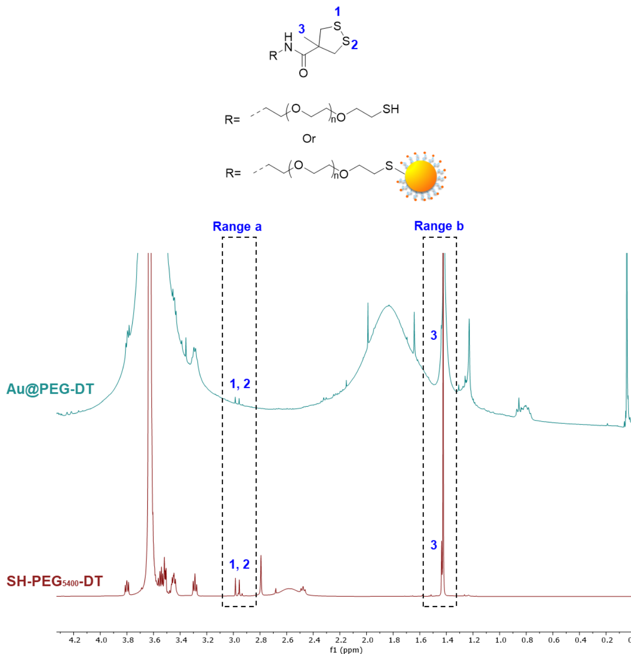
Figure S2. ^1\text{H-NMR} (400 Hz, 298K, \text{CDCl}_3 ) comparison spectrum of Au@PEG-DT (blue) and SH-PEG 5400 -DT (red).
