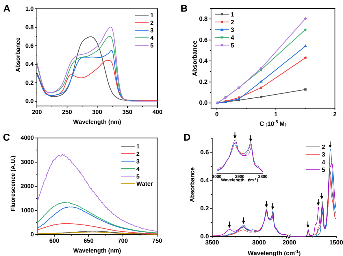
Figure 2. Spectroscopic studies of tripodal squaramide-based molecules: (A) UV-Vis spectra of 1-5 (15 \mu\text{M} ) in water. (B) Concentration varied UV absorbance of 1-5 plotted at 322nm. (C) Fluorescence spectra (15 \mu\text{M} ) of Nile Red dye embedded tripodal molecules 1-5 : ( C_{\text{NileRed}}=0.005 mg/mL, \lambda_{\text{exc}} = 550 nm., \lambda_{\text{em}} = 560\text{-}750 nm), Nile red in water is used as a control. (D) FTIR spectra of 2-5 in the solid state (samples lyophilized from water (5 mM), arrows highlight peaks considered).
