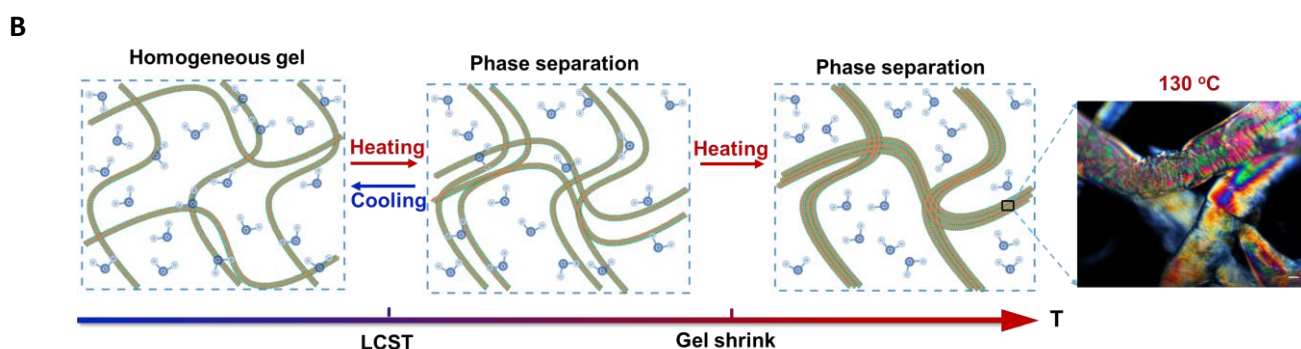
Scheme 1. (A) Squaramide-based tripodal supramolecular monomers 1-5 used in this study, and their self-assembly into supramolecular polymers and gel-phase materials. (B) Schematic of thermal transitions in the supramolecular network of 4 with increasing temperature.
