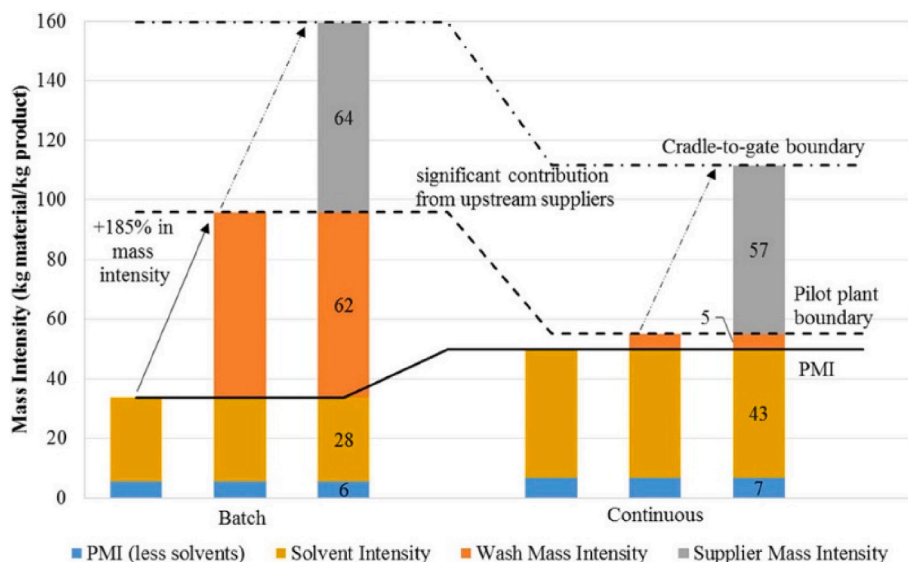
Fig. 4. LCA results of BP and CP on the synthesis of 4-DEL, focusing on the mass intensity, indicating that CP can observably reduce the environmental burden compared to BP. Adapted with permission from Lee et al. Copyright 2016 ACS Publications.
