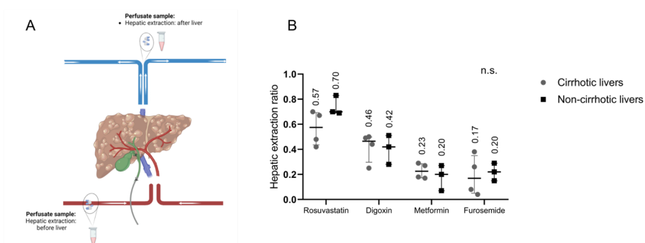
Figure 4.5 - Hepatic extraction of drug cocktail compounds. (a) Schematic representation of sample points before and after liver (b) hepatic extraction ratio of rosuvastatin, digoxin, metformin, and furosemide ( n=3 noncirrhotic livers and n=4 cirrhotic livers). Differences between groups were analyzed using the Mann-Whitney U test; P value is presented in the right corner of each graph. n.s., not significant.
