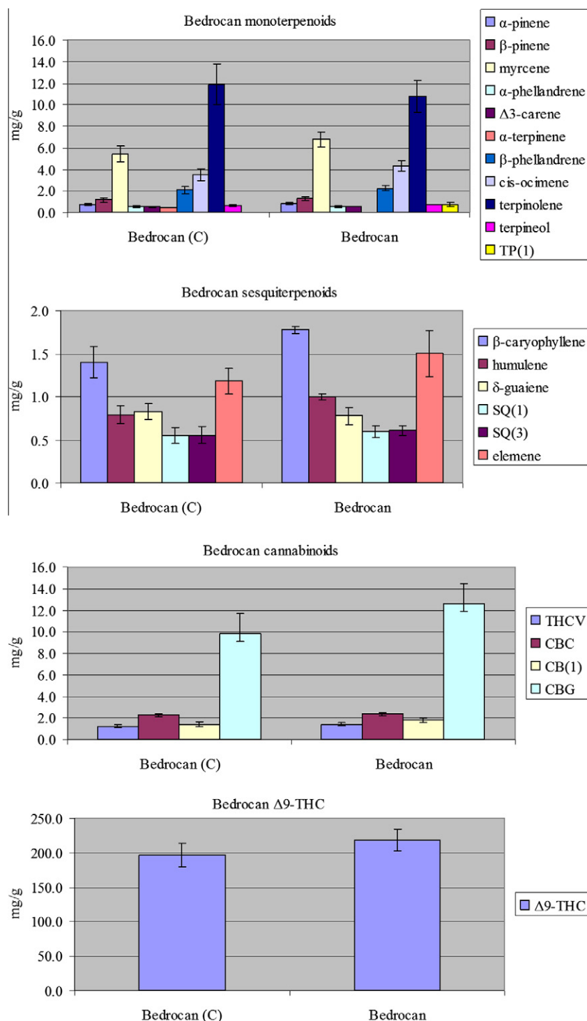
Fig. 10. Comparison of Bedrocan batches. Compounds that are missing in certain batches were present at levels <LOQ.
