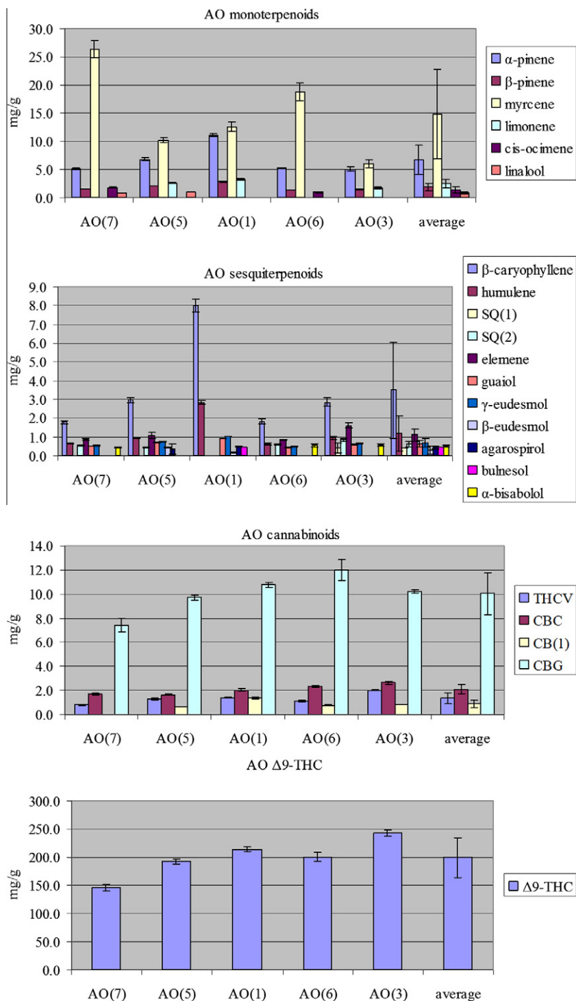
Fig. 11. Comparison of AO seed batches. Compounds that are missing in certain batches were present at levels <LOQ.
