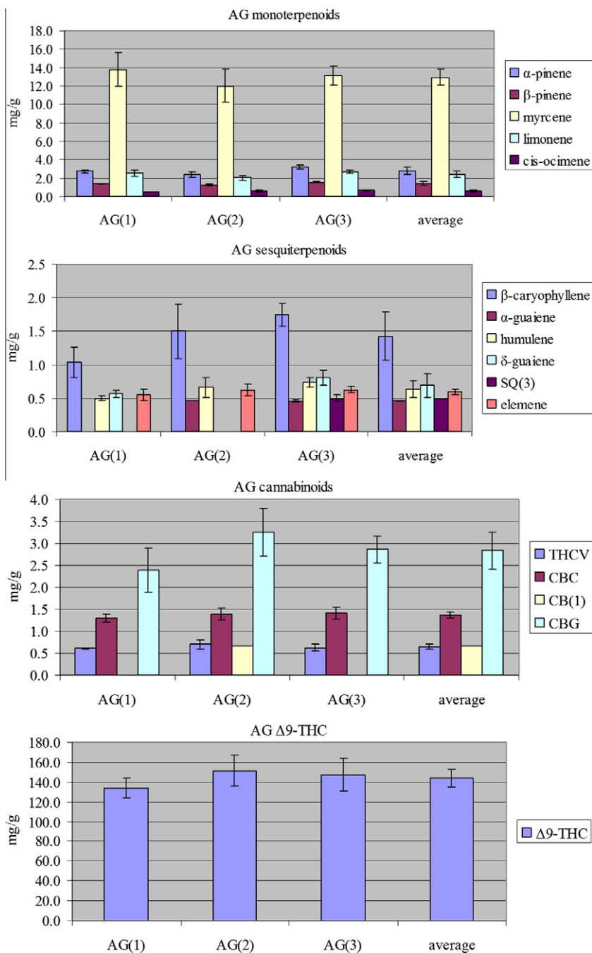
Fig. 6. Comparison of AG batches. Compounds that are missing in certain batches were present at levels <LOQ.
