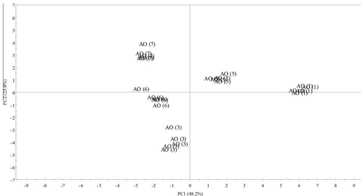
Fig. 12. PCA loading plot PC1 versus PC2 of AO seed batches.
