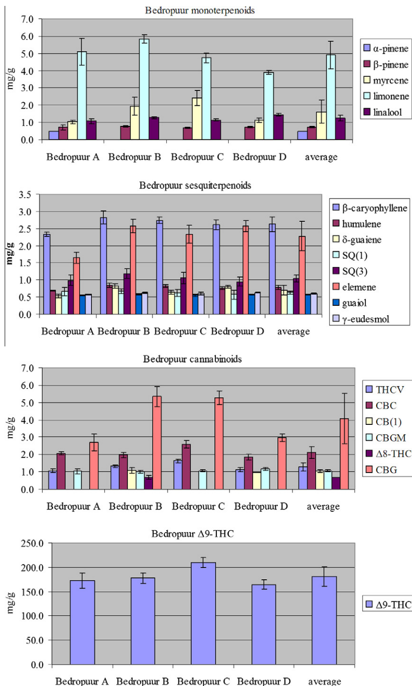
Fig. 9. Comparison of Bedropuur batches. Compounds that are missing in certain batches were present at levels <LOQ.
