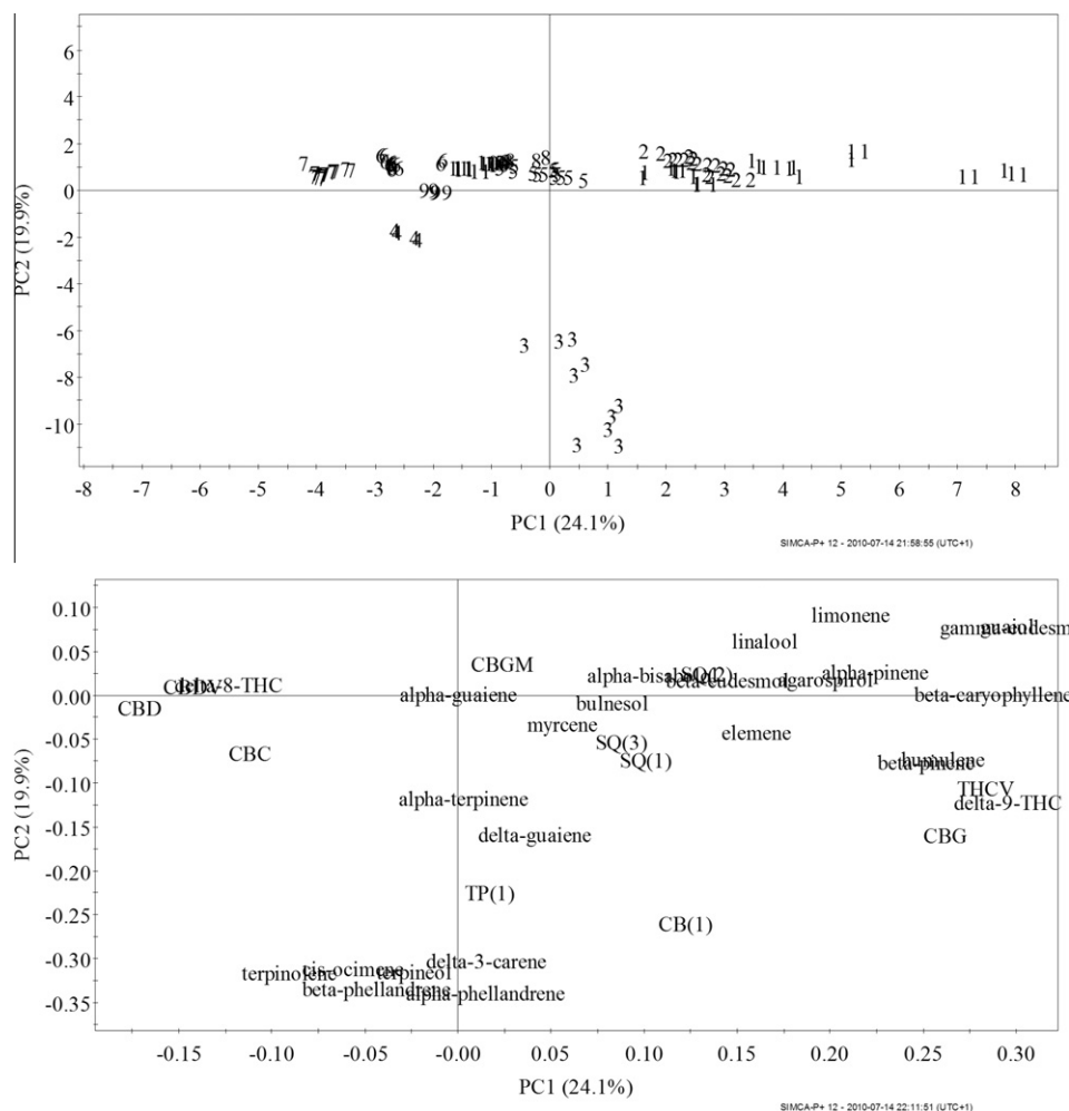
Fig. 2. PCA of all cannabis varieties. PC1 versus PC2, scatter plot (top) and loading plot (bottom). (1) AO, (2) Bedropuur, (3) Bedrocan, (4) Bediol, (5) AG, (6) AE, (7) Ai94, (8) AN, (9) AF, (10) AM, and (11) AD.
