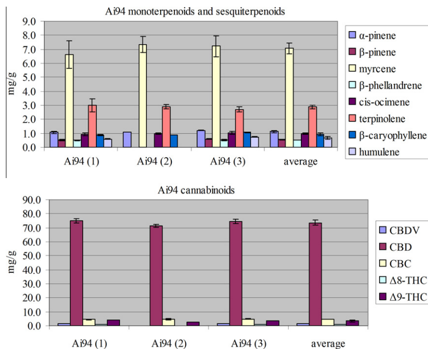
Fig. 8. Comparison of Ai94 batches. Compounds that are missing in certain batches were present at levels <LOQ.
