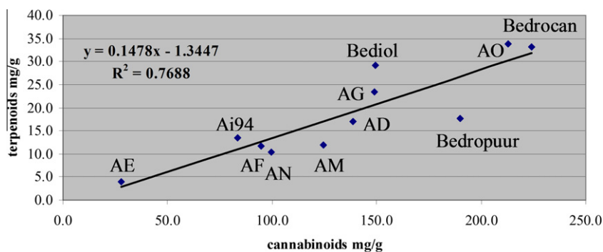
Fig. 1. Correlation of cannabinoid versus terpene levels.
