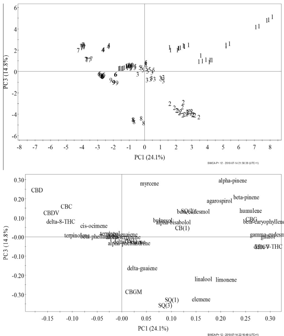
Fig. 3. PCA of all cannabis varieties. PC1 versus PC3, scatter plot (top) and loading plot (bottom). (1) AO, (2) Bedropuur, (3) Bedrocan, (4) Bediol, (5) AG, (6) AE, (7) Ai94, (8) AN, (9) AF, (10) AM, and (11) AD.
