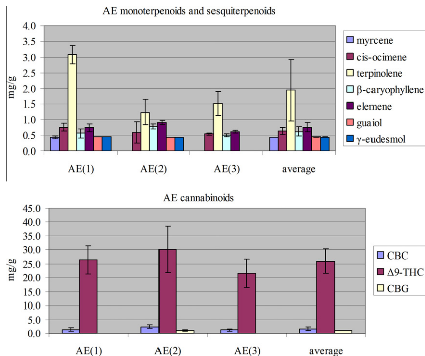
Fig. 7. Comparison of AE batches. Compounds that are missing in certain batches were present at levels <LOQ.
