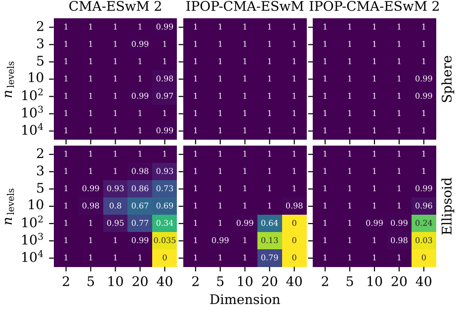
Figure 5.6: Success rates for CMA-ESwM with a doubled default population size (CMA-ESwM 2), CMA-ESwM with an IPOP restart strategy (IPOP-CMA-ESwM) and CMA-ESwM with an IPOP restart strategy and a doubled default population size (IPOP-CMA-ESwM 2) on the sphere function (top row) and ellipsoid function (bottom row), across various dimensions (x-axis) and discretization levels n_{\text{levels}} (y-axis). Each algorithm is given a budget of 2000 evaluations per dimension, with 200 runs conducted for each setting. The target function value is set to 10^{-8} .
