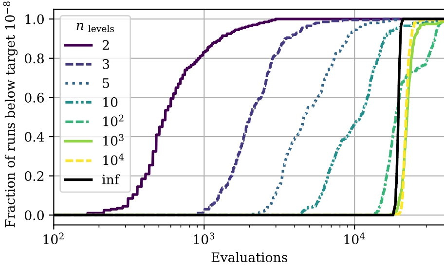
Figure 5.8: Empirical Cumulative Distribution Function for the IPOP-CMA-ESwM with a doubled default population size on the 20 dimensional ellipsoid function for n_{\text{levels}} \in \{2, 3, 5, 10, 10^2, 10^3, 10^4\} and the standard CMA-ES for n_{\text{levels}} \in \{\text{inf}\} . The target function value is set to 10^{-8} and 200 runs are conducted for each setting.
