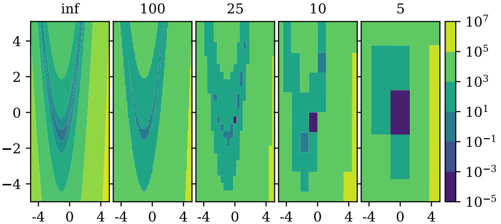
Figure 5.2: Discretized two-dimensional Rosenbrock function f(\mathbf{x}) , with \mathbf{x} \in [-5, 5]^2 for the different numbers of levels n_{\text{levels}} \in \{\text{inf}, 100, 25, 10, 5\} . Several local optima can be created due to the discretization, clearly observable for n_{\text{levels}} = 25 .
