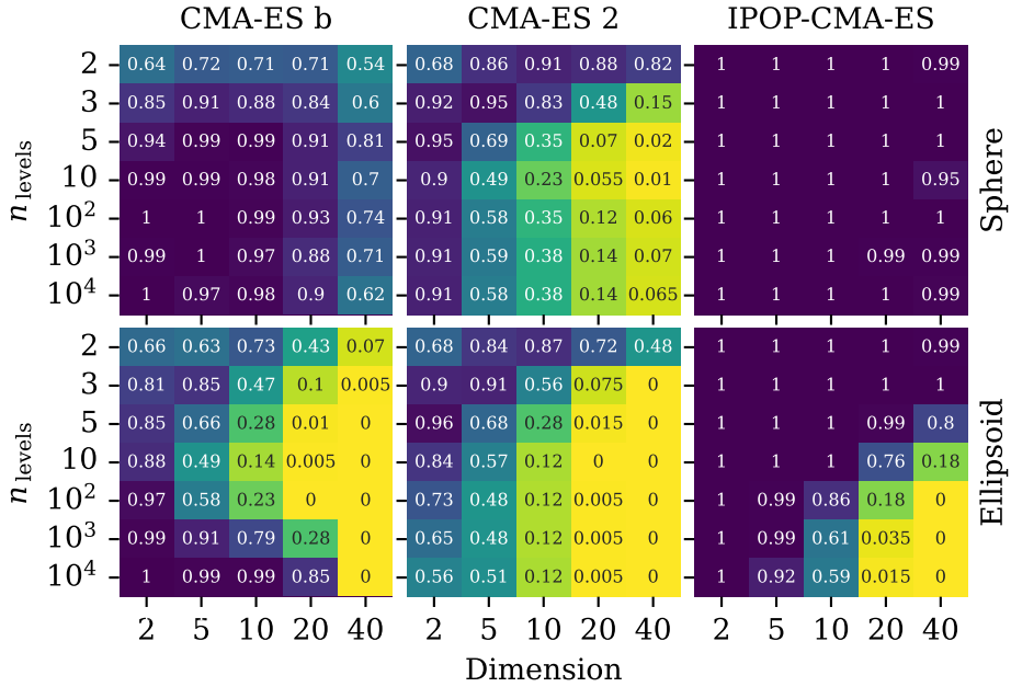
Figure 5.5: Success rates for CMA-ES with box-constraint handling (CMA-ES b), CMA-ES with a doubled default population size (CMA-ES 2) and CMA-ES with an IPOP restart strategy (IPOP-CMA-ES) on the sphere function (top row) and ellipsoid function (bottom row), across various dimensions (x-axis) and discretization levels n_{\text{levels}} (y-axis). Each algorithm is given a budget of 2000 evaluations per dimension, with 200 runs conducted for each setting. The target function value is set to 10^{-8} .
