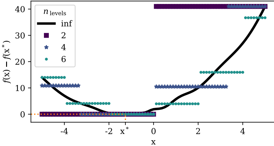
Figure 5.1: Discretized one-dimensional ellipsoid function f(\mathbf{x}) , with \mathbf{x} \in [-5, 5] for the different numbers of levels n_{\text{levels}} \in \{\text{inf}, 2, 4, 6\} with the global optimum at \mathbf{x}^* .
