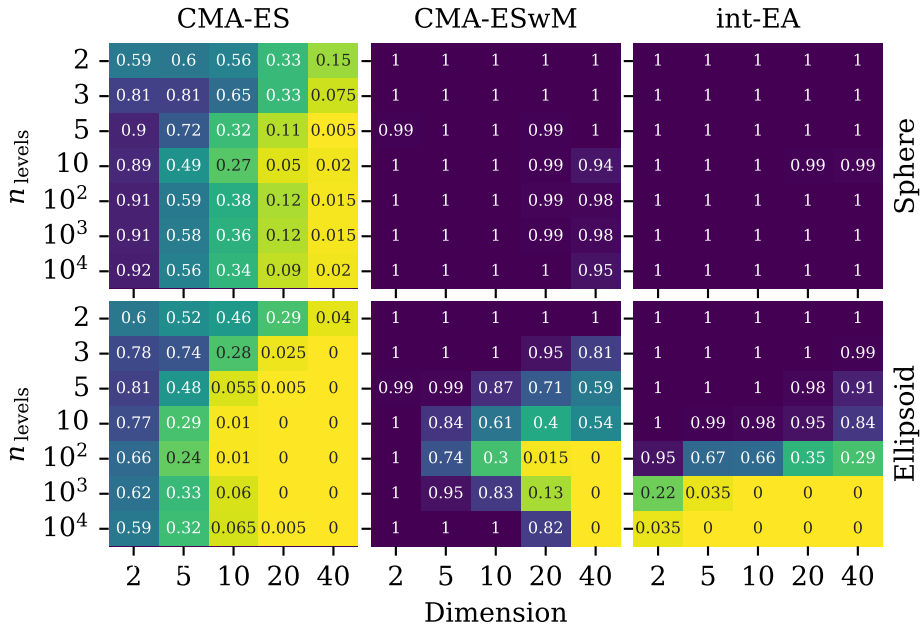
Figure 5.4: Success rates for CMA-ES, CMA-ESwM and int-EA on the sphere function (top row) and ellipsoid function (bottom row), across various dimensions (x-axis) and discretization levels n_{\text{levels}} (y-axis). Each algorithm is given a budget of 2000 evaluations per dimension, with 200 runs conducted for each setting. The target function value is set to 10^{-8} .
