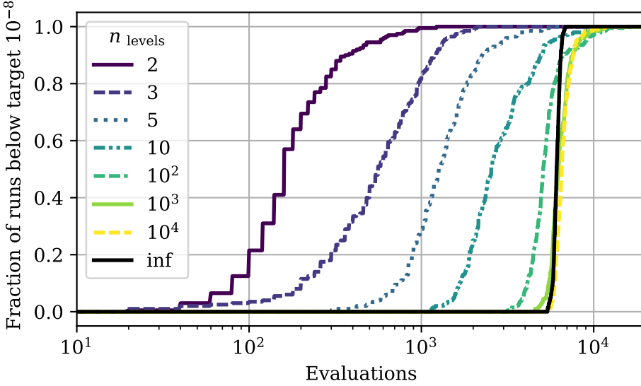
Figure 5.7: Empirical Cumulative Distribution Function for the IPOP-CMA-ESwM with a doubled default population size on the 10 dimensional ellipsoid function for n_{\text{levels}} \in \{2, 3, 5, 10, 10^2, 10^3, 10^4\} and the standard CMA-ES for n_{\text{levels}} \in \{\text{inf}\} . The target function value is set to 10^{-8} and 200 runs are conducted for each setting.
