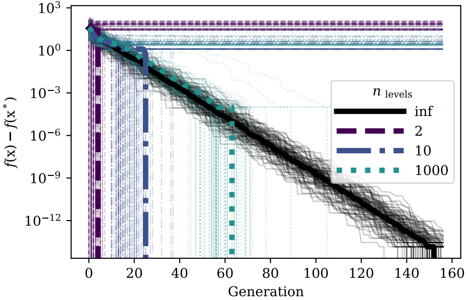
Figure 5.3: Distance to the optimal function value \delta_{f^*} over generations of single CMA-ES runs on a discretized five-dimensional sphere function with a spectrum of different numbers of levels n_{\text{levels}} \in \{2, 10, 10^3, \text{inf}\} for a total of 100 runs and the median (bold line) for each number of levels.
