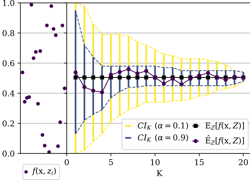
Figure 2.4: Left: The |\Omega_Z| = 20 uniformly distributed values \{f(\mathbf{x}, z_1), \dots, f(\mathbf{x}, z_{|\Omega_Z|})\} . Right: Illustration of two CIs, each consisting of a CI after K = 1, \dots, 20 evaluations for the significance levels \alpha \in \{0.1, 0.9\} . Each CI_K is constructed with the K sampled values available after K evaluations. In addition, the true mean E_Z[f(\mathbf{x}, Z)] and the estimated (sample) mean \hat{E}_Z[f(\mathbf{x}, Z)] are displayed along with the number of sampled values K .
