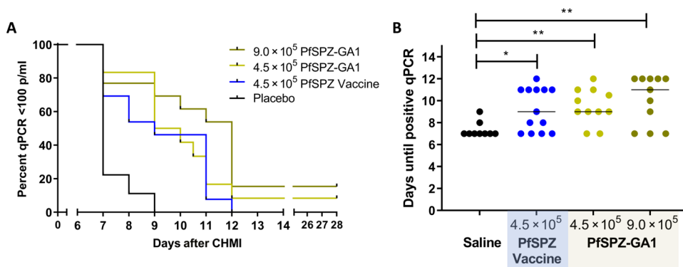
Fig. 3. Parasitemia after CHMI. (A) Kaplan-Meier showing number of volunteers without blood-stage parasitemia as measured by qPCR between 0 to 28 days after CHMI (log-rank, P = 0.0003 ) and (B) days until patency [qPCR > 100 p/ml, for the 9.0 \times 10^5 PfSPZ-GA1 Vaccine (dark green), 4.5 \times 10^5 PfSPZ-GA1 Vaccine (green), 4.5 \times 10^5 PfSPZ Vaccine (blue), and placebo group (black)]. Lines indicate median. (B) shows significance by Mann-Whitney test: * P < 0.05 and ** P < 0.01 .
