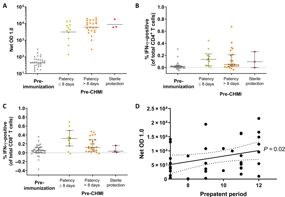
Fig. 5. Relationship between immune parameters and protection. (A) Relationship between anti-PfCSP antibody titers (lines indicate geometric mean), % of (B) IFN- \gamma -producing CD4 ^+ or (C) CD8 ^+ T cells (lines indicate median and interquartile ranges) and the protection status of volunteers. Protection grouped by day of positive qPCR (patency) \leq 8 or > 8 or “sterile” if qPCR negative until day 28. One-way ANOVA, P = 0.05 . (D) Correlation of anti-PfCSP antibody titer 14 days after the final immunization with prepatent period. Pearson correlation P = 0.02 and r = 0.32 .
