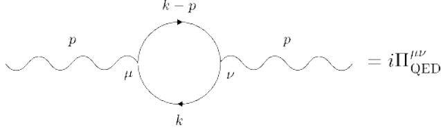
Figure 1.4: Self energy of photon
