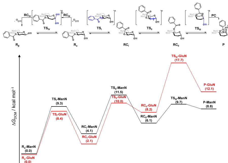
Supplementary Figure 5. The computed reaction profiles for the formation of the dioxanium ion and anomeric \beta -triflate from \alpha -1-O-triflyl-2,4,6-tri-O-methyl-3-O-benzoyl-glucose ( R_\alpha -GluN), and mannose ( R_\alpha -ManN). For clarity the C-2 substituent is removed in all chemdrawings. Gibbs free energies in dichloromethane ( \Delta G_{DCM} , in kcal mol -1 ) are given relative to the anomeric \alpha -triflate R_\alpha for each separate potential energy surface. Computed at PCM(CH 2 Cl 2 )-M06-2X//6-311++G(d,p)/PCM(CH 2 Cl 2 )-B3LYP-D3BJ/6-31+g(d). See Supporting Information Table S2 for all data of the stationary points of the reaction profiles.
