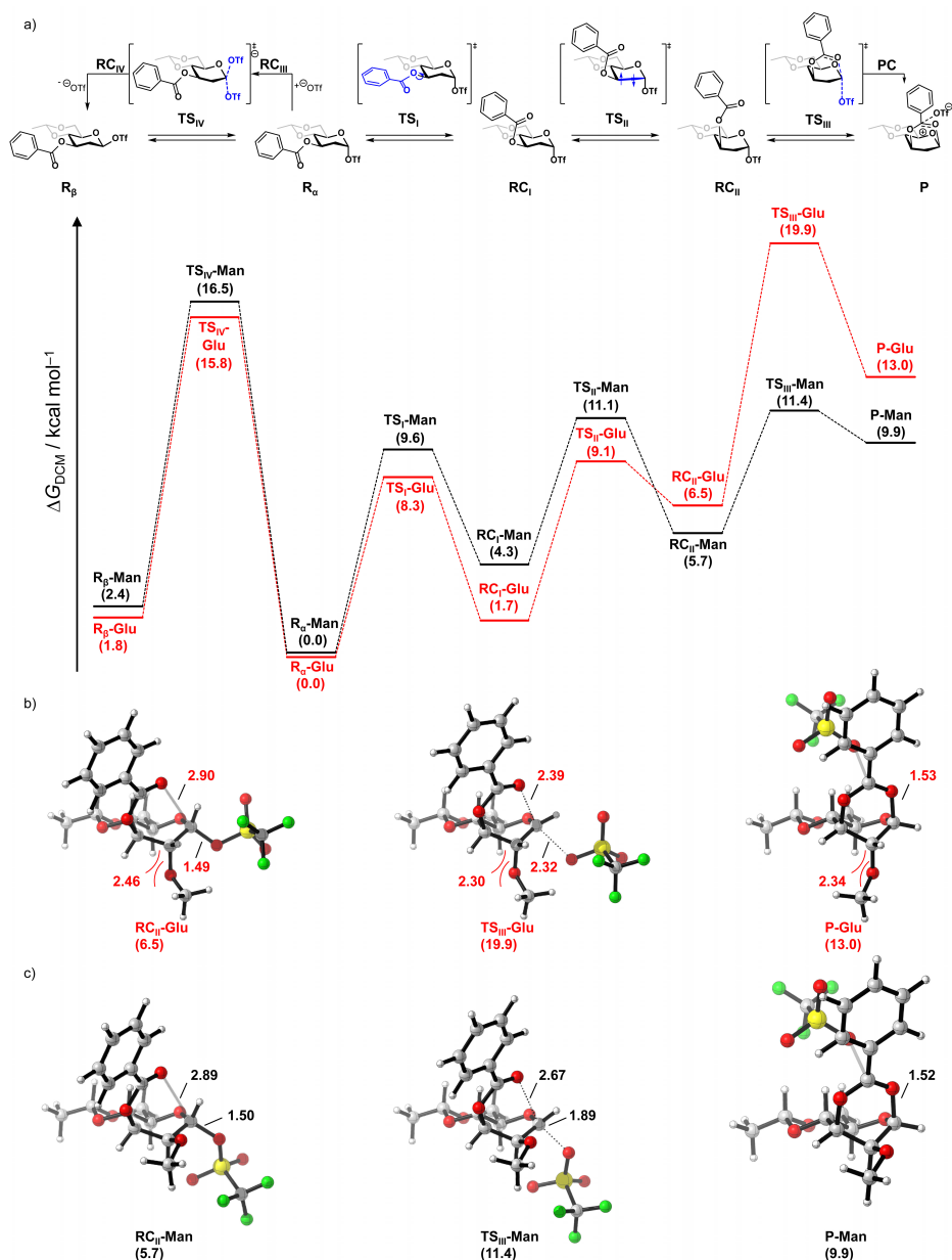
Figure 2. a) The computed reaction profiles for the formation of the dioxanum ion and anomeric \beta -triflate from \alpha -1- O -triflyl-2- O -methyl-3- O -benzoyl-4,6- O -ethylidene glucose ( R_{\alpha} -Glu) and mannose ( R_{\alpha} -Man). For clarity the C-2 substituent is removed in all structures in Figure 2a. Gibbs free energies in dichloromethane ( T = 213.15 K, \Delta G_{DCM} , in kcal mol -1 ) are given relative to the anomeric \alpha -triflate R_{\alpha} for each separate potential energy surface. Structures of RC_{II} , TS_{III} , PC and P for the (c) mannoside and (d) glucoside, were visualized by Cylview. 47 Distances are given in Å. Computed at PCM(CH 2 Cl 2 )-M06-2X/6-311++G(d,p)//PCM(CH 2 Cl 2 )-B3LYP-D3BJ/6-31+g(d). See Supporting Information Table S2 for all data of the stationary points of the reaction profiles.
