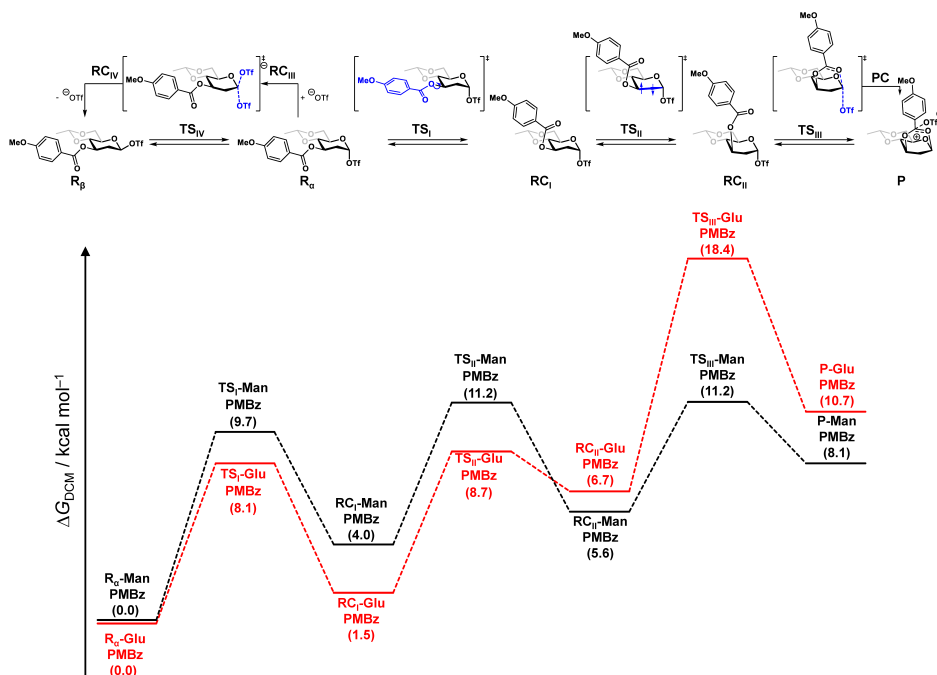
Supplementary Figure 6. The computed reaction profiles for the formation of the dioxanium ion and anomeric β-triflate α-1- O -triflyl-2- O -methyl-3- O -(4- O -methyl-benzoyl)-4,6- O -ethylidene-glucose (R α -Glu) and mannose (R α -Man). For clarity the C-2 substituent is removed in all chemdrawings. Gibbs free energies in dichloromethane (ΔG DCM , in kcal mol -1 ) are given relative to the anomeric α-triflate R α for each separate potential energy surface. Computed at PCM(CH 2 Cl 2 )-M06-2X//PCM(CH 2 Cl 2 )-B3LYP-D3BJ/6-31+G(d). See Supporting Information Table S2 for all data of the stationary points of the reaction profiles.
