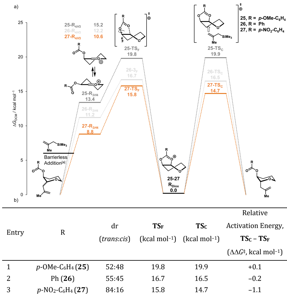
Figure 2. a) Reaction profiles of nucleophilic substitution reactions of 2- O -acyloxy pyran cations ( 25 , 26 , and 27 ) with 2-methallyltrimehtylsilane ( 10 , C ). b) Summary of critical substitution barrier heights compared to experimentally found diastereomeric ratios. 30,34 Computed at SMD(dichloromethane)-revDSD-PBEP86-D4-def2TZVPP/PCM(dichloromethane)-B3LYP-D3BJ-def2TZVPP and expressed as relative Gibbs free energy (T=228.15 K) in kcal mol -1 . [a] Electronically barrierless, determined by constrained PES analysis.
