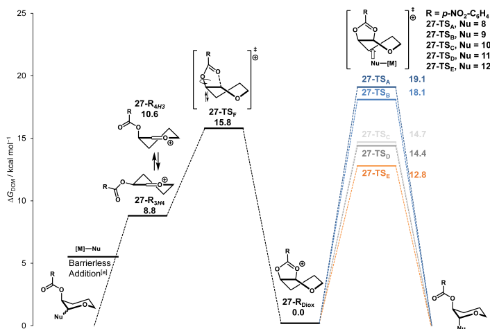
Figure S4. Reaction profiles of nucleophilic substitution reactions of 2- O - p -nitrobenzoyl pyran cations (27) with C -nucleophiles 8 (A), 9 (B), 10 (C), 11 (D), [b] 12 (E). [b] Computed at SMD(dichloromethane)-revDSD-PBEP86-D4-def2TZVPP//PCM(dichloromethane)-B3LYP-D3BJ-def2TZVPP and expressed as relative Gibbs free energy (T=228.15K) in kcal mol -1 . [a] Electronically barrierless, determined by constrained PES analysis. [b] The t -Bu groups of nucleophiles 11, 12 were replaced with electronically similar but smaller methyl groups for computational feasibility.
