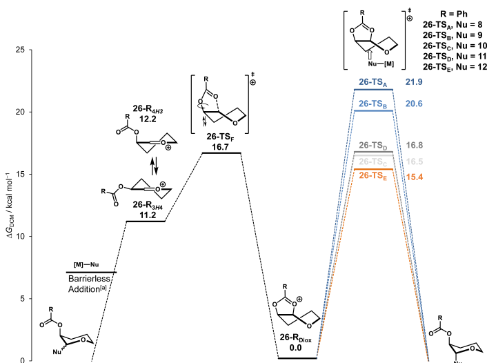
Figure S3. Reaction profiles of nucleophilic substitution reactions of 2- O -benzoyl pyran cations (26) with C -nucleophiles 8 (A), 9 (B), 10 (C), 11 (D), [b] 12 (E). [b] Computed at SMD(dichloromethane)-revDSD-PBEP86-D4-def2TZVPP//PCM(dichloromethane)-B3LYP-D3BJ-def2TZVPP and expressed as relative Gibbs free energy (T=228.15K) in kcal mol -1 . [a] Electronically barrierless, determined by constrained PES analysis. [b] The t -Bu groups of nucleophiles 11, 12 were replaced with electronically similar but smaller methyl groups for computational feasibility.
