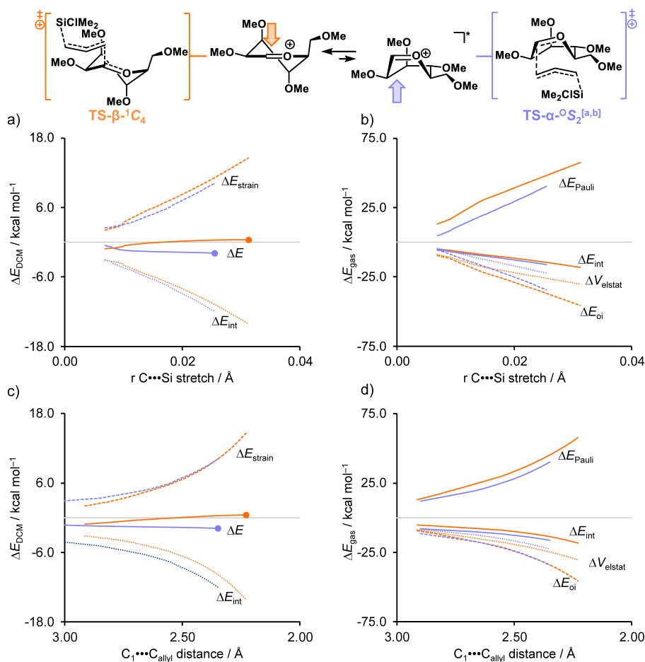
Figure 7. Activation strain (a and c) and energy decomposition analysis (b and d) for the S_E2' reactions of allyl(chloro)dimethylsilane + mannosyl cation via the \alpha -product-forming TS-\alpha^{-0}S_2 (light blue) and via the \beta -product-forming TS-\beta^{-1}C_4 (orange). Energy values are plotted to the transition state (indicated by a dot), along the IRC projected on the \text{C}\cdots\text{Si} bond stretch (a and b) or \text{C}_1\cdots\text{C}_{\text{allyl}} bond distance (c and d). Schematic representation of the physical factors influencing the facial selectivity of the mannosyl cation (d). Energies are depicted as electronic energies and were computed at \text{PCM}(\text{CH}_2\text{Cl}_2)\text{-B3LYP}/6\text{-311G(d,p)} for \Delta E_{\text{DCM}} or \text{ZORA-B3LYP}/\text{TZ2P}/\text{PCM}(\text{CH}_2\text{Cl}_2)\text{-B3LYP}/6\text{-311G(d,p)} for \Delta E_{\text{gas}} . [a] The TS-\alpha^{-0}S_2 pathway was plotted against the constrained potential energy surface. 41 [b] The itinerary leading up to TS-\alpha^{-0}S_2 starts from a boat-like non-stationary point.
