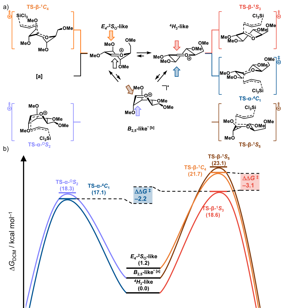
Supplementary Figure S3. The possible S E 2' reaction pathways (a) and the corresponding reaction profile (b) of the addition of allyltrichlorosilane to the glucosyl cation, via the following transition states: TS-β-1C 4 (orange), TS-β-1S 5 (brown), TS-β-1S 3 (red), TS-α-0S 2 (light blue) and TS-α-4C 1 (blue). Energies are depicted as Gibbs free energies ( T = 213.15 K) and were computed at PCM(CH 2 Cl 2 )-B3LYP/6-311G(d,p). [a] The itinerary leading up to TS-α-0S 2 and TS-β-1S 5 start from a boat-like non-stationary point.
