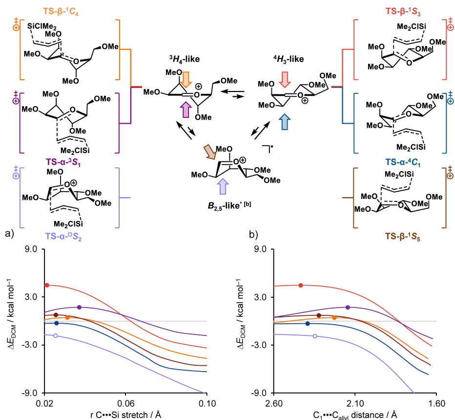
Supplementary Figure S2. The possible \text{SE}_2' reaction pathways of the addition of allyl(chloro)dimethylsilane to the mannosyl cation, via the following transition states: TS- \beta -C 4 (orange), TS- \beta -S 5 (brown), TS- \beta -S 3 (red), TS- \alpha -S 2 (light blue) and TS- \alpha -C 1 (blue). Energy values are plotted along the IRC projected on the C...Si bond stretch (a) or C...C allyl bond distance (b). Transition states are indicated by a filled dot. The representative structure of the TS- \alpha -S 2 is indicated by a non-filled dot. Energies are depicted as electronic energies and were computed at PCM(CH 2 Cl 2 )-B3LYP/6-311G(d,p). [a] A representative structure for the transition state geometry was used. [b] The itinerary leading up to TS- \alpha -S 2 and TS- \beta -S 5 start from a boat-like non-stationary point.
