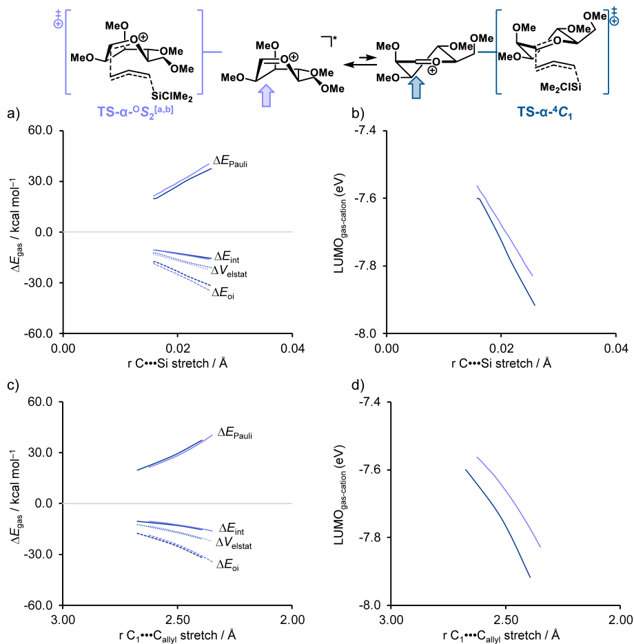
Supplementary Figure S14. Energy decomposition analysis (a and c) and LUMO energy (in eV) of the mannosyl cation (b and d) for the S_N2' reactions of allyl(chloro)dimethylsilane + mannosyl cation via the \alpha -product forming TS- \alpha^4C_1 (blue) and via the \alpha -product forming TS- \alpha^0S_2 (light blue), along the IRC projected on the \text{C}\cdots\text{Si} bond stretch (a and b) and the \text{C}_1\cdots\text{C}_{\text{allyl}} bond distance (c and d). Energies are depicted as electronic energies and were computed at ZORA-B3LYP/TZ2P//PCM( \text{CH}_2\text{Cl}_2 )-B3LYP/6-311G(d,p). [b] The itinerary leading up to TS- \alpha^0S_2 starts from a boat-like non-stationary point.
