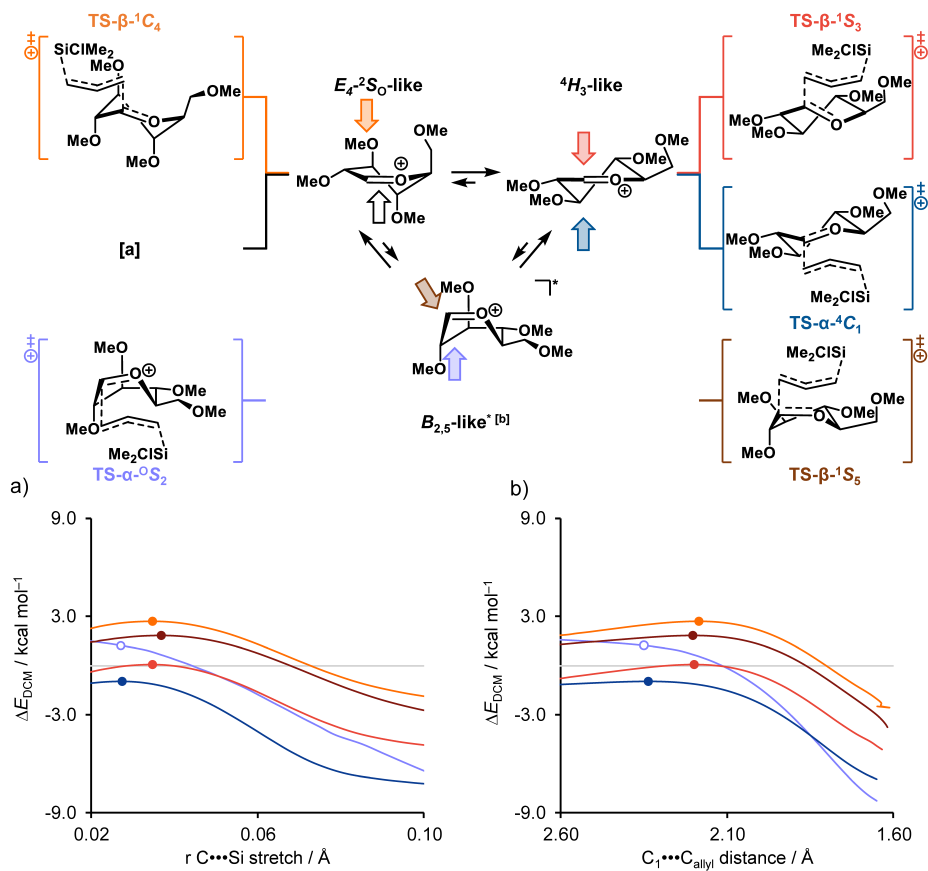
Supplementary Figure S1. The possible S_E2' reaction pathways of the addition of allyl(chloro)dimethylsilane to the glucosyl cation, via the following transition states: TS-\beta-1C_4 (orange), TS-\beta-1S_5 (brown), TS-\beta-1S_3 (red), TS-\alpha-0S_2 (light blue) and TS-\alpha-4C_1 (blue). Energy values are plotted along the IRC projected on the C \cdots Si bond stretch (a) or C_1 \cdots C_{allyl} bond distance (b). Transition states are indicated by a filled dot. The representative structure of the TS-\alpha-0S_2 is indicated by a non-filled dot. Energies are depicted as electronic energies and were computed at PCM(CH 2 Cl 2 )-B3LYP/6-311G(d,p). [a] A representative structure for the transition state geometry was used. 41 [b] The itinerary leading up to TS-\alpha-0S_2 and TS-\beta-1S_5 start from a boat-like non-stationary point.
