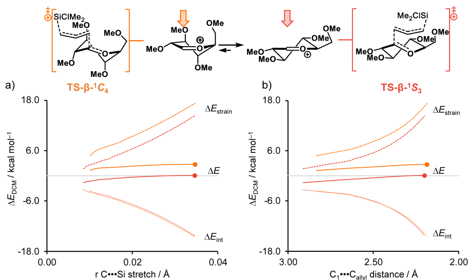
Figure 6. Activation strain analysis for the S_E2' reactions of allyl(chloro)dimethylsilane + glucosyl cation via the \beta -product-forming TS-\beta-1C_4 (orange) and via the \beta -product-forming TS-\beta-1S_3 (red), where the energy values are plotted to the transition state (indicated by a dot), along the IRC projected on the C \cdots Si bond stretch (a) or C_1 \cdots C_{allyl} bond distance (b). Energies are depicted as electronic energies and were computed at PCM( CH_2Cl_2 )-B3LYP/6-311G(d,p) for \Delta E_{DCM} . [a] The TS-\alpha-0S_2 pathway was plotted against the constrained potential energy surface. 41
