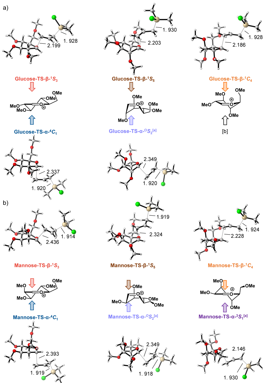
Figure 2. Structures 42 of the transition states of the S_E2' reactions of ally(chloro)dimethylsilane and the glucosyl (a) or mannosyl (b) cations. Key distances are given in Å. [a] A representative structure for the transition state geometry was used. 41 [b] The bottom-side attack on the ^3H_4 yields is unfavorable, instead the glycosyl cations deform to other transition state shapes during searches.
