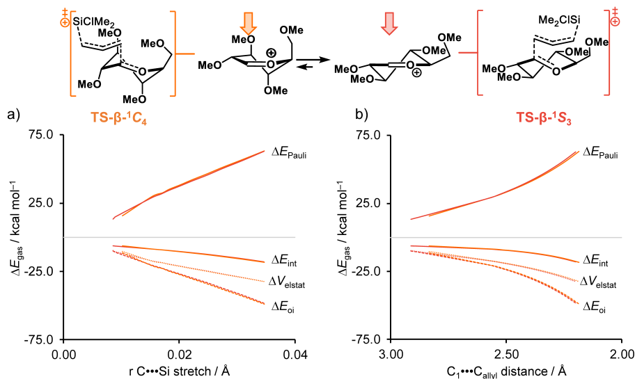
Supplementary Figure S12. Energy decomposition analysis for the S_N2' reactions of allyl(chloro)dimethylsilane + glucosyl cation via the \beta -product forming TS- \beta -1C 4 (orange) and via the \beta -product forming TS- \beta -1S 3 (red), where the energy values are plotted to the transition state (indicated by a dot), along the IRC projected on the C...Si bond stretch (a) or C 1 ...C allyl bond distance (b). Energies are depicted as electronic energies and were computed at ZORA-B3LYP/TZ2P//PCM(CH 2 Cl 2 )-B3LYP/6-311G(d,p).
