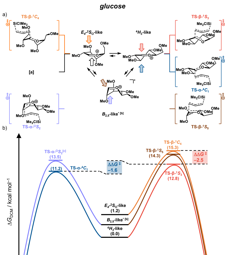
Figure 3. The possible S_E2' reaction pathways (a) and the corresponding reaction profiles (b) of the addition of allyl(chloro)dimethylsilane to the glucosyl cation via the following transition states: TS- \beta -1 C_4 (orange), TS- \beta -1 S_5 (brown), TS- \beta -1 S_3 (red), TS- \alpha - O_2S_2 (light blue) and TS- \alpha -4 C_1 (blue). Energies are depicted as Gibbs free energies ( T = 213.15 K) and were computed at PCM( \text{CH}_2\text{Cl}_2 )-B3LYP/6-311G(d,p). [a] The TS- \alpha -3 S_1 is unfavorable and could not be located. [b] The itinerary leading up to TS- \alpha - O_2S_2 and TS- \beta -1 S_5 start from a boat-like non-stationary point. [c] A representative structure for the transition state geometry was used. 41
