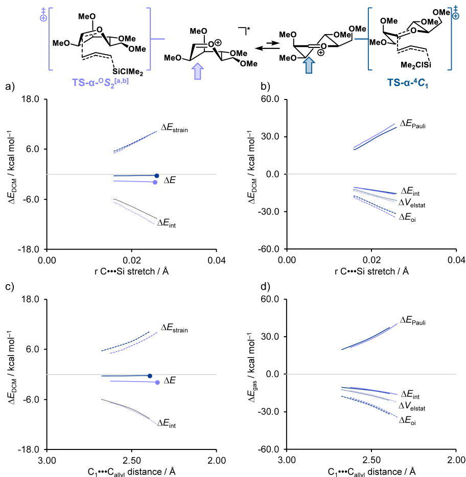
Figure 8. Activation strain (a and c) and energy decomposition analysis (b and d) for the S_E2' reactions of allyl(chloro)dimethylsilane + mannosyl cation via the \alpha -product-forming TS-\alpha^4C_1 (blue) and TS-\alpha-O_S2 (light blue), where the energy values are plotted to the transition state (indicated by a dot), along the IRC projected on the C\cdots Si bond stretch (a and b) or C_1\cdots C_{\text{allyl}} bond distance (c and d). Energies are depicted as electronic energies and were computed at PCM( \text{CH}_2\text{Cl}_2 )-B3LYP/6-311G(d,p) for \Delta E_{\text{DCM}} or ZORA-B3LYP/TZ2P//PCM( \text{CH}_2\text{Cl}_2 )-B3LYP/6-311G(d,p) for \Delta E_{\text{gas}} . [a] The TS-\alpha-O_S2 pathway was plotted against the constrained potential energy surface. [41] [b] The itinerary leading up to TS-\alpha-O_S2 starts from a boat-like non-stationary point.
