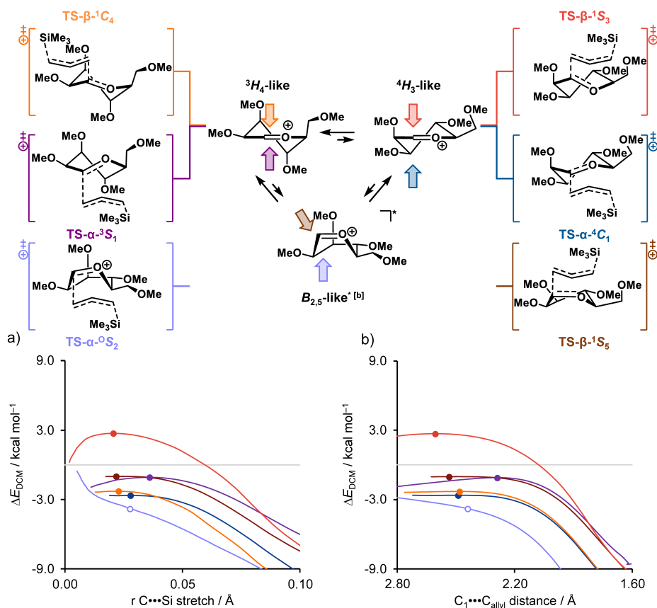
Supplementary Figure S8. The possible S_E2' potential energy surfaces of the addition of allyltrimethylsilane to the mannosyl cation, via the following transition states: TS-β-1C 4 (orange), TS-β-1S 5 (brown), TS-β-1S 3 (red), TS-α-0S 2 (light blue) and TS-α-4C 1 (blue). Energy values are plotted along the IRC projected on the C...Si bond stretch (a) or C 1 ...C allyl bond distance (b). Transition states are indicated by a filled dot. The representative structure of the TS-α-0S 2 is indicated by a non-filled dot. Energies are depicted as electronic energies and were computed at PCM(CH 2 Cl 2 )-B3LYP/6-311G(d,p). [a] A representative structure for the transition state geometry was used. [b] The itinerary leading up to TS-α-0S 2 and TS-β-1S 5 start from a boat-like non-stationary point.
