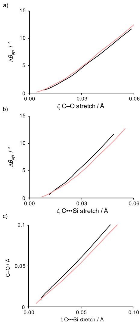
Figure S5. Degree of pyramidalization for the \text{S}_{\text{E}}2' reactions of allyltrimethylsilane and cation 1 via the top face-attack (black: chair-like TS) and bottom face-attack (pink: twist boat-like TS), where the energy values are plotted from the reactant complex to the transition state, along the IRC projected on the (a) C–O (b) C•••Si bond stretch. The pyramidalization angle is defined as the sum of the three \theta_{\text{R–C–R}} . Computed at COSMO( \text{CH}_2\text{Cl}_2 )-ZORA-B3LYP/TZ2P//PCM( \text{CH}_2\text{Cl}_2 )-B3LYP/6-311G(d,p).
