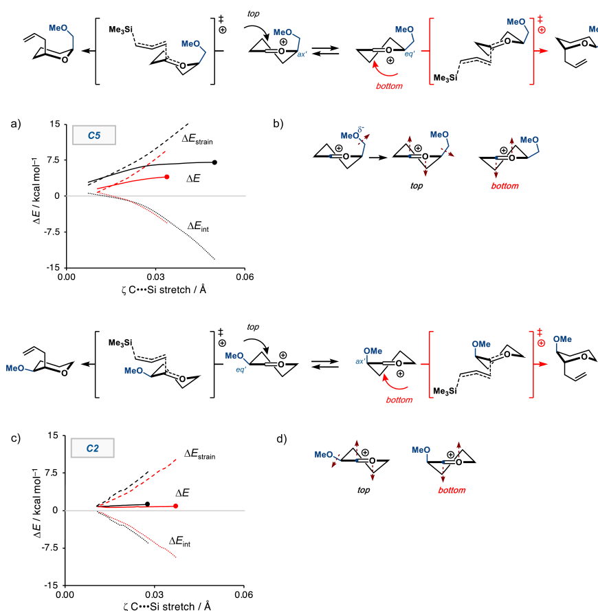
Figure 6. (a,c) Activation strain model for the S_E2' reactions of allyltrimethylsilane + cation 5 and 2 via the top face-attack (black: chair-like TS) and bottom face-attack (red: chair-like TS), where the energy values are plotted to either the transition state or a local maximum (indicated by a dot), along the IRC projected on the C...Si bond stretch. (b,d) Movement of the C1=O + bond and substituent along the S_E2' reaction for cation 5 and 2 . Computed at COSMO(CH 2 Cl 2 )-ZORA-B3LYP/TZ2P//PCM(CH 2 Cl 2 )-B3LYP/6-311G(d,p).
