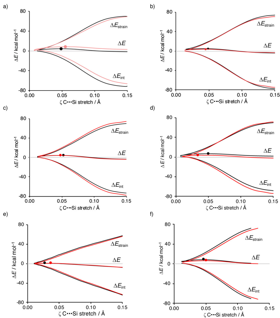
Figure S1. Activation strain model for the S_E2' reactions of allyltrimethylsilane + cation 1 (a) via the top face-attack (black: chair-like TS) and bottom face-attack (pink: twist boat-like TS), and 4 (b), 3 (c), 5 (d), 2 (e), 6 (f) via the top face-attack (black: chair-like TS) and bottom face-attack (red: chair-like TS), where the energy values are plotted along the IRC projected on the C\cdots Si bond stretch. Computed at COSMO( CH_2Cl_2 )-ZORA-B3LYP/TZ2P//PCM( CH_2Cl_2 )-B3LYP/6-311G(d,p).
