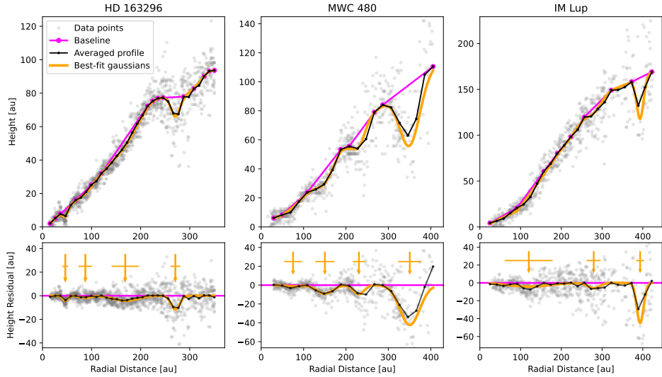
Figure 3.B.10: Data (grey dots), averaged profile (black curve), assumed baseline (pink profile), and best-fit Gaussians (orange line) obtained for each system from the analysis in Sect. 3.2.1 for ^{12}\text{CO} . The bottom panels show the residuals obtained after subtracting the baseline profile from the data points. The vertical arrows mark the best-fit centre of each Gaussian component considered in each system. The horizontal line marks the width of the Gaussian component.
