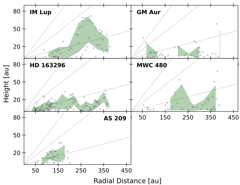
Figure 3.B.7: \text{HCO}^+ data points.
