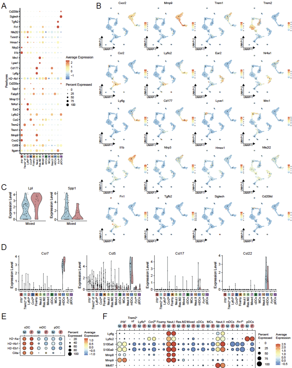
Supplementary Figure S6. Comparison of aortic myeloid cells between aged male and female Ldlr -/- mice.
