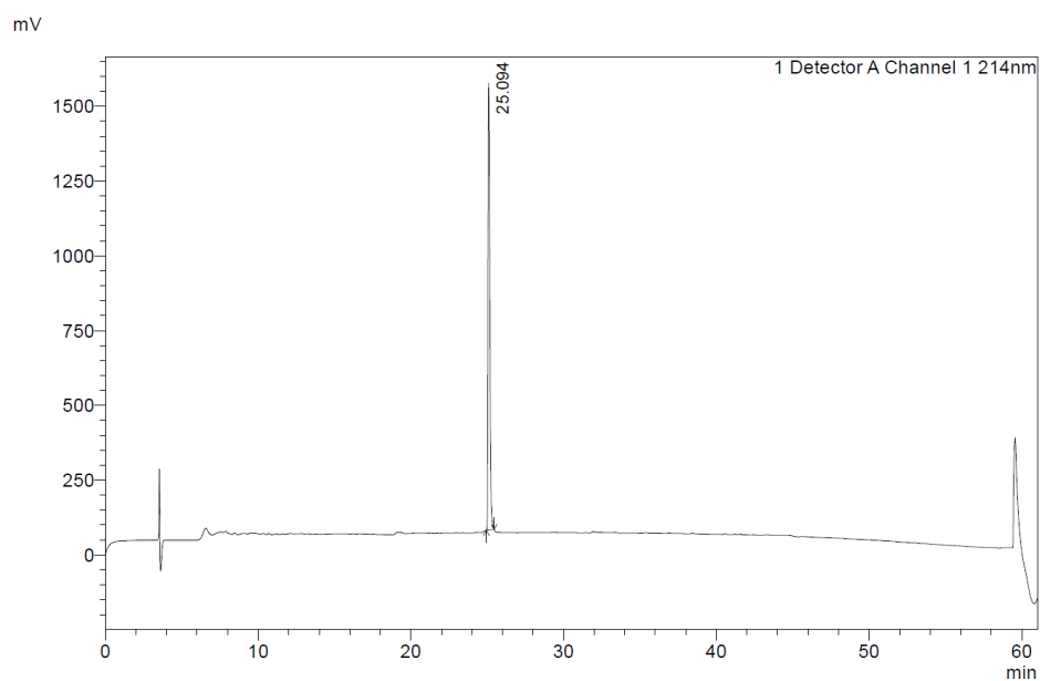
Figure S12. HPLC trace showing the reinjection of purified Oct-Glu9 (10). The peptide eluted as a single peak at 25.094 min using the HPLC method C.
