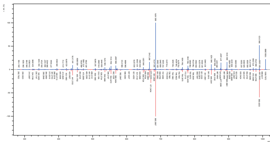
Figure S6. Direct MS/MS comparison of surfactin Leu/Ile7 C13 from the extract of Bacillus sp. 90A-23 with surfactin Leu/Ile7 C13 spectrum from GNPS spectral library (CCMSLIB00000006885).
