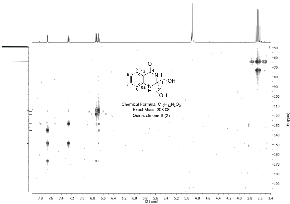
Figure S15. HMBC spectrum of quinazolinone B (2) in \text{CD}_3\text{OD} .
