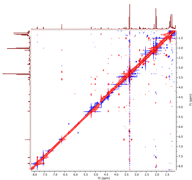
Figure S15. NOESY spectrum of saquayamycin N (1) (850 MHz, in \text{CD}_3\text{OD} ).
