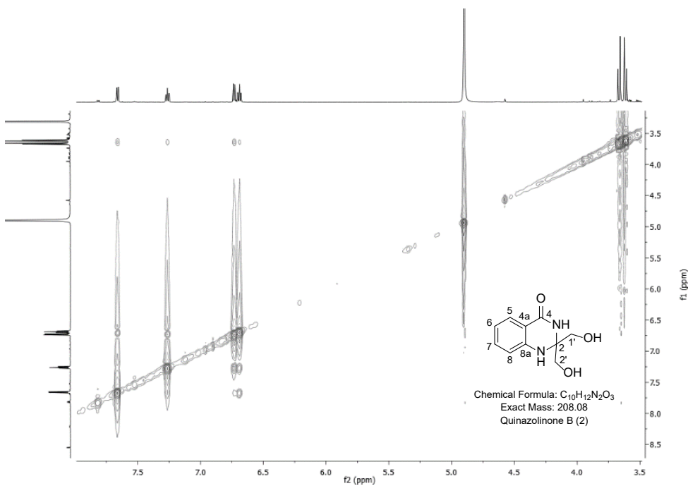
Figure S16. ^1\text{H} - ^1\text{H} NOSEY spectrum of quinazolinone B (2) in \text{CD}_3\text{OD} .
