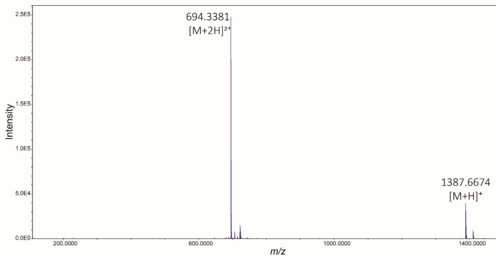
Figure S5. HRMS spectrum of 2.
