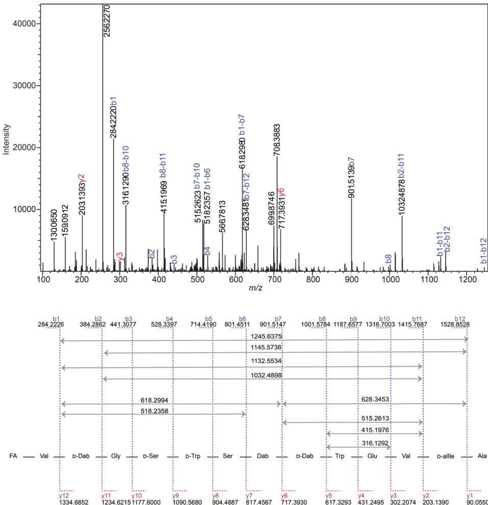
Figure S1. MS/MS spectrum of tridecaptin A 3 produced by of Paenibacillus sp. JJ-21 (precursor ion [M + 3H] 3+ m/z 539.9712). The assignment of the sequence of amino acid residues at the top of the spectrum is based on the mass differences between the consecutive y and b ions.
