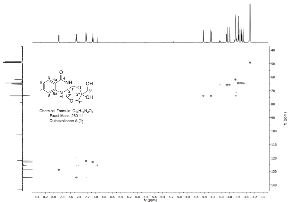
Figure S6. HSQC spectrum of quinazolinone A (1) in CD_3OD .
