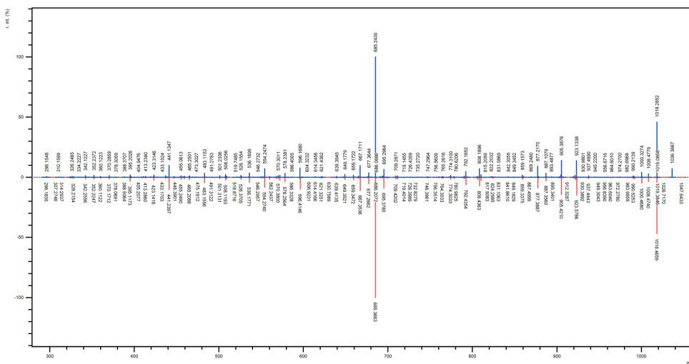
Figure S8. Direct MS/MS comparison of surfactin Leu/Ile7 C15 from the extract of Bacillus sp. 90A-23 with surfactin Leu/Ile7 C15 spectrum from GNPS spectral library (CCMSLIB00000006895).
