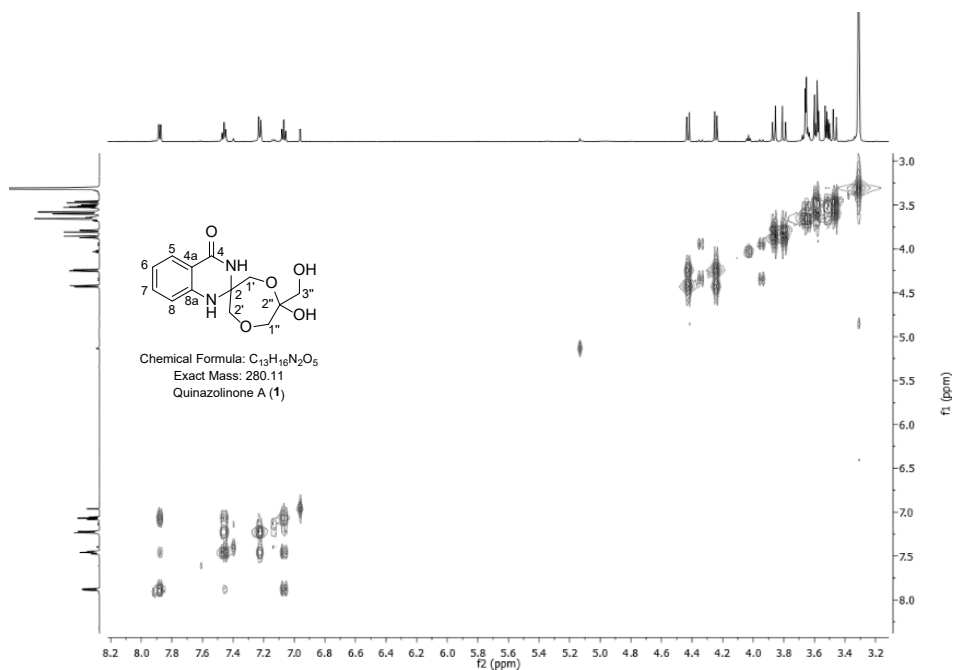
Figure S5. ^1H - ^1H COSY spectrum of quinazolinone A (1) in CD_3OD .
