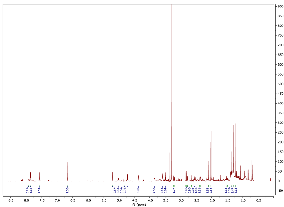
Figure S10. ^1\text{H} NMR spectrum of saquayamycin N (1) (850 MHz, in \text{CD}_3\text{OD} ).
