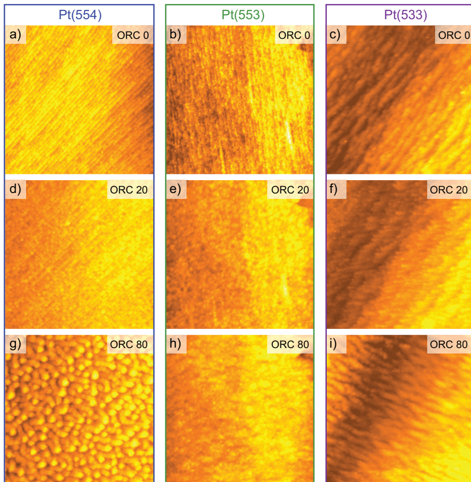
Figure O.5: EC-STM Images of Pt(111)-Vicinal Surfaces after Oxidation-Reduction Cycles. (a), (b), and (c) show the as-prepared Pt(554), Pt(553), and Pt(533) electrodes, respectively. (d), (e), and (f) show the same samples on the same place after 20 ORCs. Finally, (g), (h), and (i) show again the same place on the surfaces after 80 ORCs. All images are 100 \times 100 \text{ nm}^2 , and were recorded in 0.1 \text{ M HClO}_4 at sample and tip potentials of 0.1 \text{ V} and 0.15 \text{ V} , respectively.
