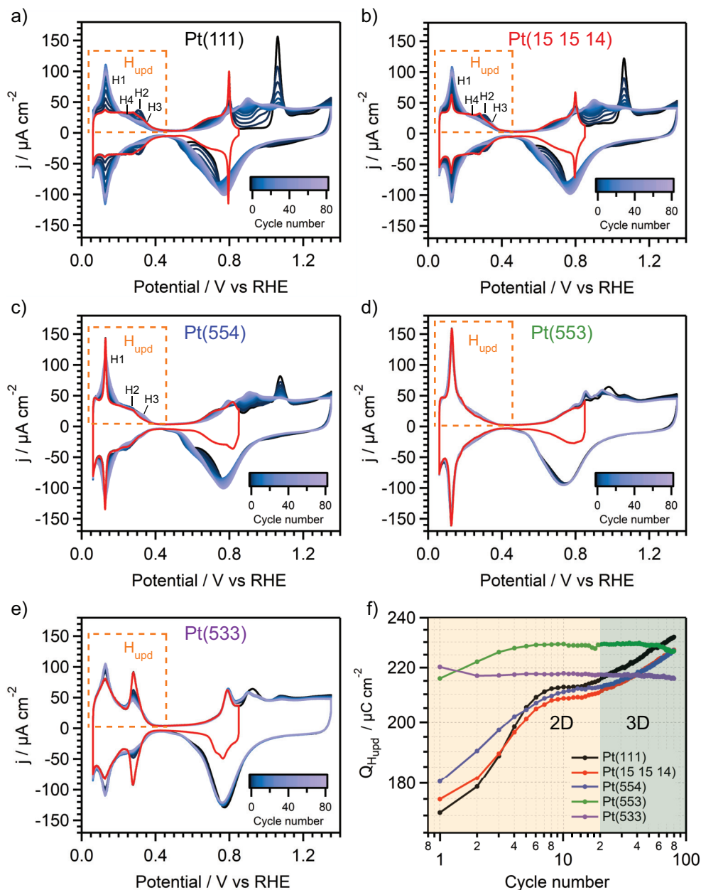
Figure O.4: Oxidation-Reduction Cycles on Pt(111) and its Vicinal Surfaces. (a-e) Oxidation-reduction cycles on Pt(111), Pt(15 15 14), Pt(554), Pt(553), and Pt(533). The H_{\text{upd}} region is highlighted with an orange rectangle, while the step-related peaks within are indicated as H1-H4. (f) The H_{\text{upd}} charge versus the cycle number (for each of the surfaces studied) is a good electrochemical measure for the roughness [6]. The two roughening regimes, in 2D and in 3D, are indicated in yellow and green, respectively.
