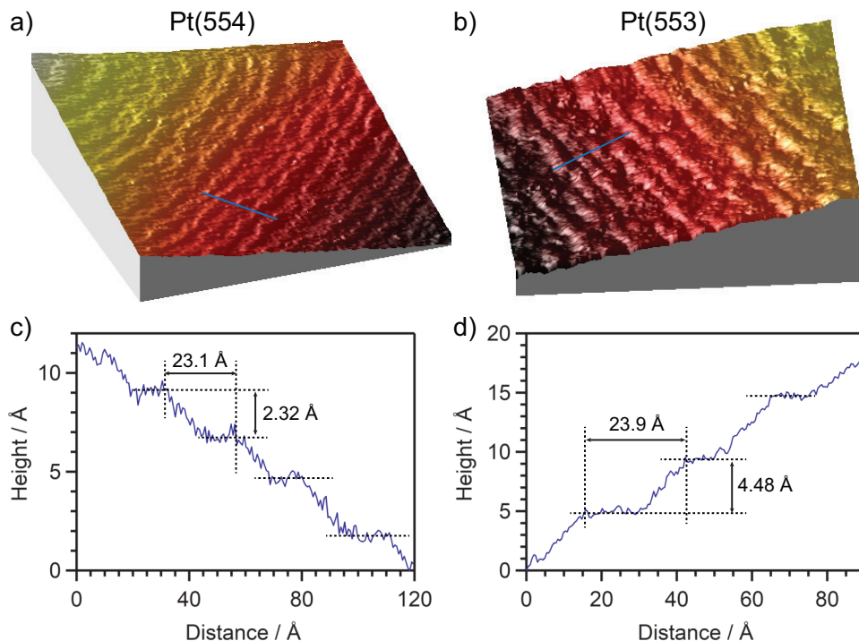
Figure 3.1: EC-STM Measurements of Pt(111)-Vicinal Surfaces. 3D rendered EC-STM images of (a) Pt(554) and (b) Pt(553), recorded in 0.1 M \text{HClO}_4 with U_s = 0.1 V and U_t = 0.15 V. Both images are 48 \times 48 \text{ nm}^2 . The blue lines crossing the steps on Pt(554) and Pt(553) indicate the positions of the corresponding height lines shown in (c) and (d). Note that the step height on Pt(553) is twice the one on Pt(554) and that both surfaces show an almost equal terrace width, although it should be theoretically 46 % smaller on Pt(553).
