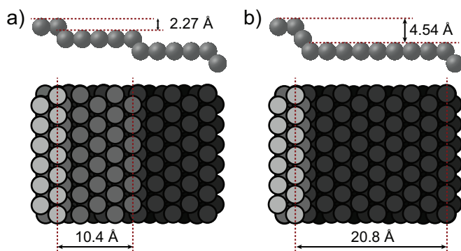
Figure 3.2: Ball Model of a Pt(553) Surface: (a) with single steps, (b) with double, bunched steps.
