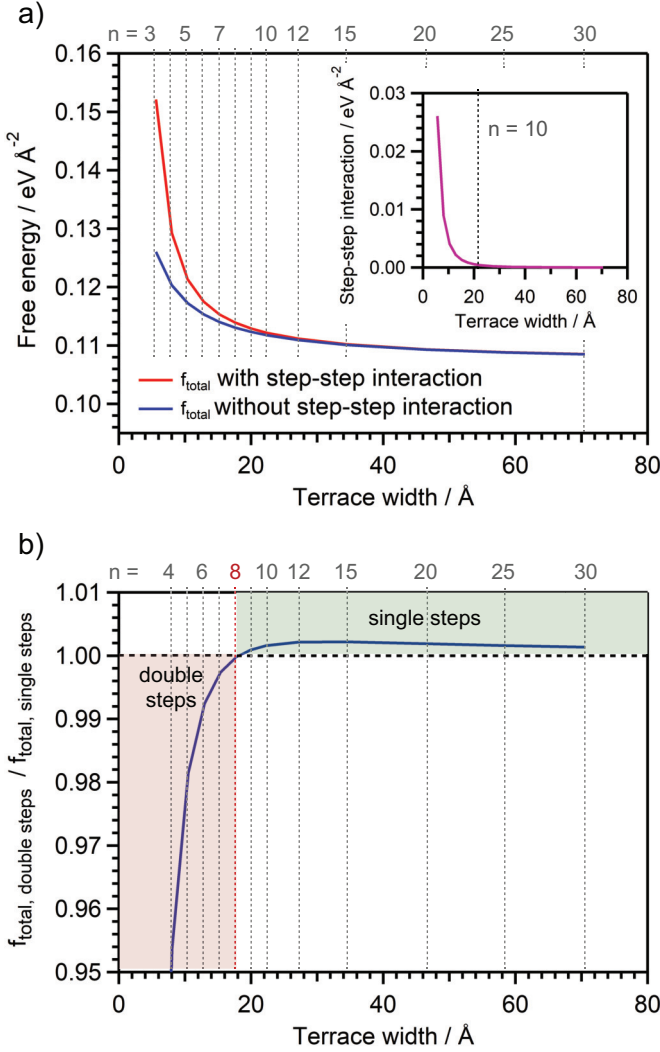
Figure 3.4: Thermodynamics of Step Bunching. (a) f_{total} with step-step interaction (red), f_{total} without step-step interaction (blue), and step-step interaction (inset, in purple) versus the terrace width for T = 1300 K. For the calculations, we used equations 3.1 and 3.2, with f_{terr} = 1.07 \text{ eV } \text{\AA}^{-2} from Ref. [25] and the values of f_{step}^0 = 0.120 \text{ eV } \text{\AA}^{-1} and f_{kink}^0 = 0.206 \text{ eV} from Ref. [26]. We extracted the step interaction parameter B_{step} = 12.76 \text{ eV } \text{\AA}^2 from the one reported in Ref. [25], which we extrapolated to match with our temperature (see Appendix B). (b) Surface free energy ratio between configurations with double and single steps. To calculate the surface free energy for the double steps we reasonably approximated f_{doublestep}^0 = 2 \times f_{step}^0 = 0.240 \text{ eV } \text{\AA}^{-1} and f_{doublekink}^0 = 2 \times f_{kink}^0 = 0.412 \text{ eV} . We extracted B_{doublestep} = 17.11 \text{ eV } \text{\AA}^2 by scaling B_{step} with the ratio of the dipole moments of double steps and single steps, as explained in the Appendix B.
