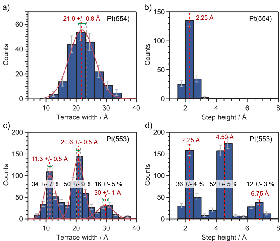
Figure 3.3: Statistical Analysis of the Surface Structure. (a) and (b) show the terrace width and step-height distributions of Pt(554), while (c) and (d) show the ones of Pt(553). The values in red and the red dashed lines indicate the center of each peak. For (a) and (c), we obtained these values from Gaussian fits, with which we deconvoluted the peaks in the case of Pt(553). The statistical errors shown with gray error bars on each bin lead to uncertainties on the center values (green arrows) as well as on the percentages of single, double, and triple steps, which are reported in black on top of the corresponding peak.
