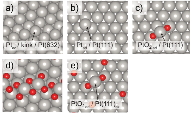
Figure 2.4: Ball Models of Step and Adatom Configurations. (a) Bare platinum step on a Pt(632) surface, which was used to calibrate the total energy scale via the Pt-adatom at the kink site. (b) Pt-adatom on an fcc site on a Pt(111) terrace. (c) PtO_2 -adatom on a bridge site on a Pt(111) terrace. (d) A fully oxidized step forming PtO_2 oxide chains similar to the spokes on the terraces [89,90]. (e) PtO_2 -adatom on a bridge site on a Pt(111) terrace that is covered with a perfectly ordered 4/25 ML O_{ads} superstructure.
