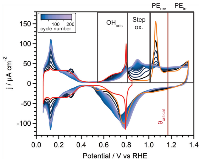
Figure 2.1: Oxidation-Reduction Cycles on Pt(111). The CV to only 0.85 V and the first ORC are shown in red and in orange, respectively, while the remaining ORCs are indicated according to the color scale. The OH adsorption, step oxidation, PE rev , and PE irr regions are indicated, as well as the voltage at the critical coverage. The scan rate is 50 mV s -1 .
