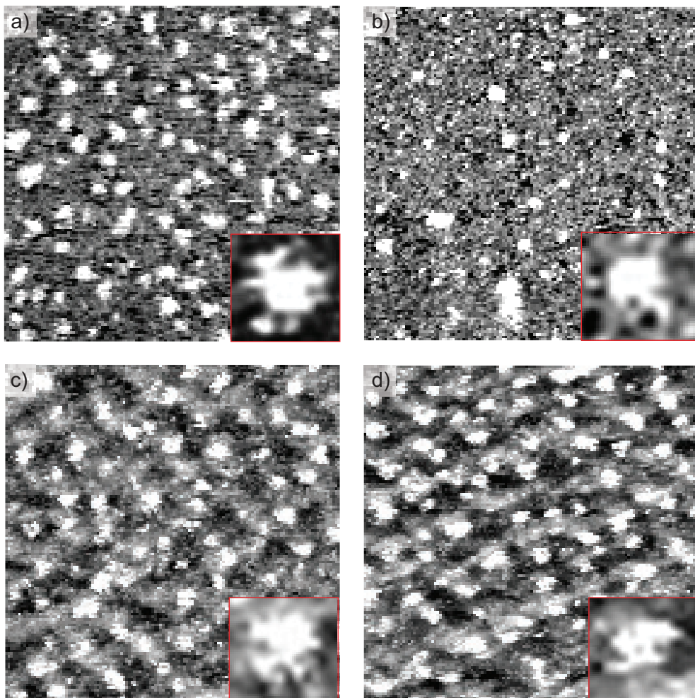
Figure 2.9: Degree of Dendritic Island Shape as Function of ORC-number. (a) As a reference, after holding the potential at 1.35 V for 200 s before reducing to 0.3 V with 25 mV/s. (b) After the first ORC between 0.06 V and 1.35 V. (c) After 6 ORCs. (d) After 7 ORCs. All ORCs are performed with a scan rate of 50 mV/s. All images are 80 \times 80 \text{ nm}^2 . Larger scale images are provided in Appendix A.
