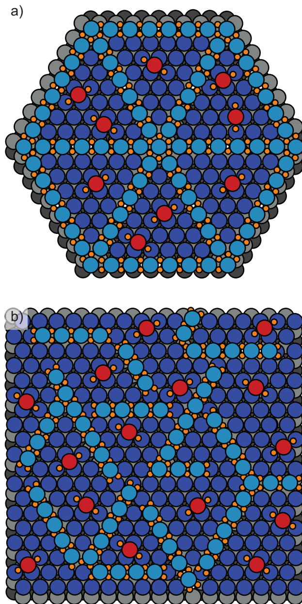
Figure 2.2: The Irreversible Place-Exchange Regime. The Pt atoms of the original, flat terrace are colored in dark blue, the lifted \text{Pt}_{\text{rev}} atoms in light blue, forming spokes or rows, the oxygen atoms in orange, and the \text{Pt}_{\text{irr}} atoms that are pushed onto the terrace, thus becoming \text{PtO}_2 -adatoms, in dark red. The \text{PtO}_2 -adatoms lead eventually to the growth of the nano-islands. (a) shows one fully ordered spoke-wheel structure without any disorder present. However, from [41, 71, 86] we know that, probably due to entropy, a certain degree of disorder is present. Therefore, (b) shows an impression of a disordered spoke-wheel phase: elements of the original triangles are still visible, in which the \text{PtO}_2 -adatoms, the \text{Pt}_{\text{irr}} atoms, are trapped .
