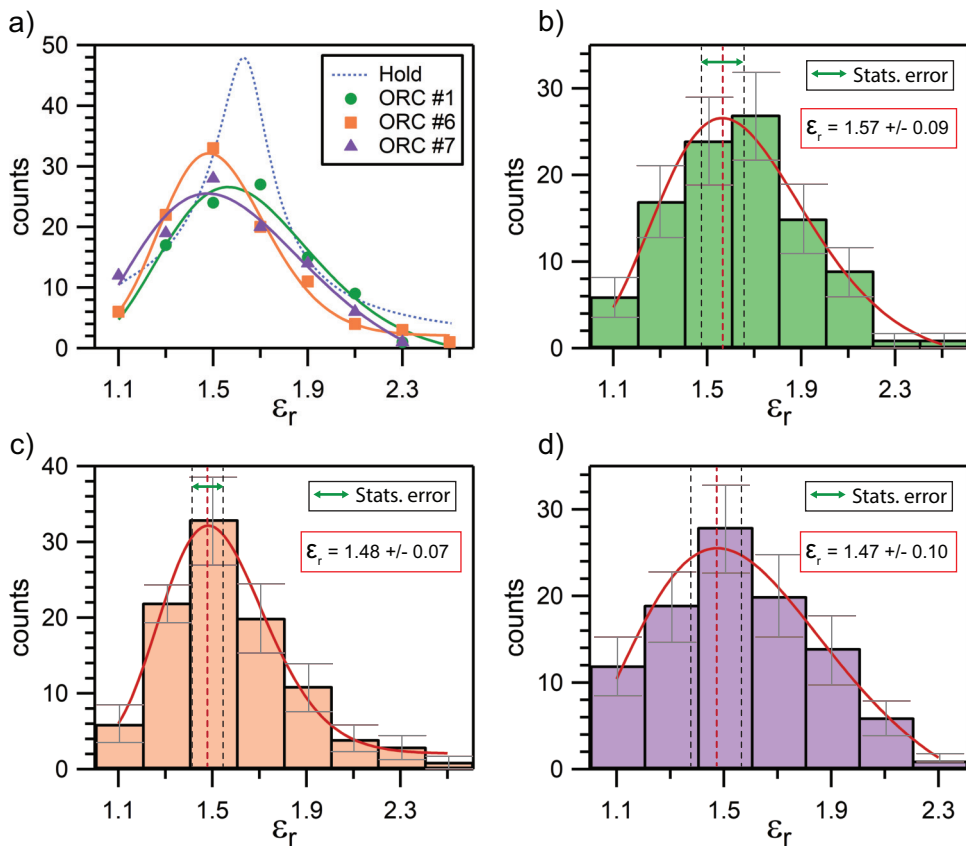
Figure 2.10: Evolution of the Statistical Distributions of \epsilon_r upon Oxidation-Reduction Cycling. (a) Comparison of the statistical distributions obtained from the measurement described before, in which the potential was held at 1.35 V for 200 s (blue dotted line), with the distributions obtained after 1, 6, and 7 ORCs, in green, orange and purple, respectively. The latter three distributions are also shown in (b), (c), and (d), respectively, where we also provide a curve fit to highlight the peak maximum, error bars based on the statistical error at each bin, and a green arrow representing the shift of the peak maximum due to the statistical error.
