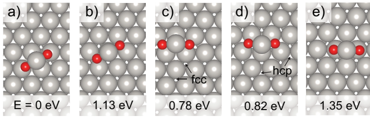
Figure 2.5: Potential Energy Landscape of a PtO_2 -adatom ( PE_{irr} -adatom) on Pt(111): (a) bridge1, (b) atop, (c) fcc, (d) hcp, (e) bridge2. The lowest energy state, the energy of a PtO_2 -adatom at bridge1, is used as reference. The diffusion barrier of a PtO_2 -adatom must be at least 0.78 eV.
