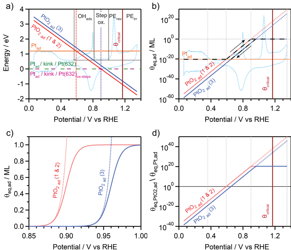
Figure 2.3: Formation Energies and Concentrations of Adatoms. (a) The formation energies of a Pt-adatom and a PtO 2 -adatom on Pt(111), and a PtO 2 -adatom on a Pt(111) with 4/25 ML O ads , are shown in orange, red, and blue, respectively. They are referenced with respect to the binding energy of an additional Pt atom attached to a kink site on Pt(632), which can be unoxidized (green dashed line) or oxidized (pink dashed line). The numbers in brackets indicate the reactions considered, as explained in the main text. The vertical dotted red and purple lines indicate the Pt-adatom oxidation potential and the potential at which E_{PtO_2,ad} (1&2) becomes zero, respectively. The first ORC is shown in dotted light blue and the different regions are indicated. (b) Equilibrium Pt- and PtO 2 -adatom concentrations calculated from (a). The dotted red and blue lines result from the Boltzmann equation which match, respectively, the solid red and blue lines (considering the entropy term without approximation) at potentials < 0.85 V. The dashed black line and the arrows indicate the path followed upon one ORC, while the vertical lines indicate the potentials used in Table 2.1. (c) Zoomed-in graph of the region between 0.85 V and 1.00 V in (b). (d) Concentration ratios between PtO 2 - and Pt-adatoms.
