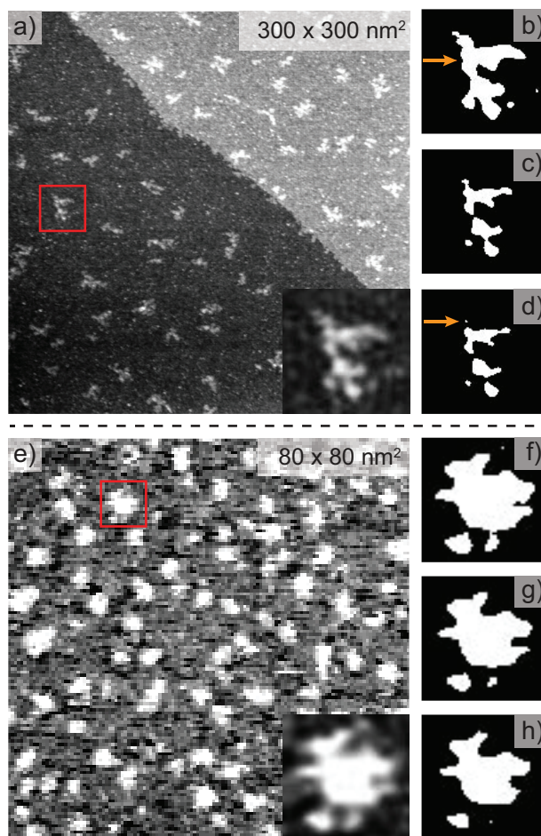
Figure 2.6: Dendritic Islands on Pt(111). (a) Vacuum-STM image of dendritic islands formed after a potential step from 1.0 to 1.3 V, holding 1.3 V for 10 s, and stepping back to 1.0 V before finally sweeping to 0.05 V at 50 mV/s. The image is reproduced with permission from T. Maagaard [40]. (b), (c) and (d) are the upper, the best, and the lower estimate, respectively, of the area of the island marked with a red square in (a). (e) Dendritic islands observed with our EC-STM after holding the potential at 1.35 V for 200 s, and then reducing to 0.3 V with 25 mV/s. This image was recorded by L. Jacobse, with U_s = 300 mV, U_t = 310 mV, and I_t \approx 300 pA. (f), (g) and (h) are the respective upper, best, and lower estimate of the area of the island marked in red in (e).
