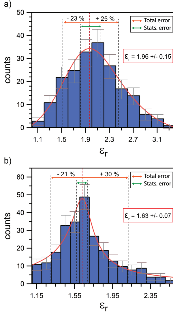
Figure 2.8: Statistical Distribution of \epsilon_r for the Best Estimate of the Island Shapes: (a) measured in vacuum (analyzed from Fig. 2.6a and Fig. A.3 in the Appendix A) and (b) in electrolyte (analyzed from Fig. 2.6e and Fig. A.5 in Appendix A). The peak maximum of the statistical distributions, obtained by fitting with a Pearson IV function, are indicated with red dashed lines. The lower and upper bound are indicated with the orange arrow, while the statistical error, derived via the possible shift within the statistical error bars, is indicated with the green arrow.
