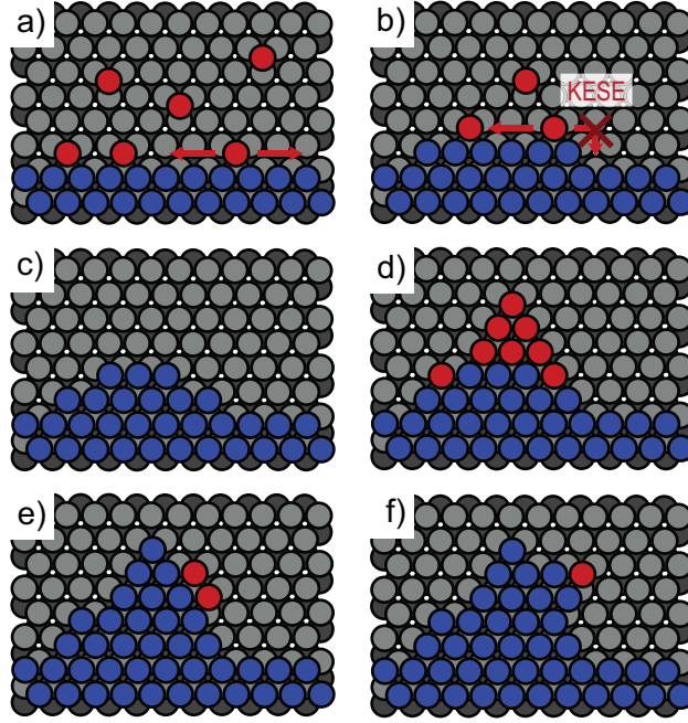
Figure 2.7: Scheme of the Growth Instability (KESE) resulting in Dendritic Islands: (a) Step-adatom (1D) diffusion resulting in the nucleation of 1D-island rows. (b) The KESE makes it more difficult for the atom to diffuse around the kink, leading to the nucleation and growth of a second row (c). (d) The arrival of more adatoms leads eventually to the growth of triangles (branches) perpendicular to the step. (e) Nucleation of a new row on the side of a triangle, which finally results in the bifurcation of the branch (f).
