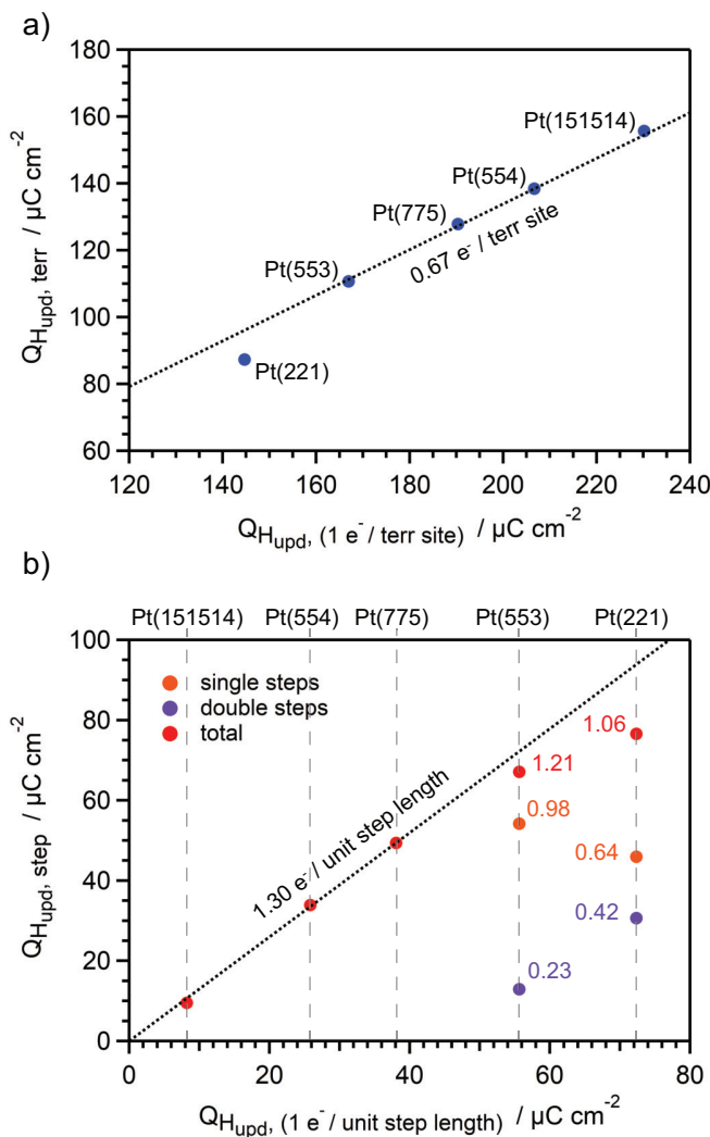
Figure 4.3: Correlation between the Measured and the Theoretical H_{upd} Charge Densities on Terraces and Steps. (a) H_{upd} charge densities on terraces, as given by a Frumkin isotherm fit, versus the theoretical charge densities assuming one electron is transferred per terrace site. (b) H_{upd} charge densities from single steps (orange), step bunches (purple), and the sum of them (red), versus the theoretical charge densities assuming one electron is interchanged per unit step length. We also provide the experimental values in units of electrons per unit step length.
