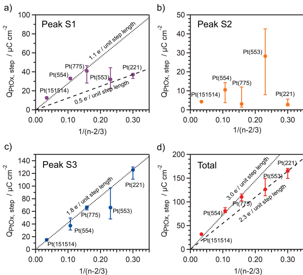
Figure 4.6: Step Oxidation Charges versus Step Density: (a-c) step oxidation charges resulting from the integral of each of the step oxidation peaks fitted in Fig. 4.5, as indicated. (d) shows the total step oxidation charge, which is the sum of the three peaks. We also show the resulting numbers of electrons transferred per unit step length for each peak, which we calculated from the trend lines. In (a) and (d), two different regimes are clearly visible: one involving Pt(15 15 14), Pt(554), and Pt(775), and the other involving Pt(553) and Pt(221). The reason for the two regimes is step bunching. The error bars show the variation of the corresponding charges when taking sub-optimal fits (i.e. with a higher Chi Squared) obtained when varying slightly the upper and lower fitting boundaries.
