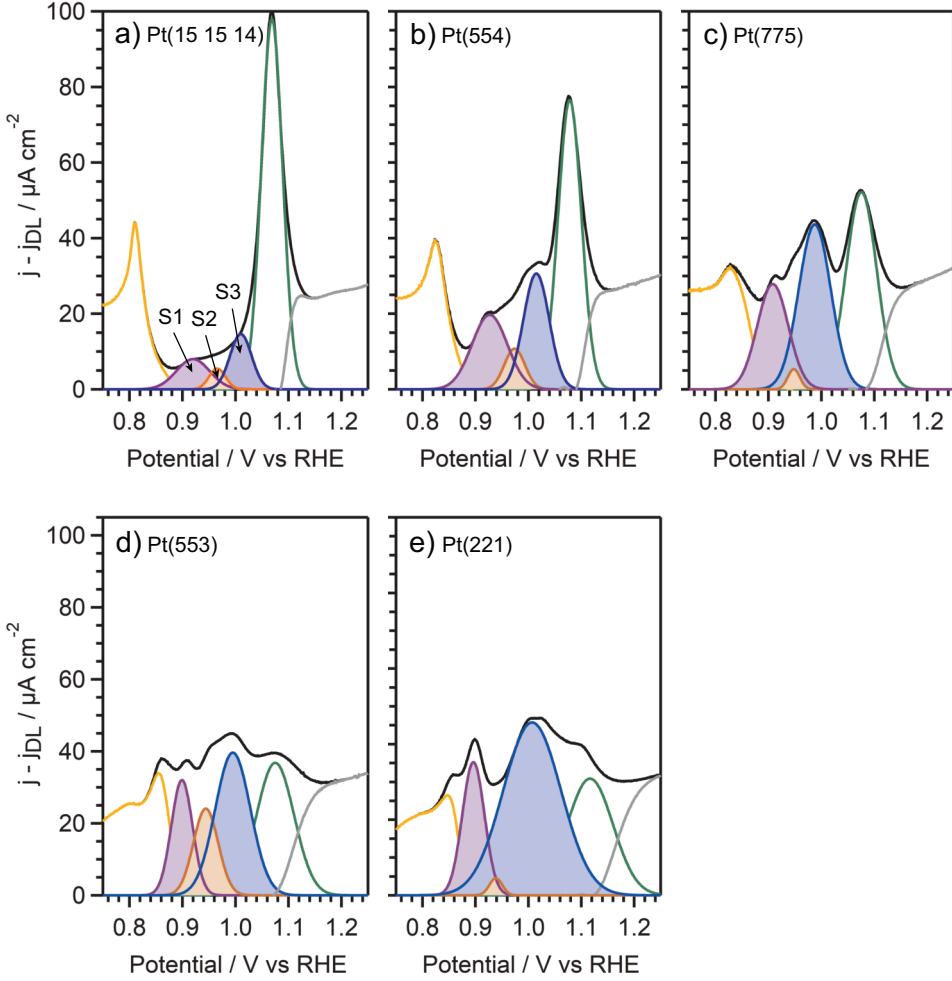
Figure 4.5: Deconvolution of the Platinum Oxidation Region: the three step oxidation peaks (S1, S2, and S3, respectively) as well as the PE_{rev} -peak (green curve) are obtained with Gaussian fit functions. The OH_{ads} butterfly peak in yellow and the PE_{irr} -peak in gray are derived by subtraction of the Gaussian peaks from the measured total current density, shown in black.
