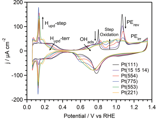
Figure 4.1: Cyclic Voltammograms of Pt(111) and its Vicinal Surfaces with (111) Steps. CVs recorded in 0.1 M HClO 4 from 0.06 to 1.35 V using a scan rate of 50 mV s -1 . The most relevant regions are indicated with the corresponding text and the general trend when increasing the step density with arrows.
