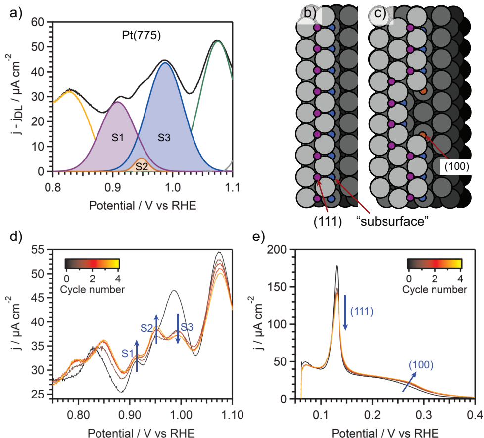
Figure 4.7: Atomic Site Identification of the Step Oxidation Peaks. (a) Step oxidation peaks of Pt(775). (b) Corresponding oxygen adsorption sites at the (111) (fcc) position at the upper step edge and the threefold subsurface position at the lower step edge. (c) Oxygen adsorption sites at a faceted (111) step with (100) microfacets, which present a partially subsurface site with twofold coordination at the lower step edge. (d) Step oxidation peaks upon oxidation-reduction cycling: S1 and S2 increase in intensity due to the increase in the number of (111) and (100) sites, respectively, while S3 decreases due to the annihilation of subsurface sites at the lower (111)-step edge. (e) H_{upd} region upon oxidation-reduction cycling: the (100) step peak increases at the expense of the (111) step peak during the first 5 cycles.
