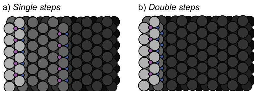
Figure 4.8: Oxidation of Single and Double Steps. (a) \text{PtO}_2 structure on single steps of Pt(553). The purple and blue oxygen circles represent oxygen atoms adsorbed at (111) (fcc) sites on the upper step edge and partially subsurface sites on the lower step edge, respectively. (b) \text{PtO}_2 structure on double steps of Pt(553). One row of \text{O}_{\text{ad}} at the upper step edge is missing in comparison to the single step structure.
