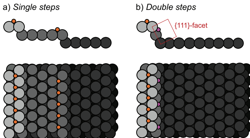
Figure 4.4: Hydrogen Adsorption at Single and Bunched Steps. (a) Hydrogen adsorption on a (111) single step and (b) on a double (bunched) step. For the single step site, we have drawn the hydrogen adsorbed at fcc sites at the upper step edge (in orange), although this is not clear from DFT calculations due to the similar binding energies between the fcc, hcp, and bridge sites [52, 71]. Moreover, from our quantitative analysis we can not discard that the step sites related to the H_{\text{upd}} -step peak are located, instead, at the lower step edge, as this would result in the same H_{\text{upd}} -step charge. On step bunches hydrogen adsorbs, in addition, at the {111}-facet formed (in purple), although we know from the charge density analysis that some of these sites must remain unoccupied. A triple step (not shown here) presents one row of fcc adsorption sites at the upper step edge and two rows at the {111}-facet.
