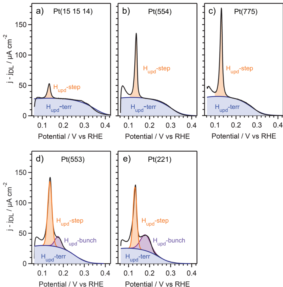
Figure 4.2: H_{upd} Deconvolution into Step and Terrace Contributions. The black line represents the total, measured H_{upd} current density after correction for the current density contribution from the double layer charging, while the blue line is the fit of the the H_{upd} -terrace current density with a Frumkin isotherm. The corresponding terrace, single step, and step bunch contributions to the H_{upd} charge density are colored in blue, orange, and purple, respectively.
