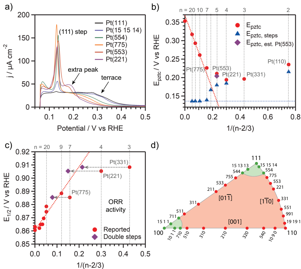
Figure 3.5: Effects of Step Bunching on Platinum Electrochemistry. (a) Hydrogen desorption fingerprint of Pt(111) and (111)-vicinal surfaces with (111) steps recorded in 0.1 M \text{HClO}_4 at a scan rate of 50 \text{ mV s}^{-1} . The peaks related to terraces, single (111) steps, and step bunches, the latter only present on Pt(553) and Pt(221), are indicated. (b) E_{pztc} (in red) and (local) E_{pztc} at step sites (in blue) versus the step density, extracted from Refs. [7, 41, 43]. The stepped surfaces that undergo step bunching ( n \leq 7 ) do not follow the linear decrease of E_{pztc} with step density shown in red. The purple diamond represents our estimation of E_{pztc} for Pt(553), calculated from a fit of the dipole moment for double steps. (c) ORR activity, represented by the half-wave potential, versus step density, extracted from Refs. [8, 9]. The ORR activity increases linearly with the step density for n \geq 9 . The purple diamonds represent the adjusted values for Pt(775), Pt(221), and Pt(331) assuming that they only have double steps. (d) Stereographic triangle showing the stable surfaces in green and the unstable ones in red. Pt(110) forms a (1x2) missing-row reconstruction [24, 49], while Pt(100) is unreconstructed in electrolyte [50].
